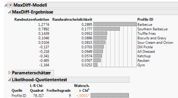
MaxDiff
