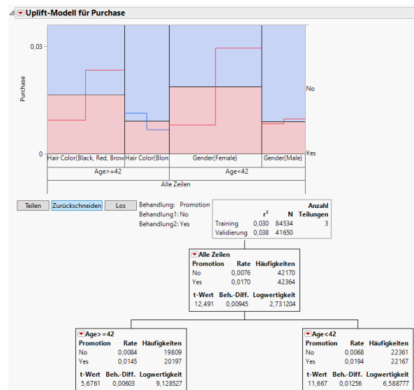
Uplift-Modell
