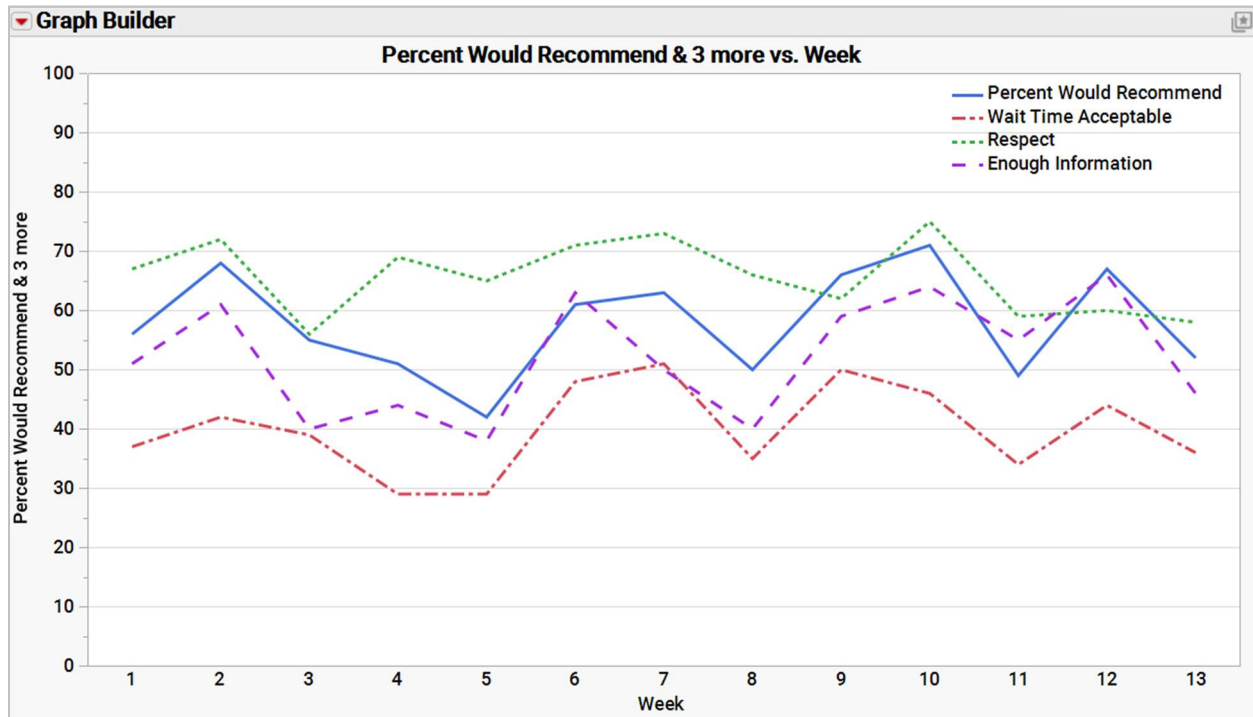
Exhibit 6 Run Chart – All Four Measures
