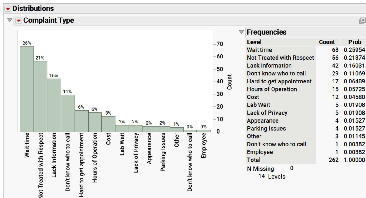
Exhibit 3 Pareto Chart of Complaint Data
