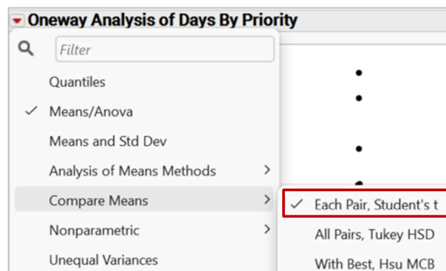
Exhibit 4 Multiple Comparison Procedures
