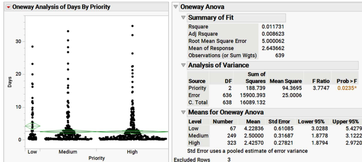
Exhibit 4 Oneway ANOVA for Days by Priority
