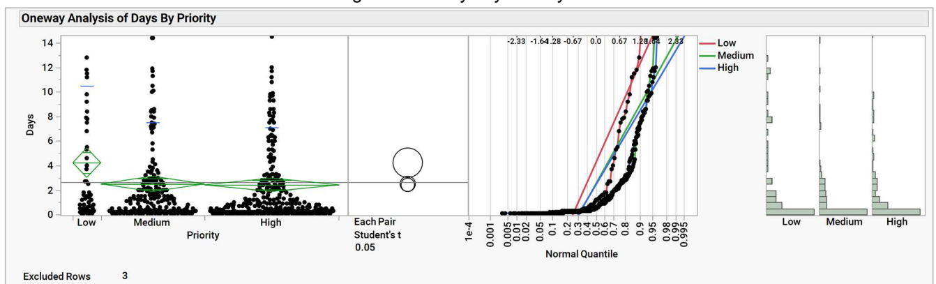
Exhibit 7 Normal Quantile Plots and Histograms for Days by Priority
