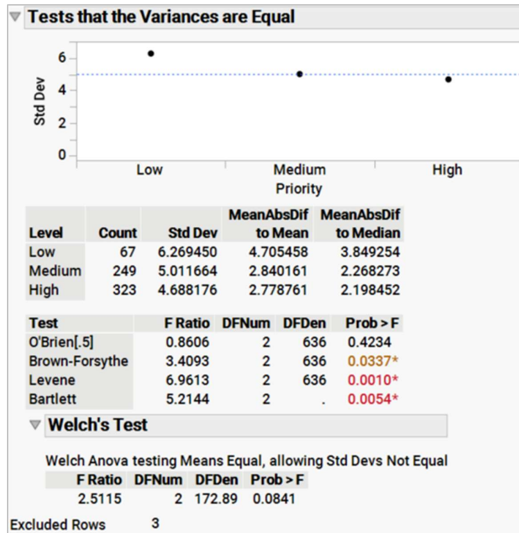
Exhibit 6 Unequal Variances Test for Days by Priority
