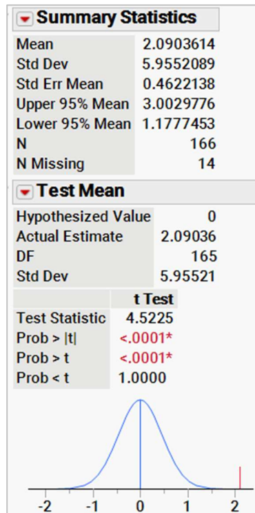
Exhibit 6 One-Sample t-Test for the Combined Score
