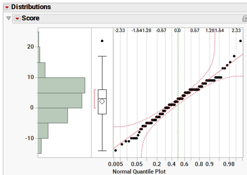
Exhibit 5 Distribution of the Combined Score Data
