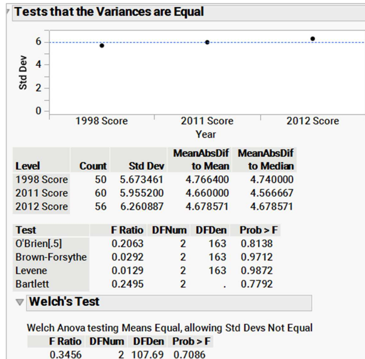
Exhibit 3 Testing for Equal Spread
