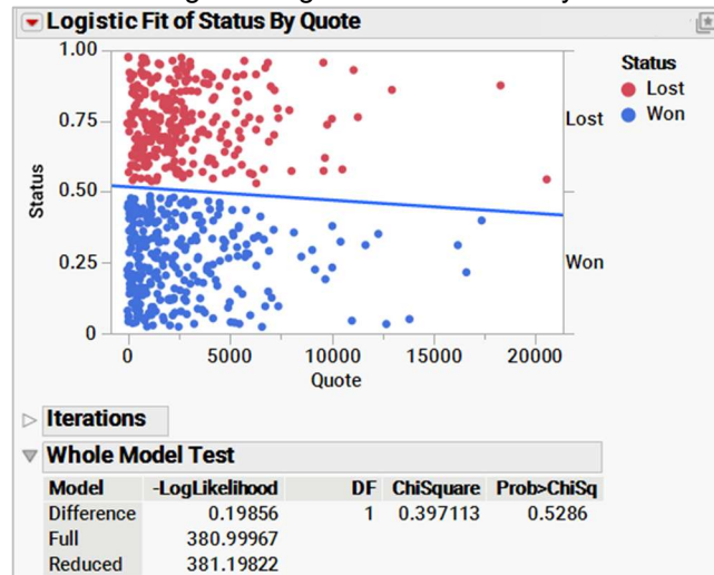
Exhibit 4 Logistic Regression of Status by Quote
