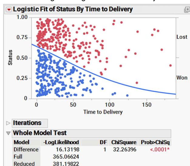
Exhibit 5 Logistic Regression of Status by Time to Delivery
