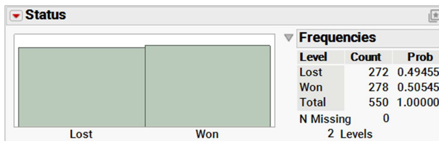
Exhibit 1 Bar Chart of Status
