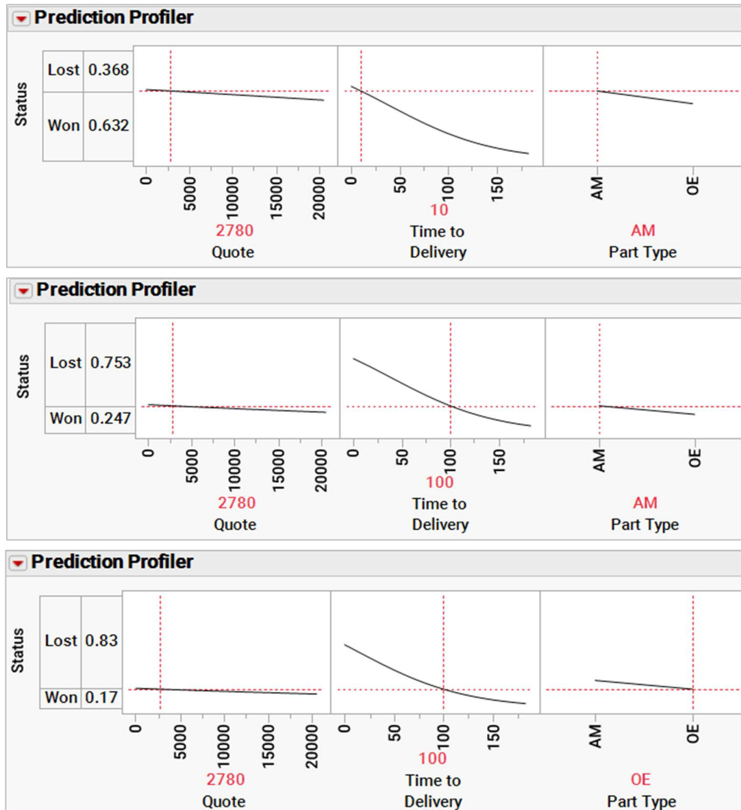
Exhibit 7 Prediction Profiler for Status with all Predictors
