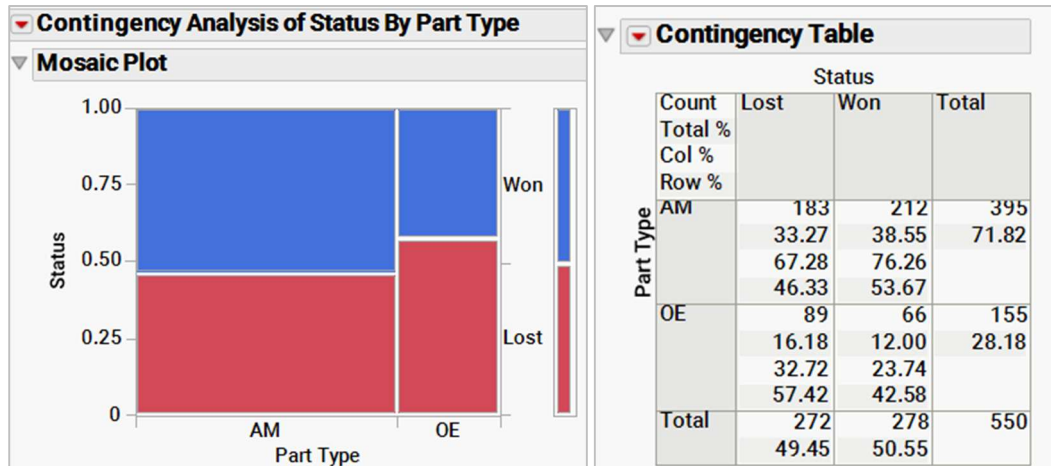
Exhibit 2 Mosaic Plot and Cross-tabulation of Status and Part Type
