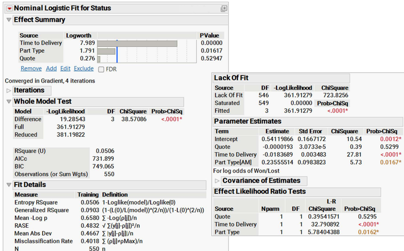
Exhibit 6 Parameter Estimates for Multiple Logistic Model
