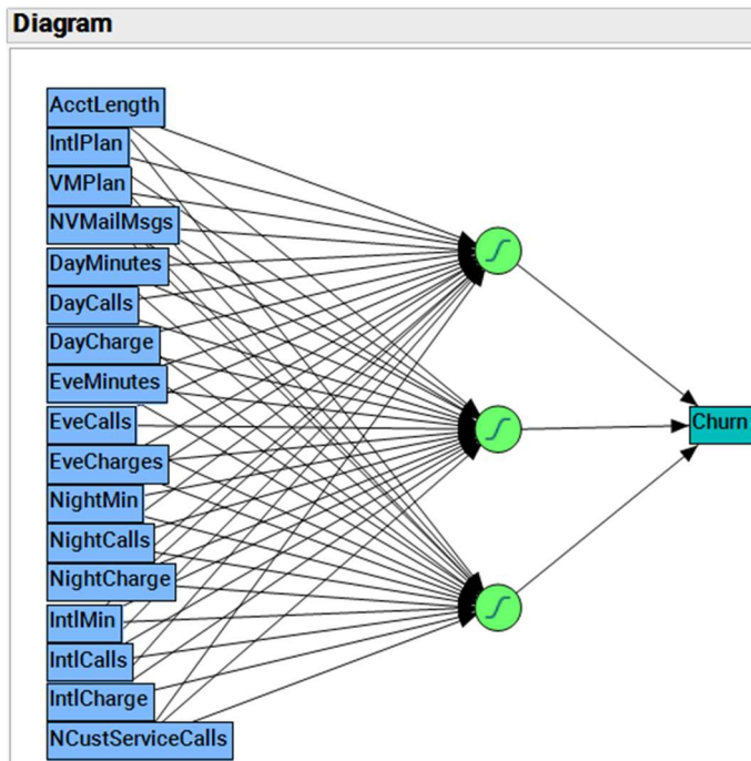
Exhibit 7 Diagram for the Fitted Neural Network Model
