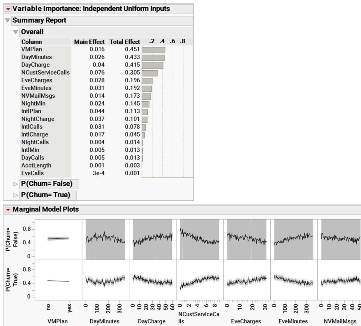
Exhibit 15 Variable Importance and Marginal Model Plot
