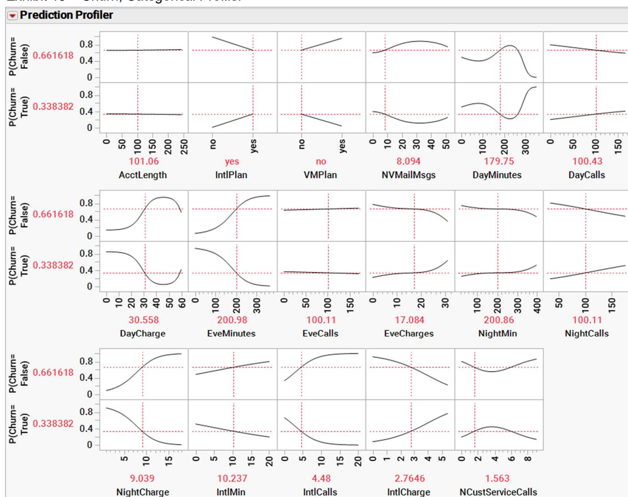
Exhibit 13 Churn, Categorical Profiler
