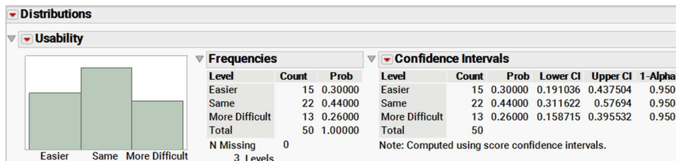
Exhibit 2 Distribution with confidence intervals
