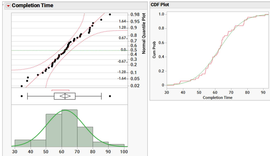
Exhibit 4 Fitting a Distribution to the Data
