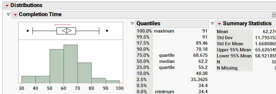
Exhibit 3 Distribution of Completion Time
