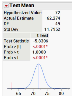
Exhibit 6 Hypothesis Test for the Population Mean
