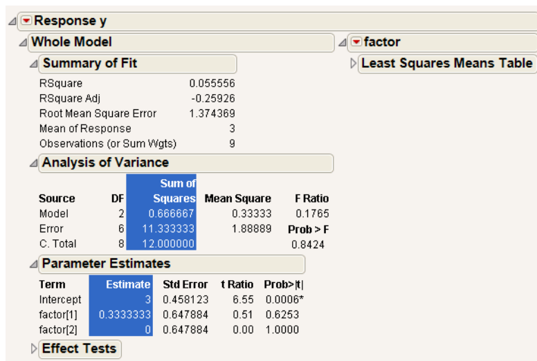
Figure 7.1 ANOVA Report Within Fit Model
