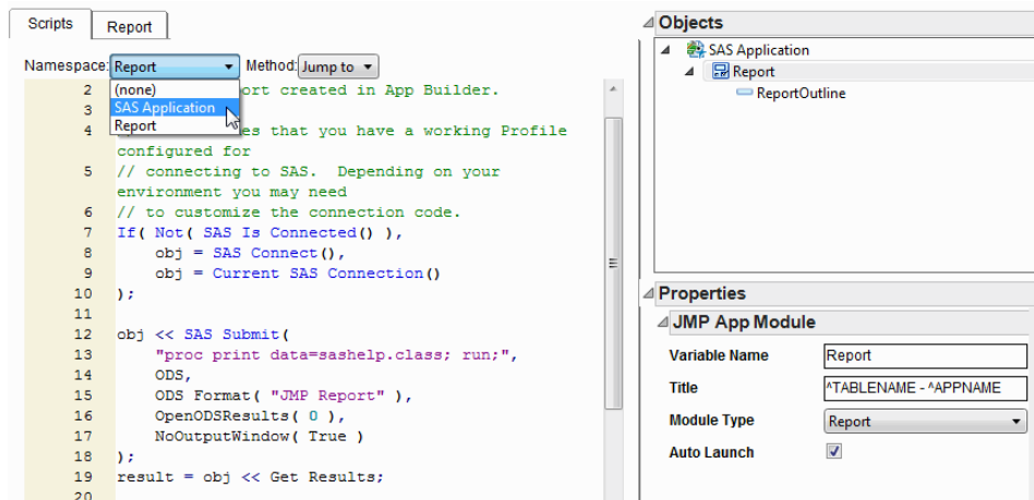
Figure 15.10 Application and Module Namespaces
