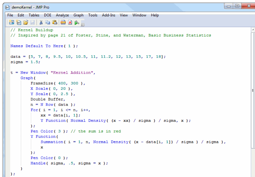
Figure 4.2 The Script Editor
