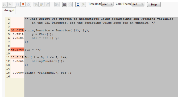
Figure 4.17 Profiled Script Window
