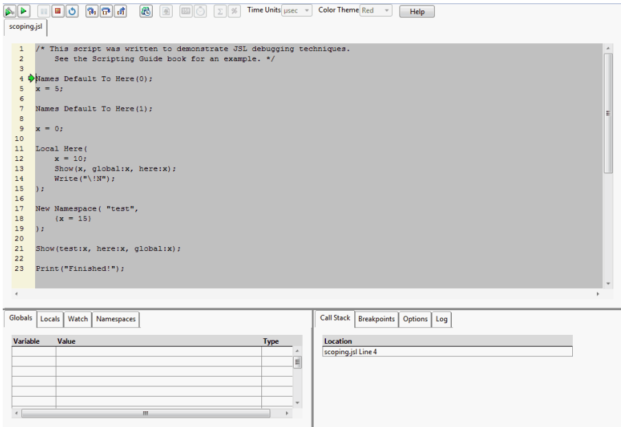
Figure 4.11 The Debugger Window
