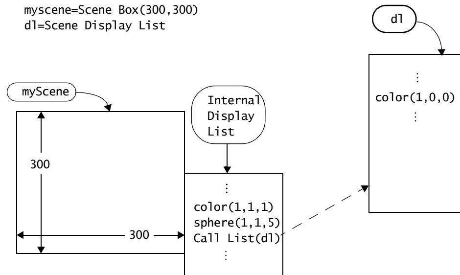
Figure 13.2 Constructing Scenes
