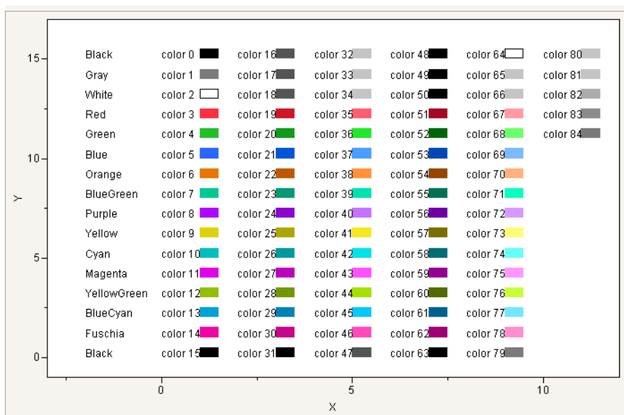
Figure 9.8 JMP Colors
