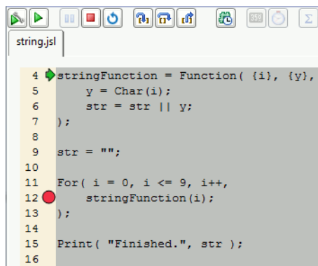
Figure 4.12 Set the Breakpoint
