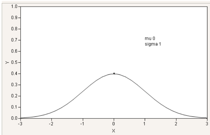
Figure 12.22 Normal Density Example for Handle
