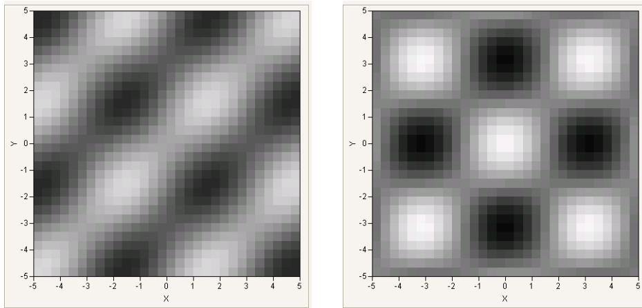
Figure 12.8 Gradient Function
