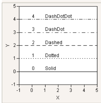
Figure 12.20 Line Styles
