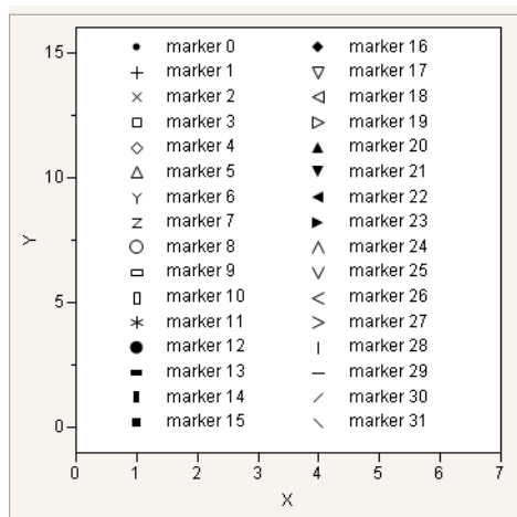
Figure 9.7 JMP Markers
