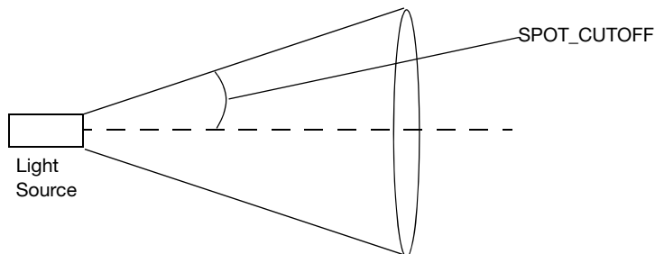
Figure 13.16 Spotlight
