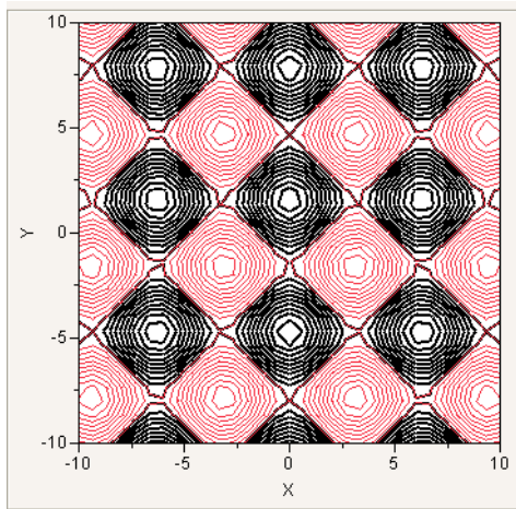
Figure 12.6 Egg Carton Function
