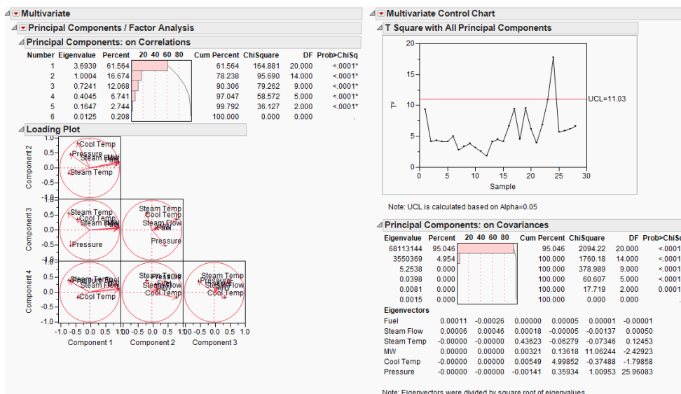
Figure 15.12 Multivariate Application
