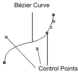
Figure 13.19 Bézier Curve
