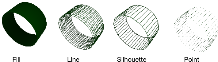
Figure 13.13 Draw Styles
