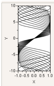
Figure 12.5 Overlapping Sine Waves Along the X-Axis
