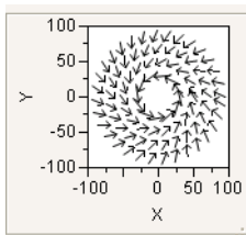
Figure 12.10 Drawing Arrows
