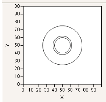
Figure 12.14 Drawing Circles
