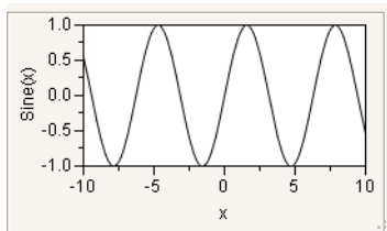
Figure 12.3 Sine Wave
