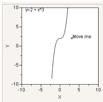
Figure 12.23 Intercepts and Powers Example for Handle
