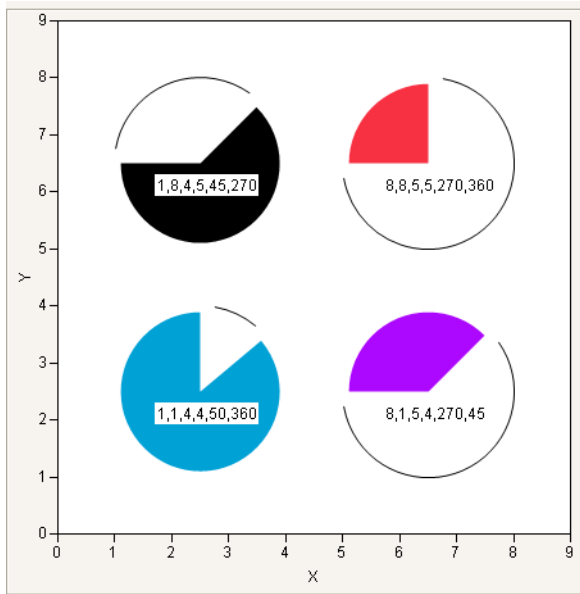
Figure 12.13 Drawing Pies and Arcs
