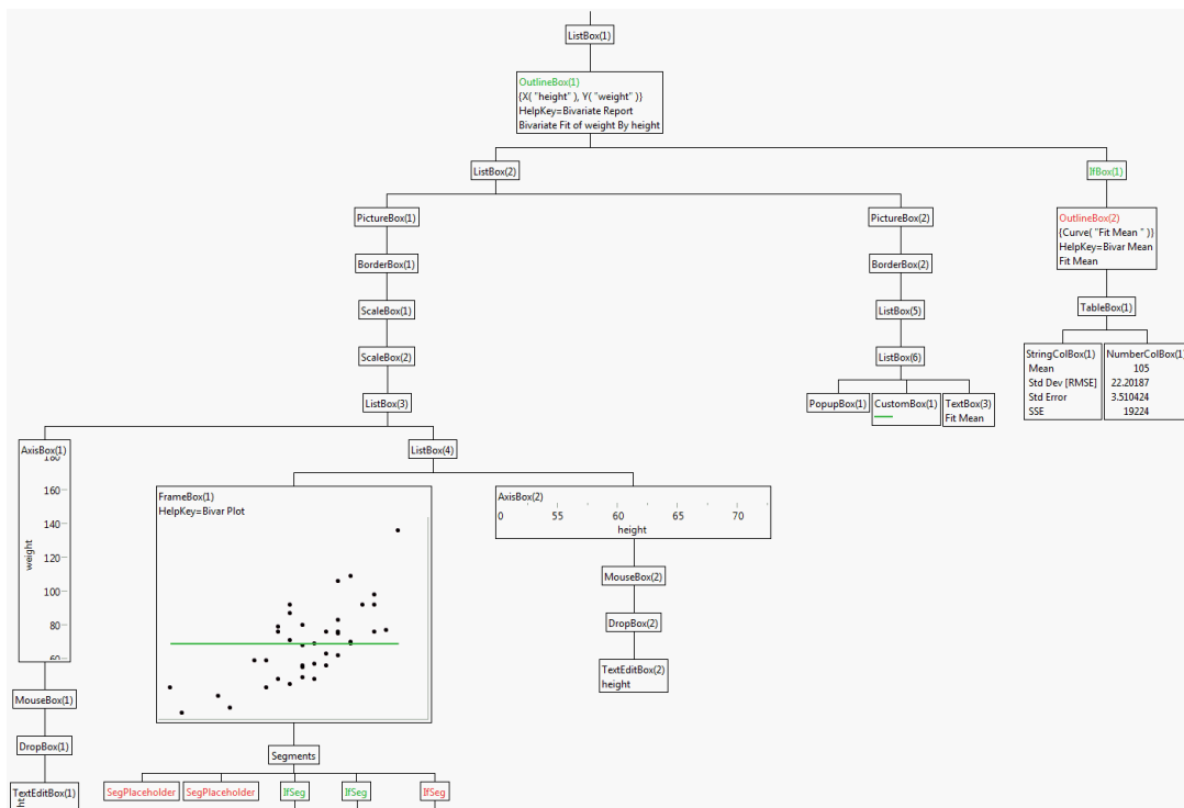
Figure 11.3 Classic Tree Structure
