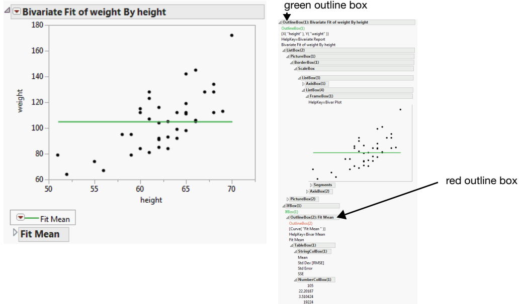
Figure 11.2 Show Tree Structure
