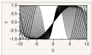
Figure 12.4 Overlapping Sine Waves
