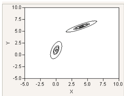
Figure 12.7 Normal Contour Function
