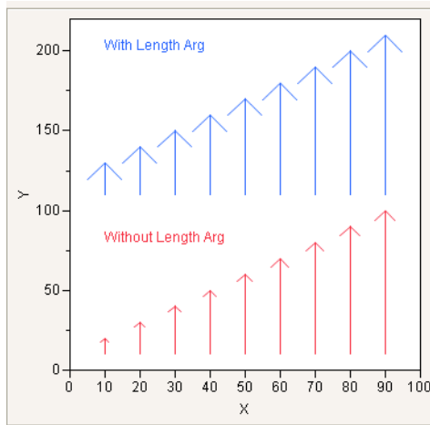
Figure 12.11 Arrowhead Sizes
