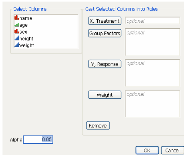
Figure 11.25 Column Dialog
