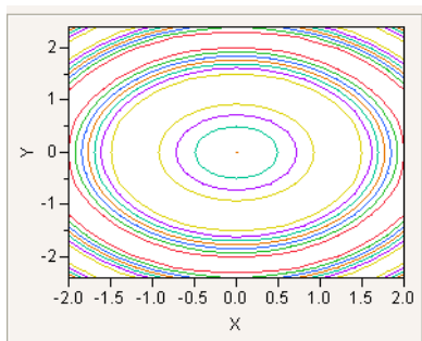
Figure 12.17 Drawing Contour Lines
