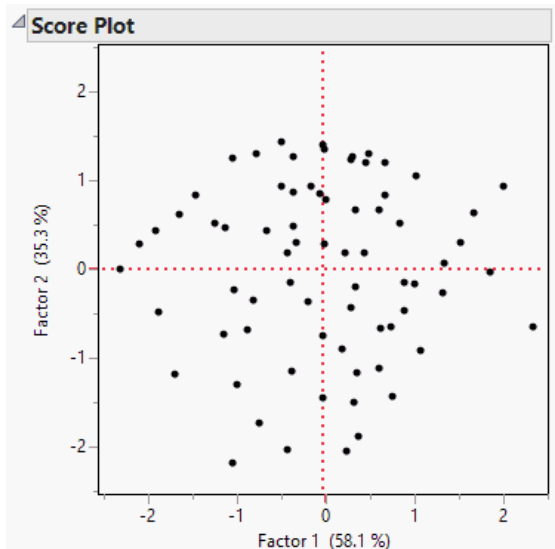
Figure 6.19 Score Plot
