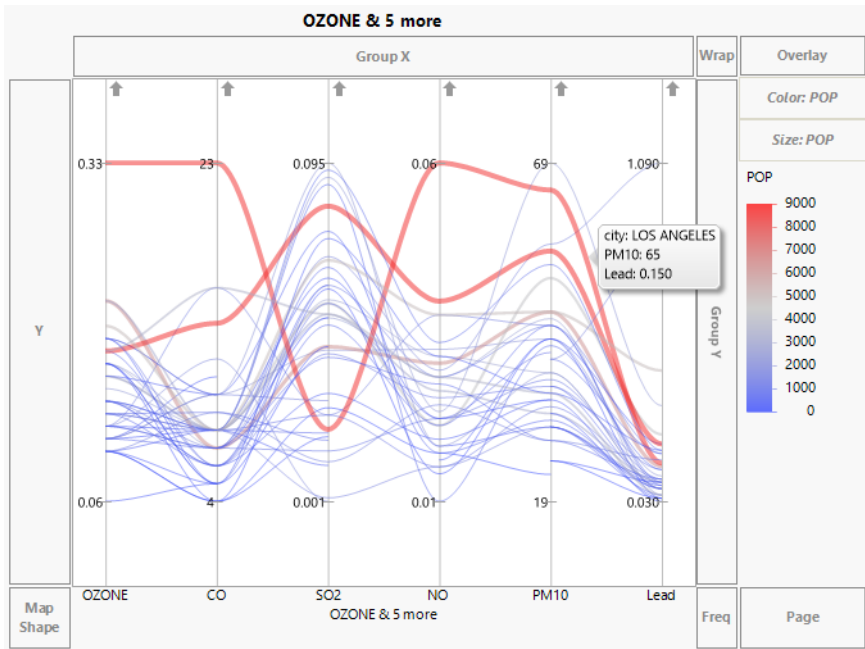
Figure 3.42 Parallel Plot for Pollution Data in Cities.jmp
