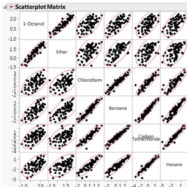
Figure 3.4 Scatterplot Matrix
