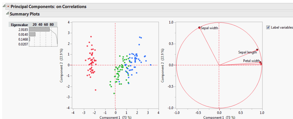
Figure 4.1 Example of Principal Components
