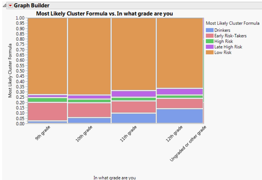
Figure 10.4 Mosaic Plot of Cluster Membership versus Grade Level
