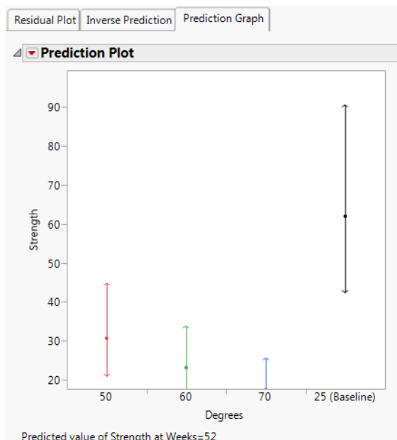
Figure 7.25 Prediction Plot at Weeks = 52
