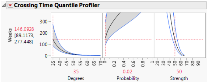
Figure 8.9 Crossing Time Quantile Profiler
