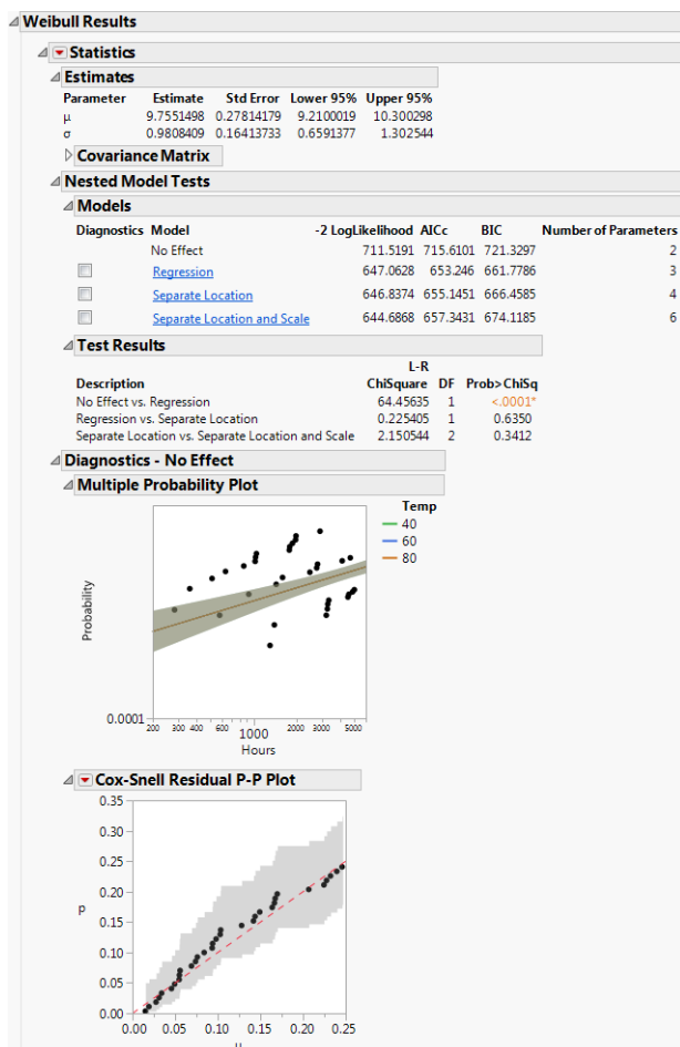
Figure 4.18 No Effect Model with the Weibull Distribution for Devalt.jmp Data
