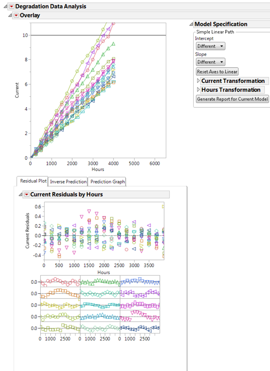
Figure 7.2 Initial Degradation Report
