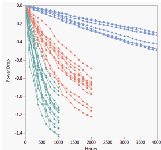
Figure 7.7 Device B Overlay Plot
