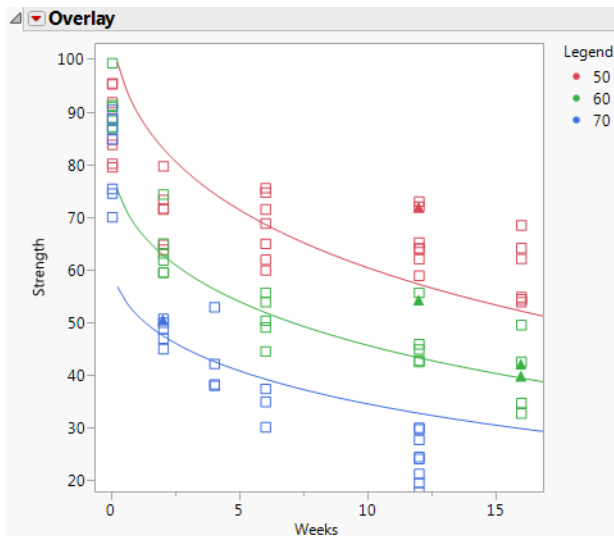
Figure 7.23 Plot of Fitted Model
