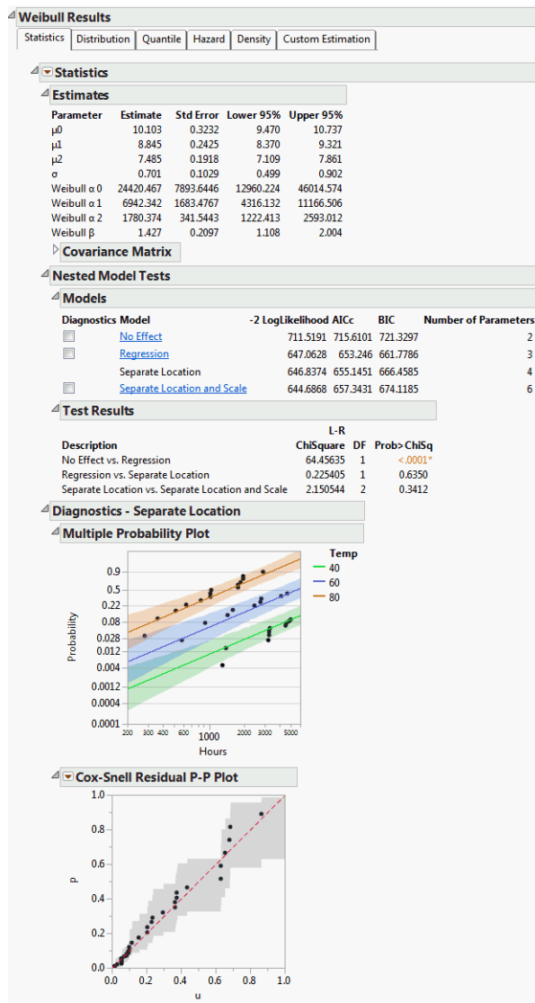
Figure 4.16 Separate Location Model with the Weibull Distribution for Devalt.jmp Data
