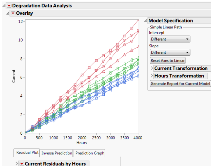
Figure 7.1 Degradation Analysis Example
