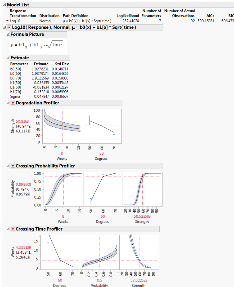
Figure 8.4 Report for Basic Model
