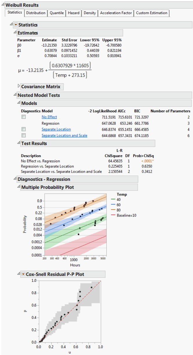
Figure 4.17 Regression Model with the Weibull Distribution for Devalt.jmp Data
