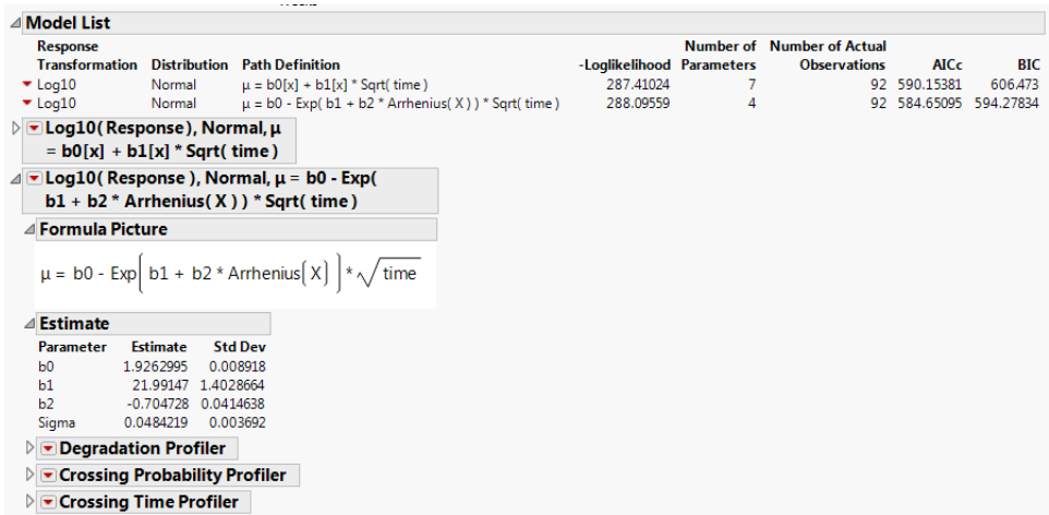
Figure 8.6 Report Including Second Model with Arrhenius Transformation
