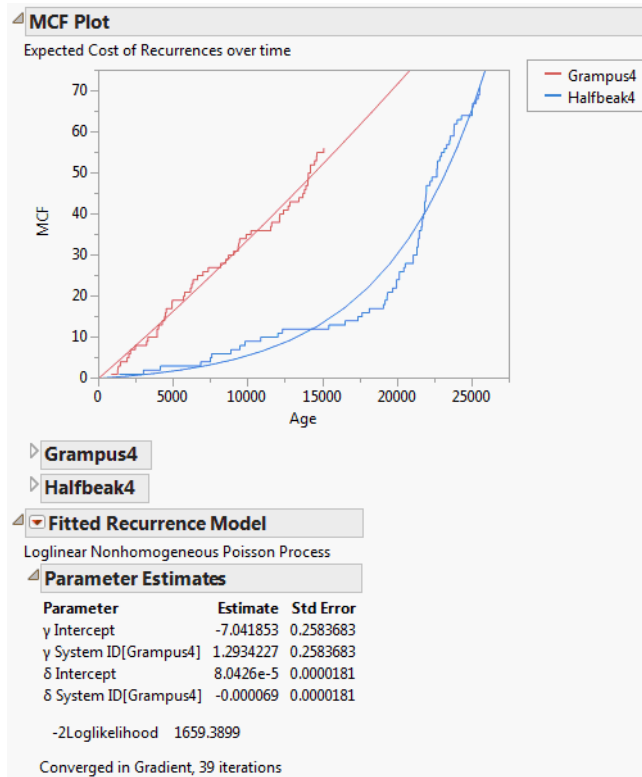
Figure 6.13 Diesel Ship Engines Fitted Model
