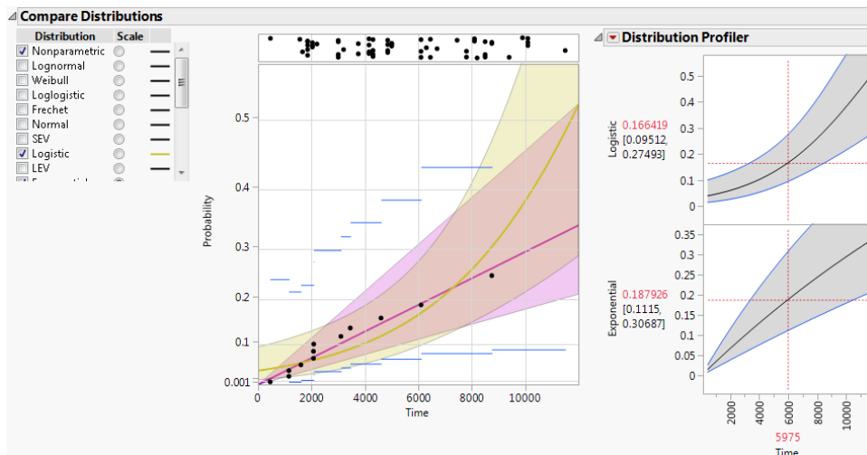
Figure 3.1 Distributional Fits and Comparisons
