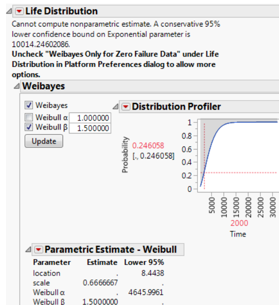
Figure 3.20 Life Distribution Report for Zero Failures
