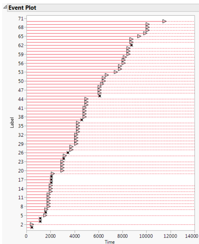
Figure 3.6 Event Plot for Right-Censored Data
