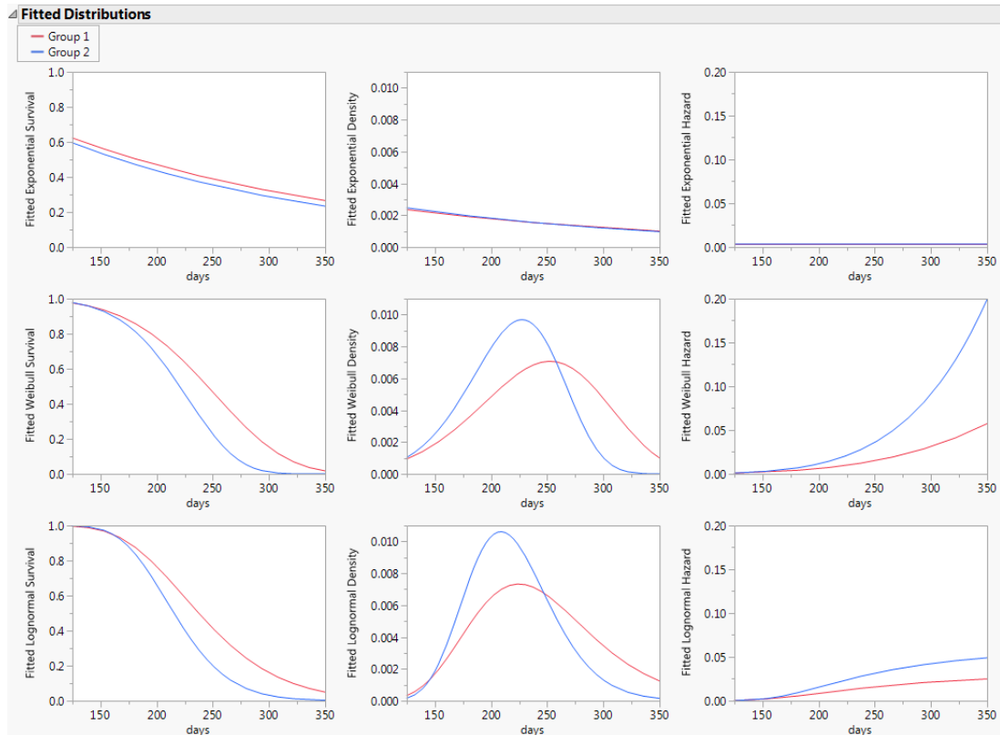
Figure 13.7 Fitted Distribution Plots for Three Distributions
