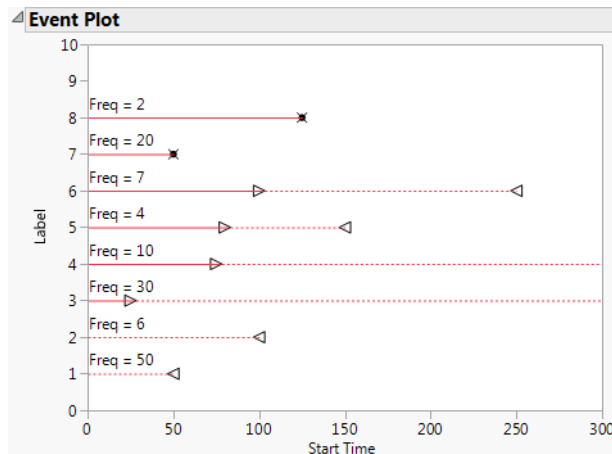
Figure 3.7 Event Plot for Mixed-Censored Data
