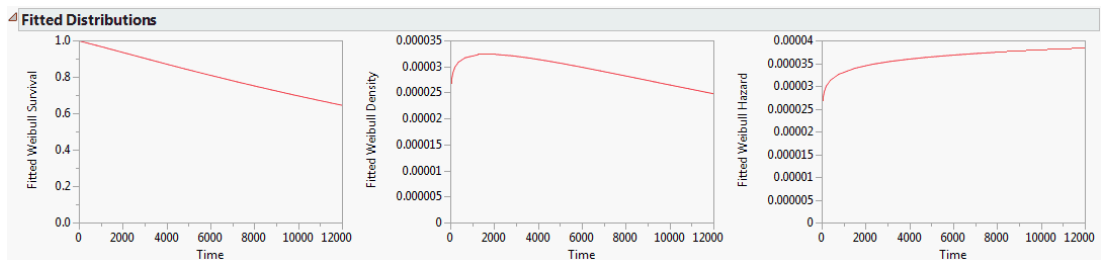
Figure 13.10 Fitted Distribution Plots
