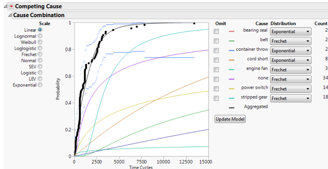
Figure 3.13 Initial Competing Cause Report
