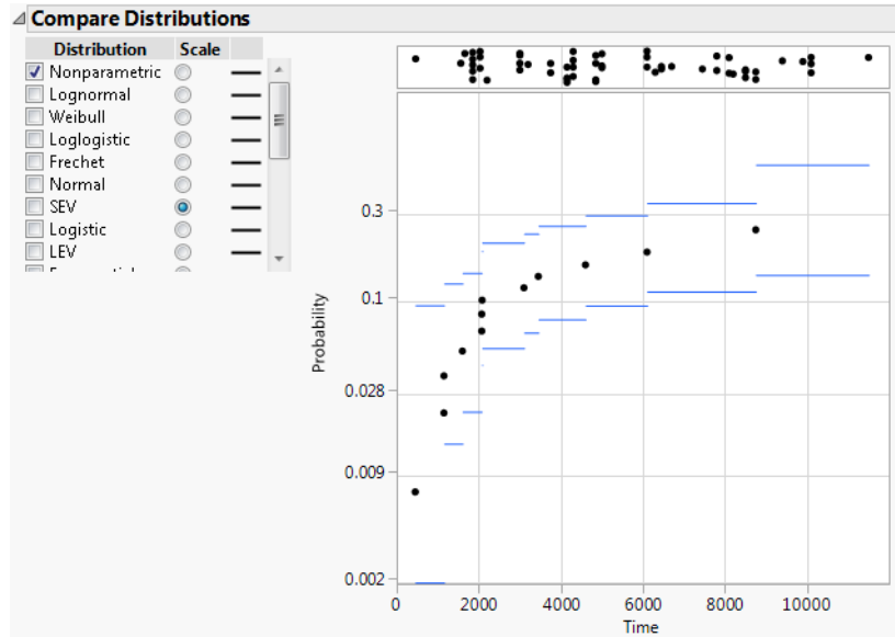
Figure 3.17 Nonparametric Estimates with a SEV Probability Scale
