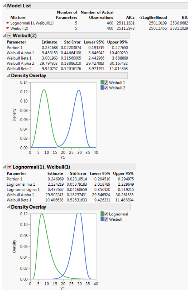
Figure 3.10 Fit Mixture for Lognormal(1), Weibull(1)
