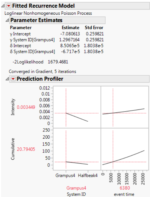
Figure 6.14 Diesel Ship Profiler
