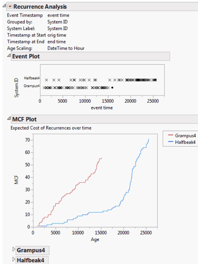
Figure 6.12 Diesel Ship Engines Report
