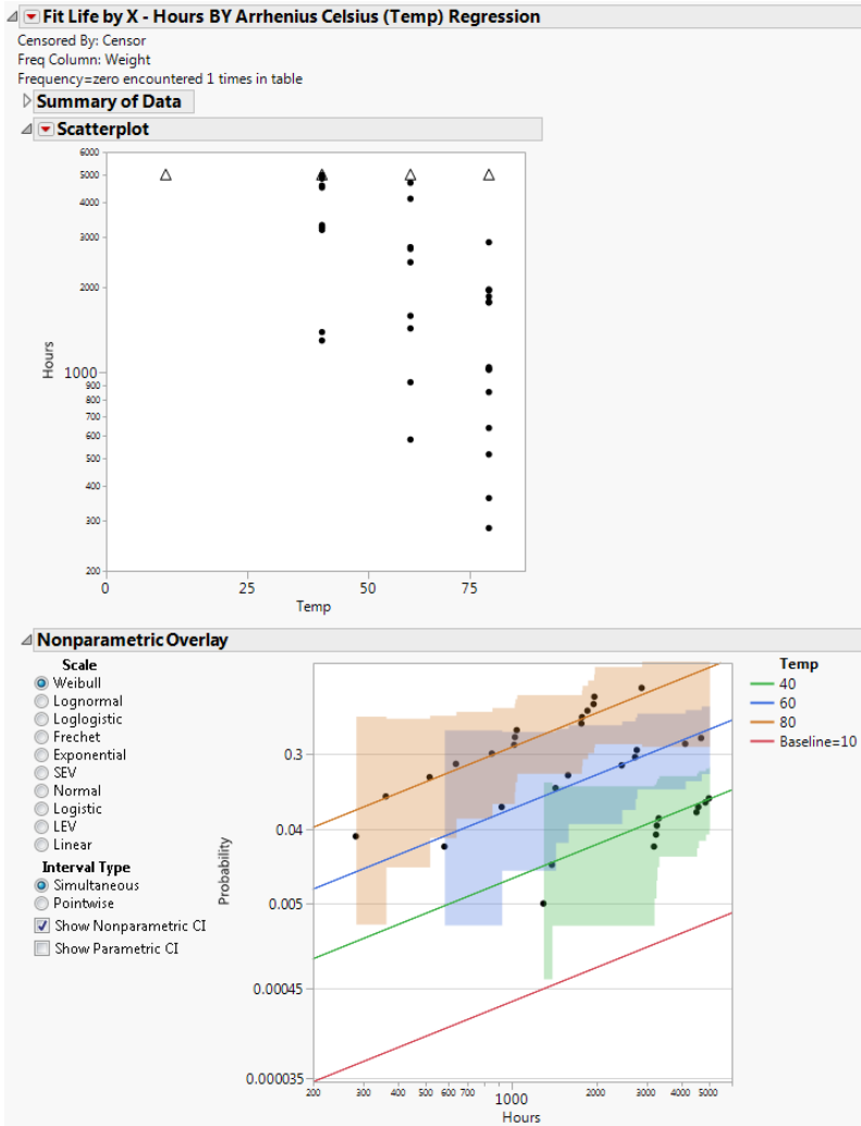
Figure 4.3 Fit Life by X Report Window for Devalt.jmp Data
