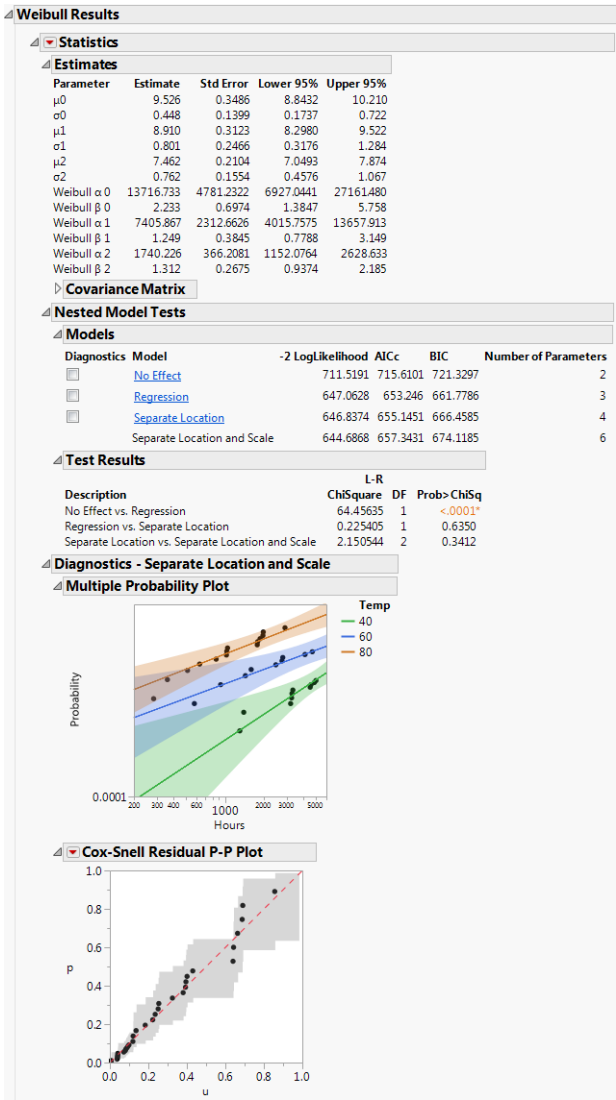
Figure 4.15 Separate Location and Scale Model with the Weibull Distribution for Devalt.jmp Data
