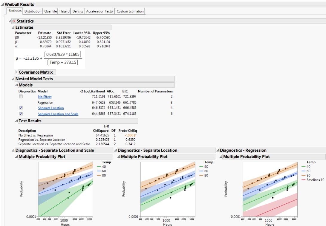
Figure 4.13 Weibull Distribution Nested Model Tests for Devalt.jmp Data
