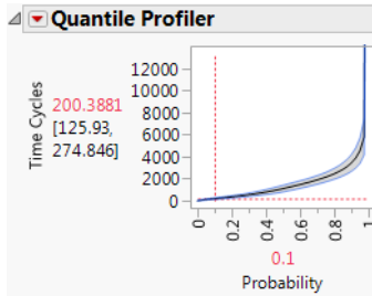
Figure 3.14 Estimated Failure Time for 10% of the Units
