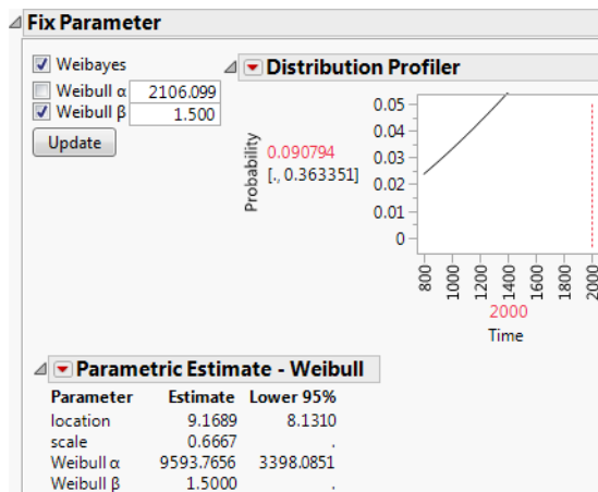
Figure 3.21 Life Distribution Report for One Failure
