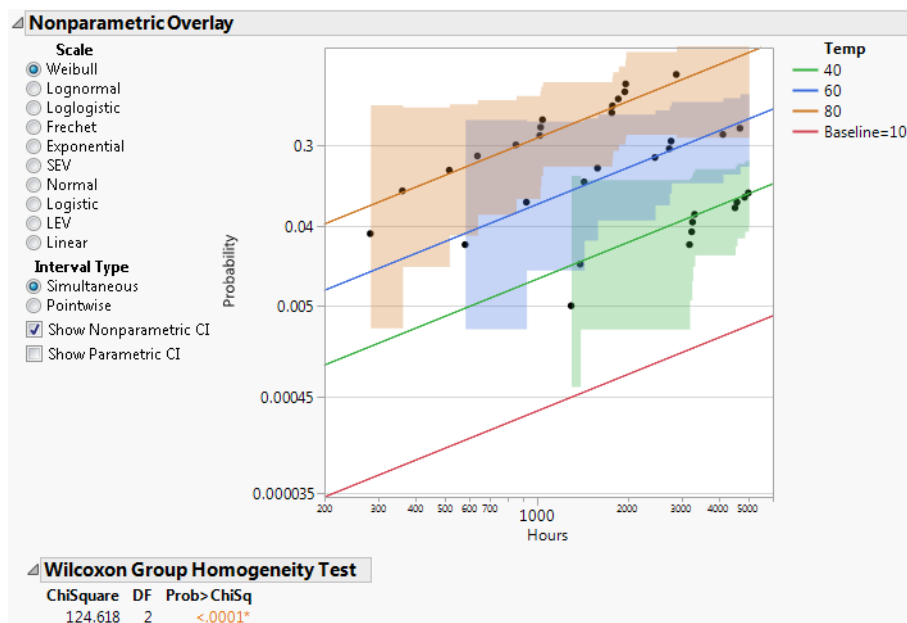
Figure 4.8 Nonparametric Overlay Plot and Wilcoxon Test for Devalt.jmp
