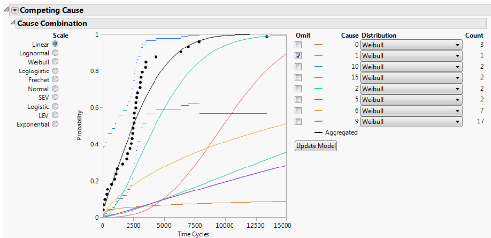
Figure 3.22 Fixed Parameter Model with Cause 1 Omitted
