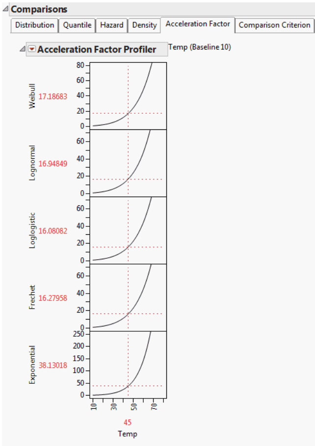
Figure 4.11 Acceleration Factor Profiler for Devalt.jmp
