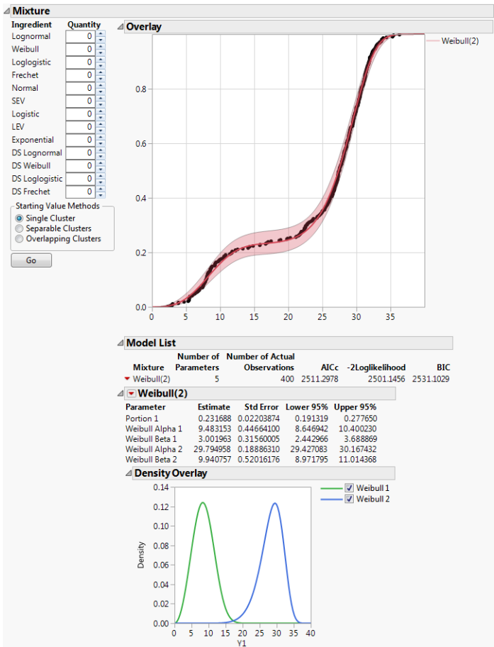
Figure 3.9 Fit Mixture for Weibull (2)
