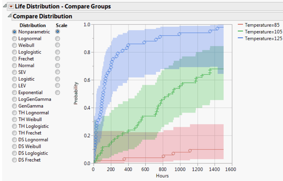
Figure 3.18 Compare Distribution for Groups
