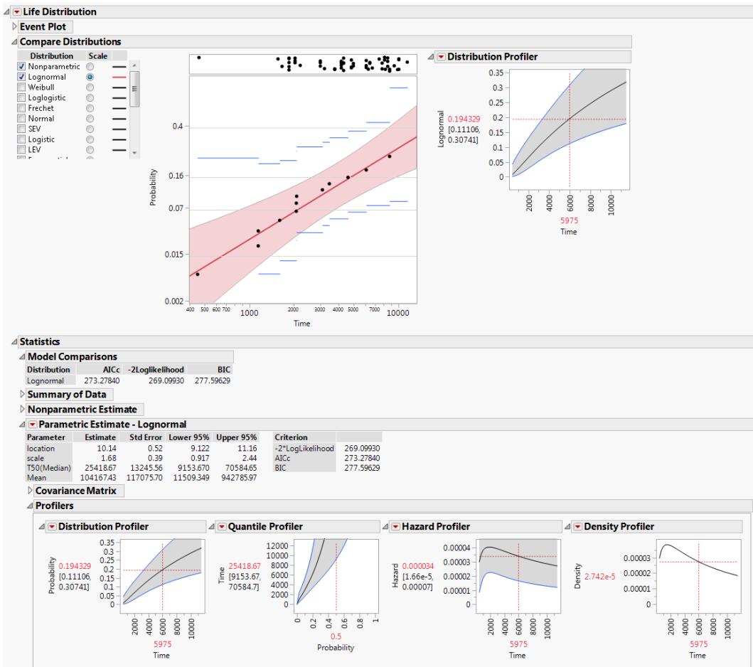
Figure 3.5 Example of the Life Distribution Report for Fan.jmp
