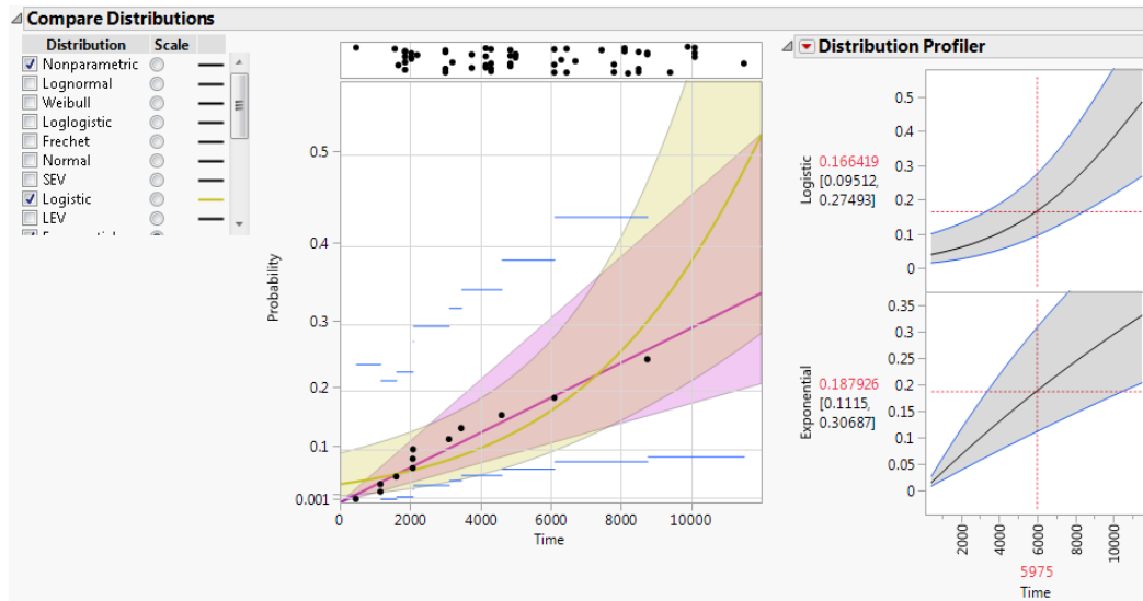
Figure 3.8 Compare Distributions Report and Distribution Profiler
