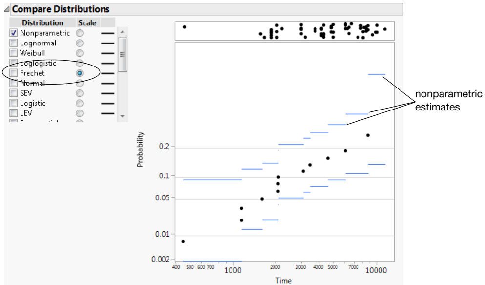
Figure 3.16 Nonparametric Estimates with a Fréchet Probability Scale
