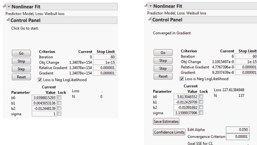
Figure 14.16 Nonlinear Model with Custom Loss Function
