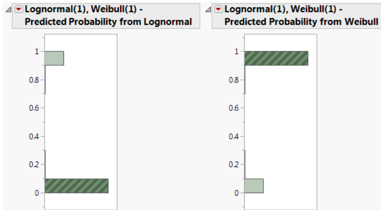
Figure 3.11 Histograms for Mixture Probabilities
