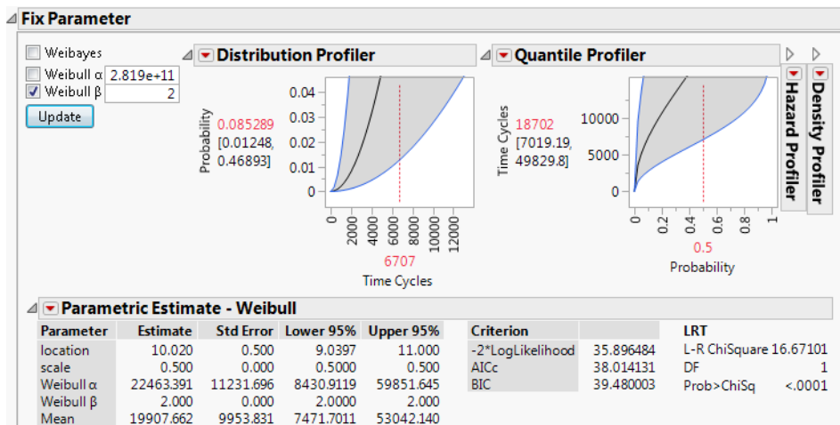
Figure 3.23 Fixed Parameter Model with Weibull Beta Specified
