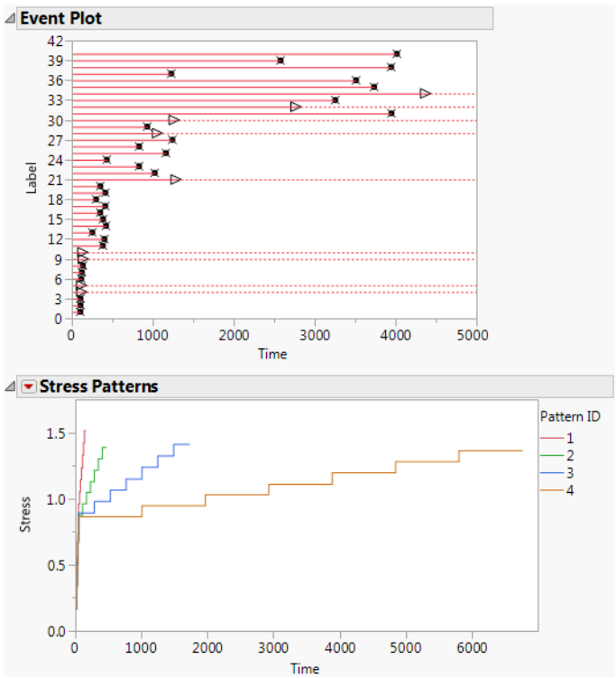
Figure 5.2 Event Plot and Stress Patterns Plot
