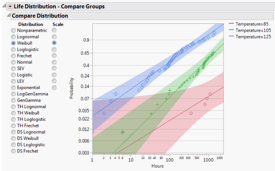
Figure 3.19 Compare Weibull Distribution for Groups
