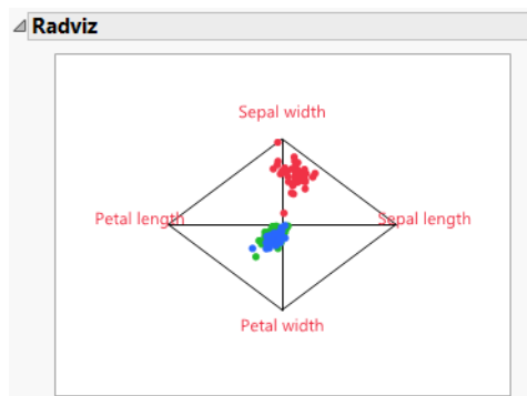
Figure 15.22 Iris.jmp Graph
