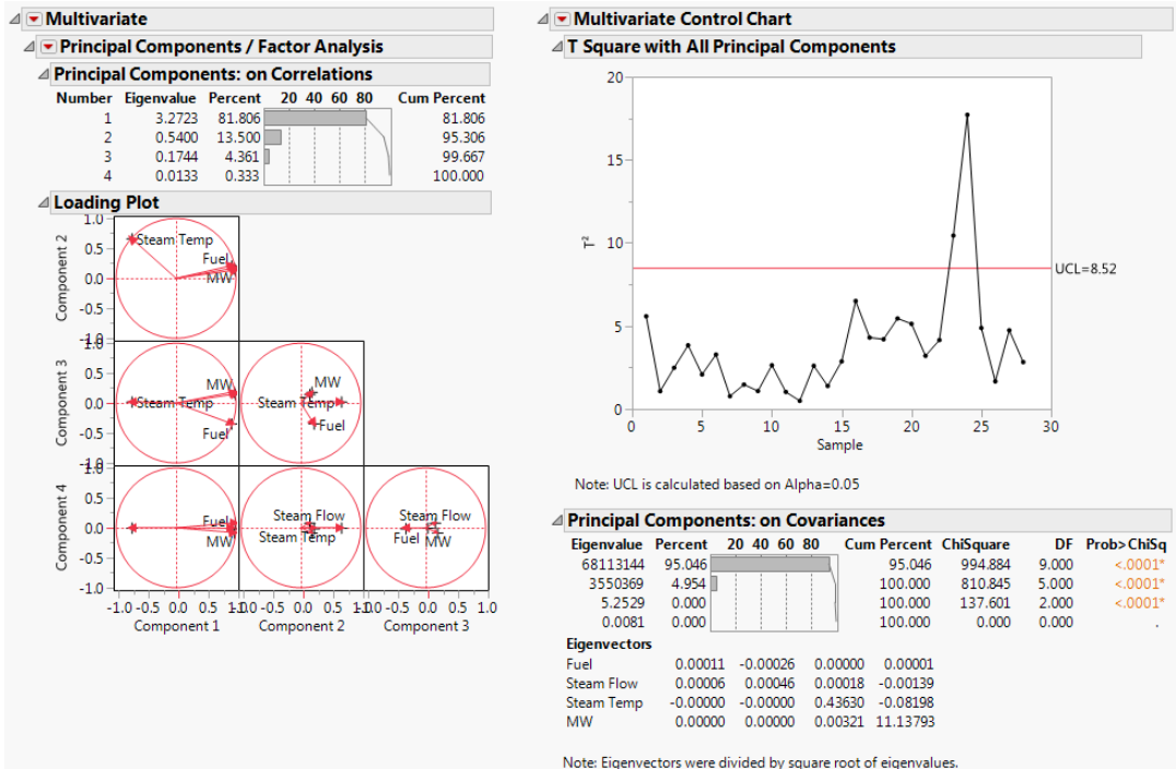
Figure 15.12 Multivariate Application
