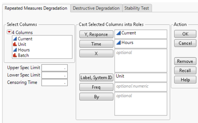
Figure 7.3 The Degradation Launch Window
