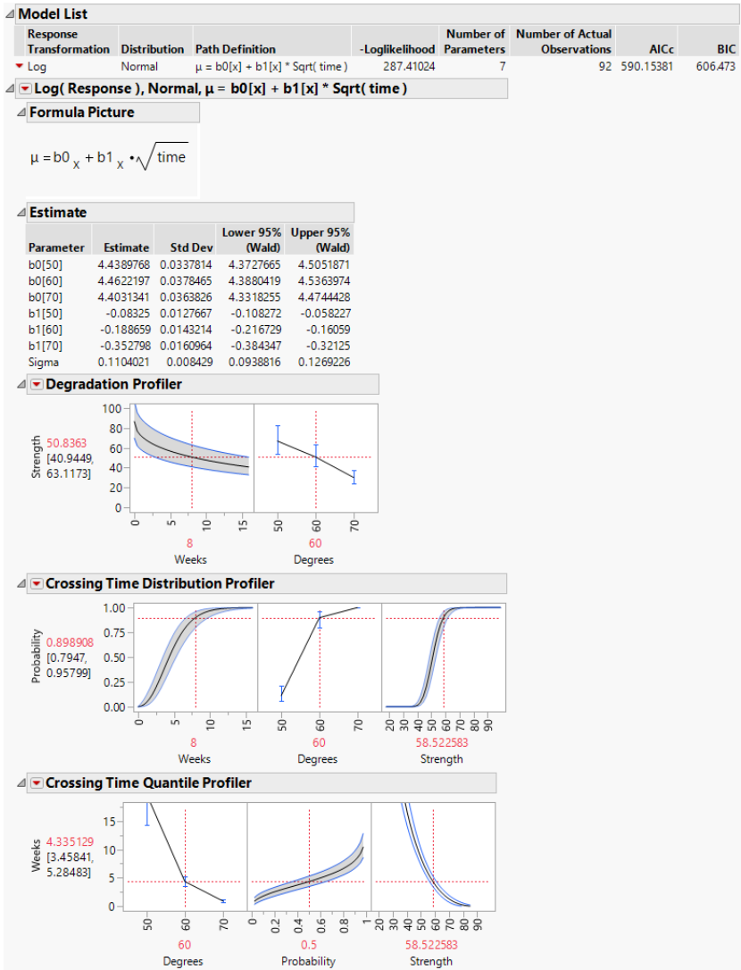
Figure 8.4 Report for Basic Model
