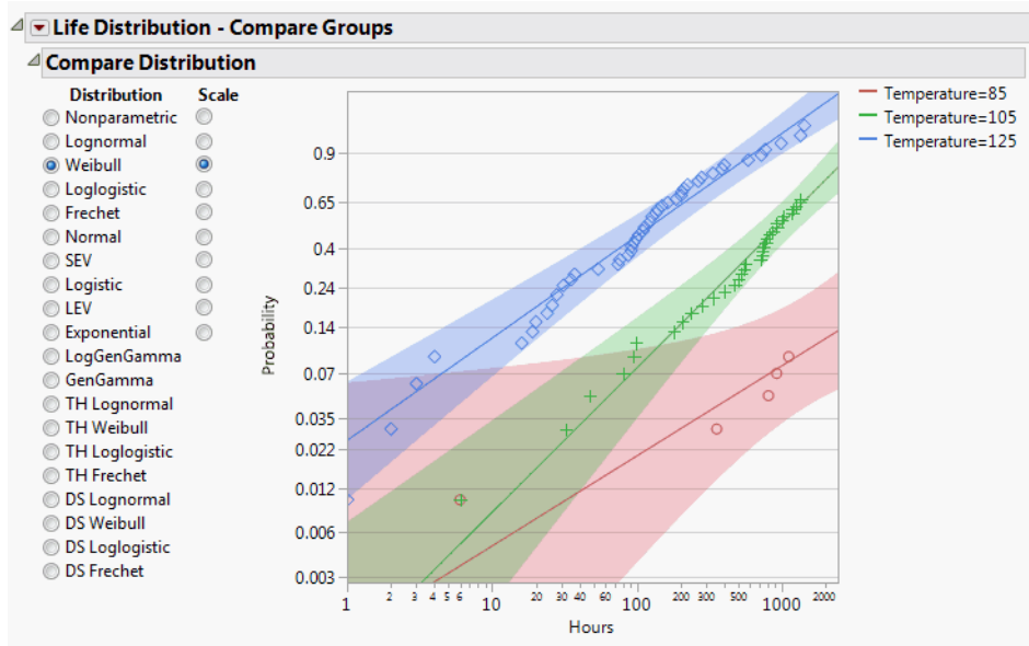
Figure 3.20 Compare Weibull Distribution for Groups
