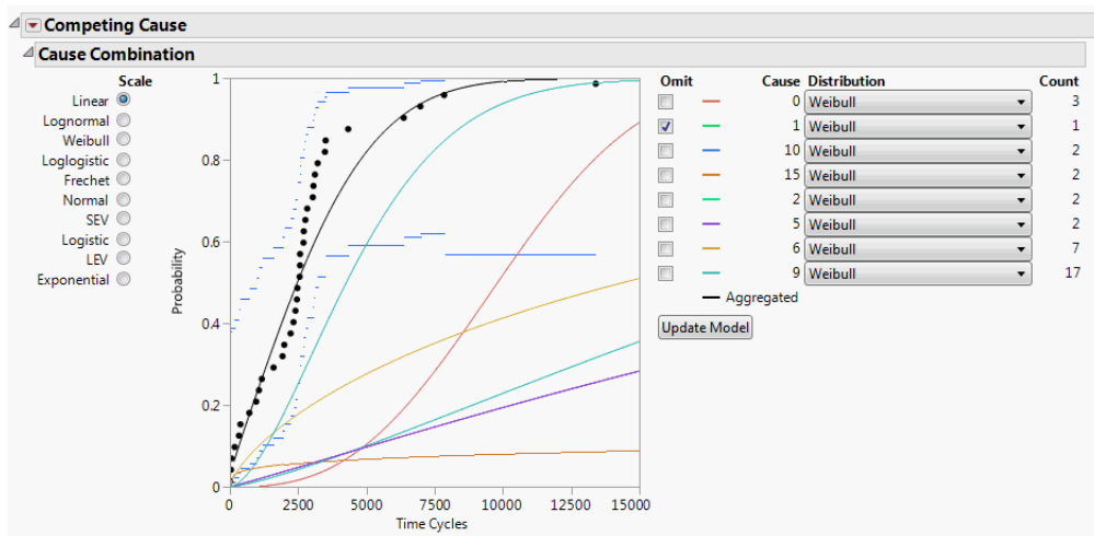
Figure 3.23 Fixed Parameter Model with Cause 1 Omitted
