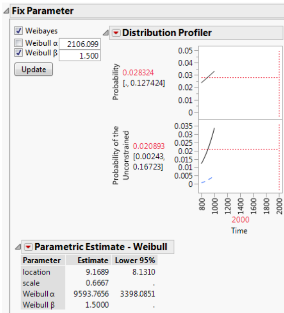
Figure 3.22 Life Distribution Report for One Failure
