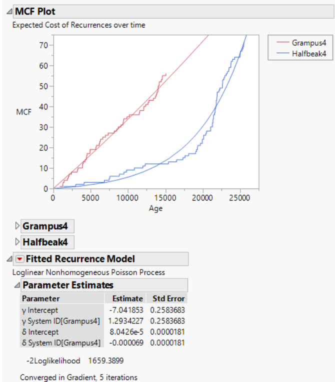
Figure 6.12 Diesel Ship Engines Report
