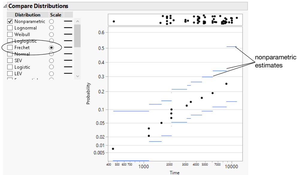
Figure 3.17 Nonparametric Estimates with a Fréchet Probability Scale
