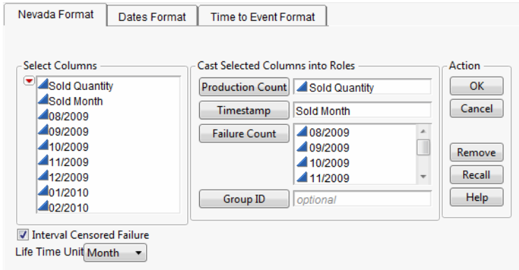
Figure 9.7 The Reliability Forecast Launch Window
