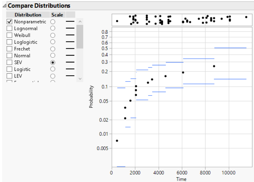
Figure 3.18 Nonparametric Estimates with a SEV Probability Scale
