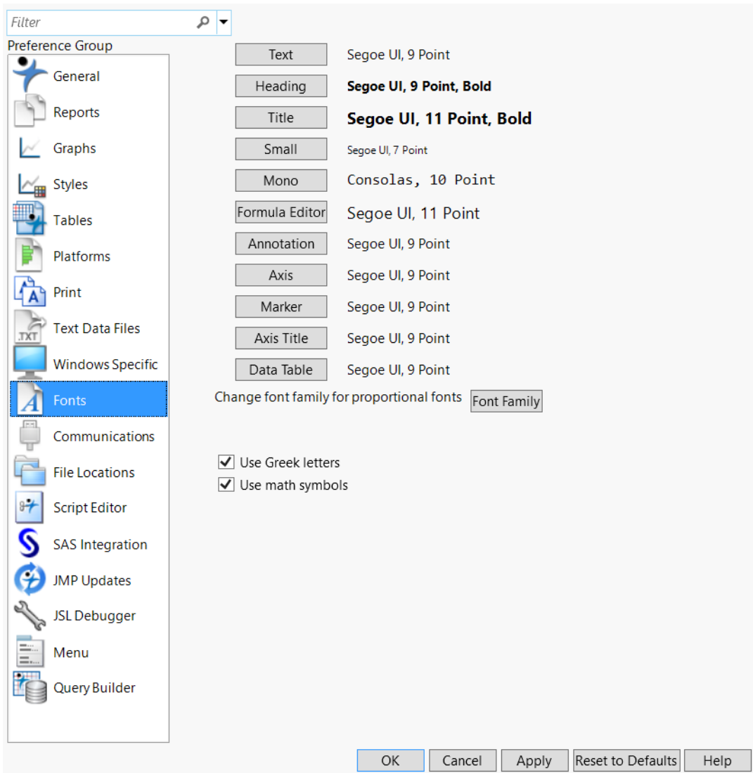
Figure 13.11 Fonts Preferences
