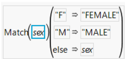
Figure 4.45 Recoded Column
