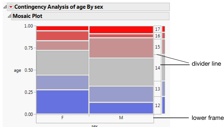
Figure 9.34 Divider Lines
