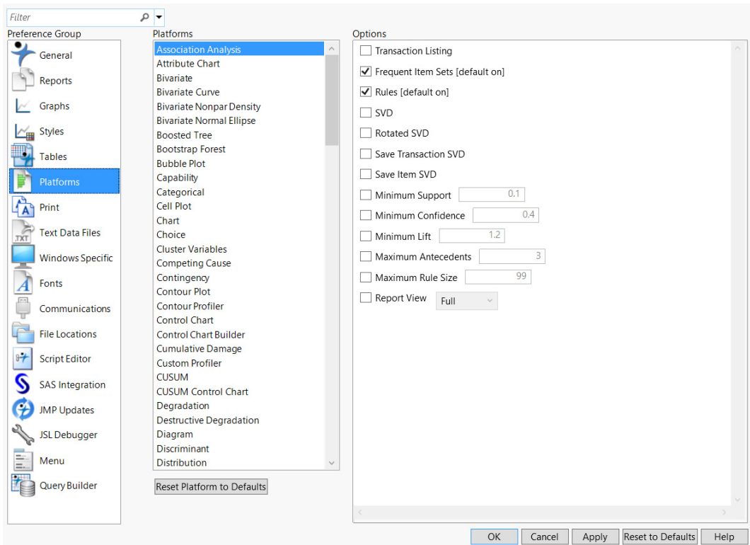
Figure 13.6 Platforms Preferences
