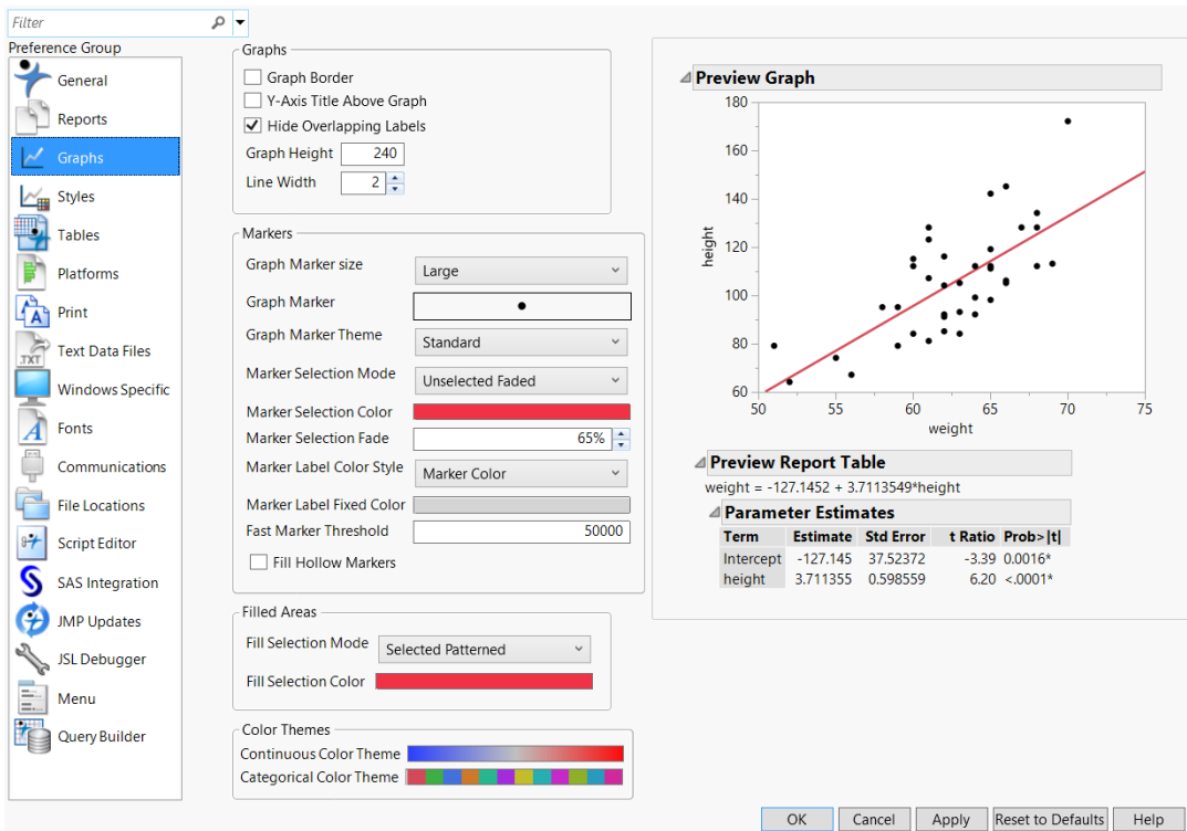
Figure 13.3 Graphs Preferences
