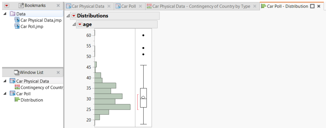
Figure 10.13 Tabbed Reports
