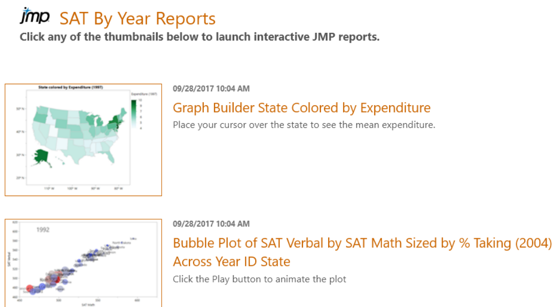
Figure 10.4 Web Report
