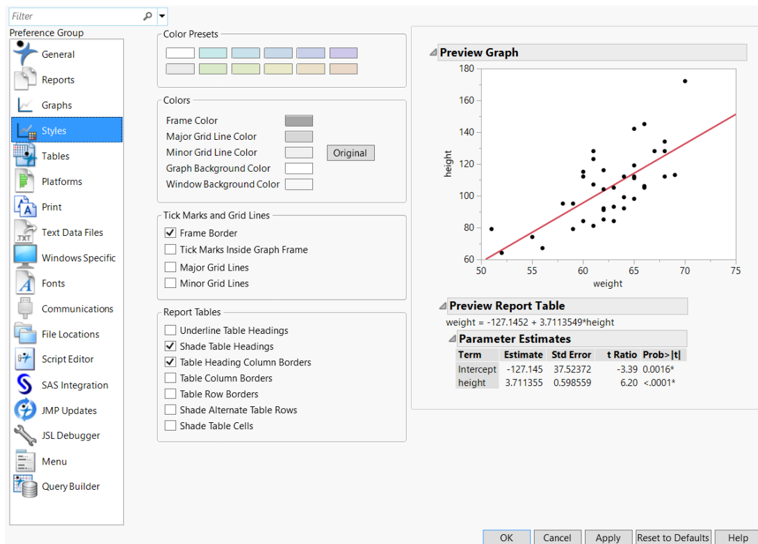
Figure 13.4 Styles Preferences
