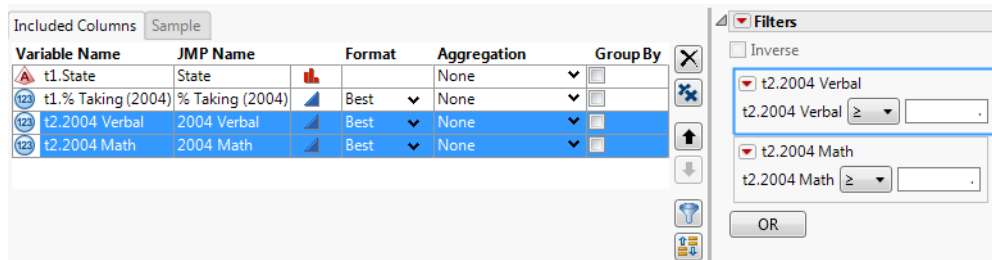
Figure 6.34 Selected Filters
