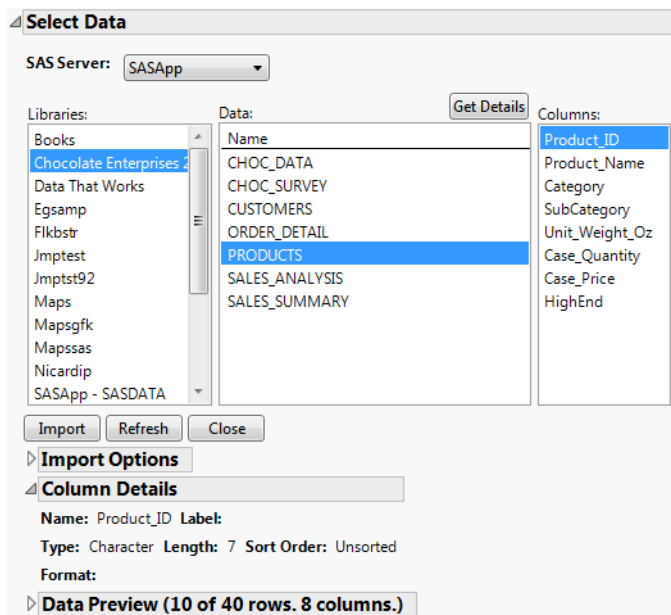
Figure 3.21 Column Details
