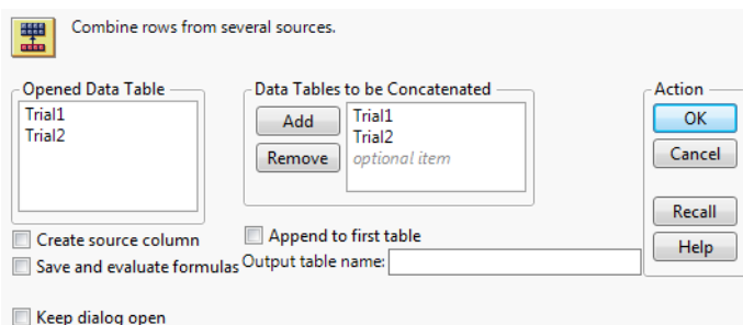
Figure 6.19 Concatenate Window
