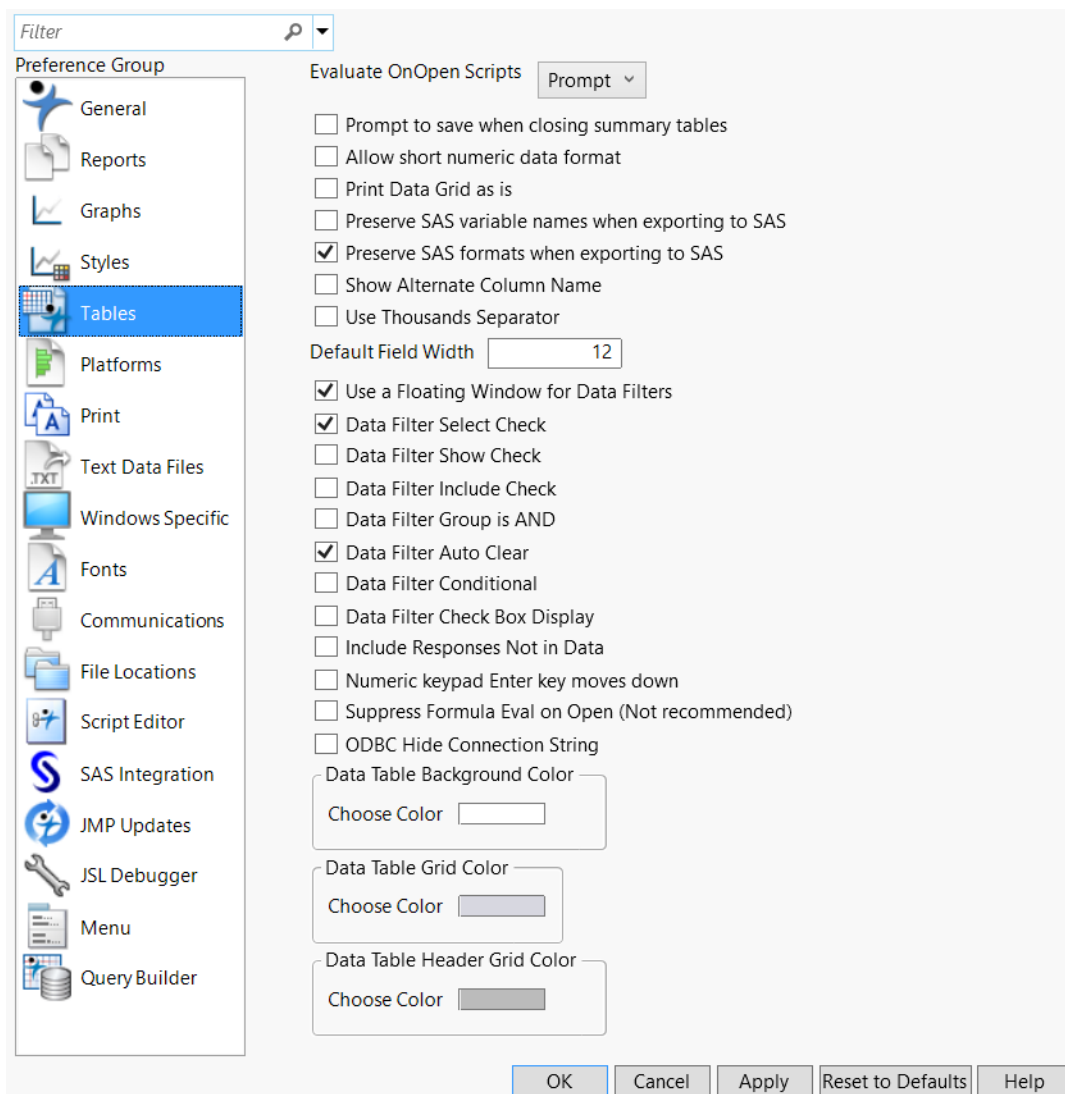
Figure 13.5 Tables Preferences
