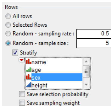
Figure 6.3 Stratified Subsets
