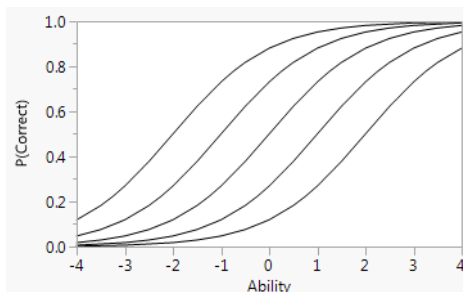
Figure 10.11 Logistic Curve for Several Values of b
