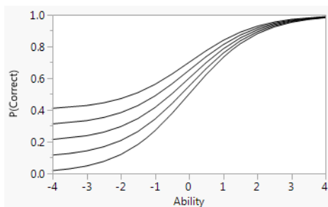
Figure 10.12 Logistic Model for Several Values of c
