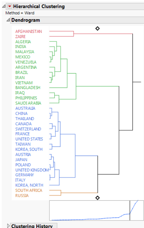
Figure 11.2 Hierarchical Clustering Report
