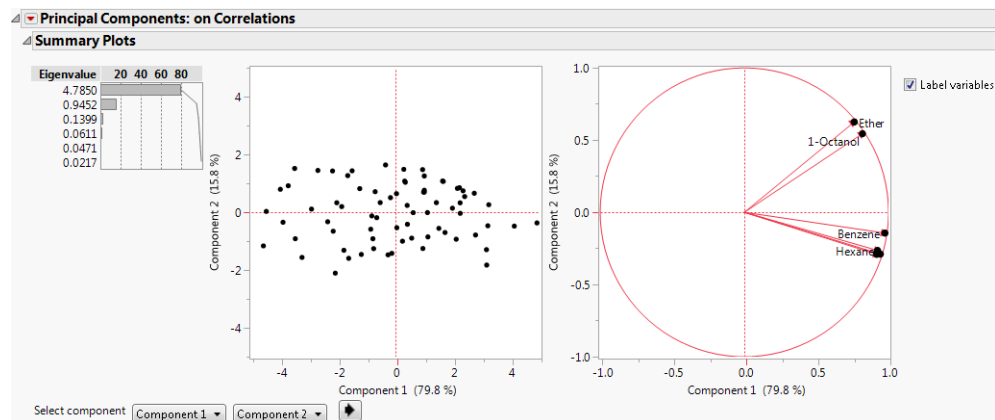
Figure 4.2 Principal Components on Correlations Report
