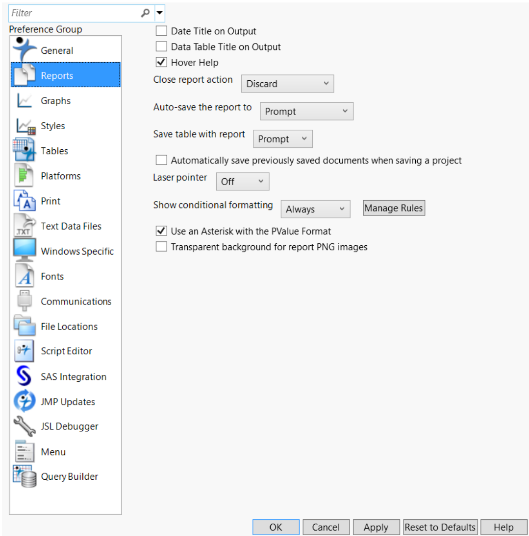
Figure 13.2 Reports Preferences
