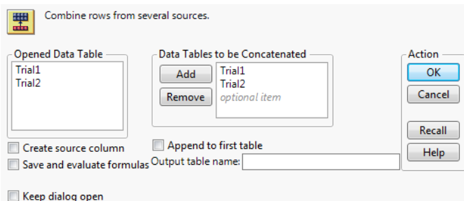
Figure 6.19 Concatenate Window
