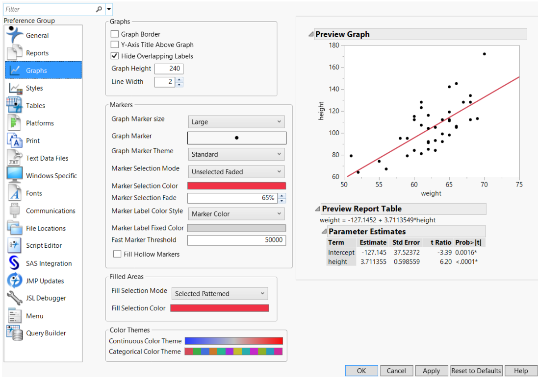
Figure 13.3 Graphs Preferences
