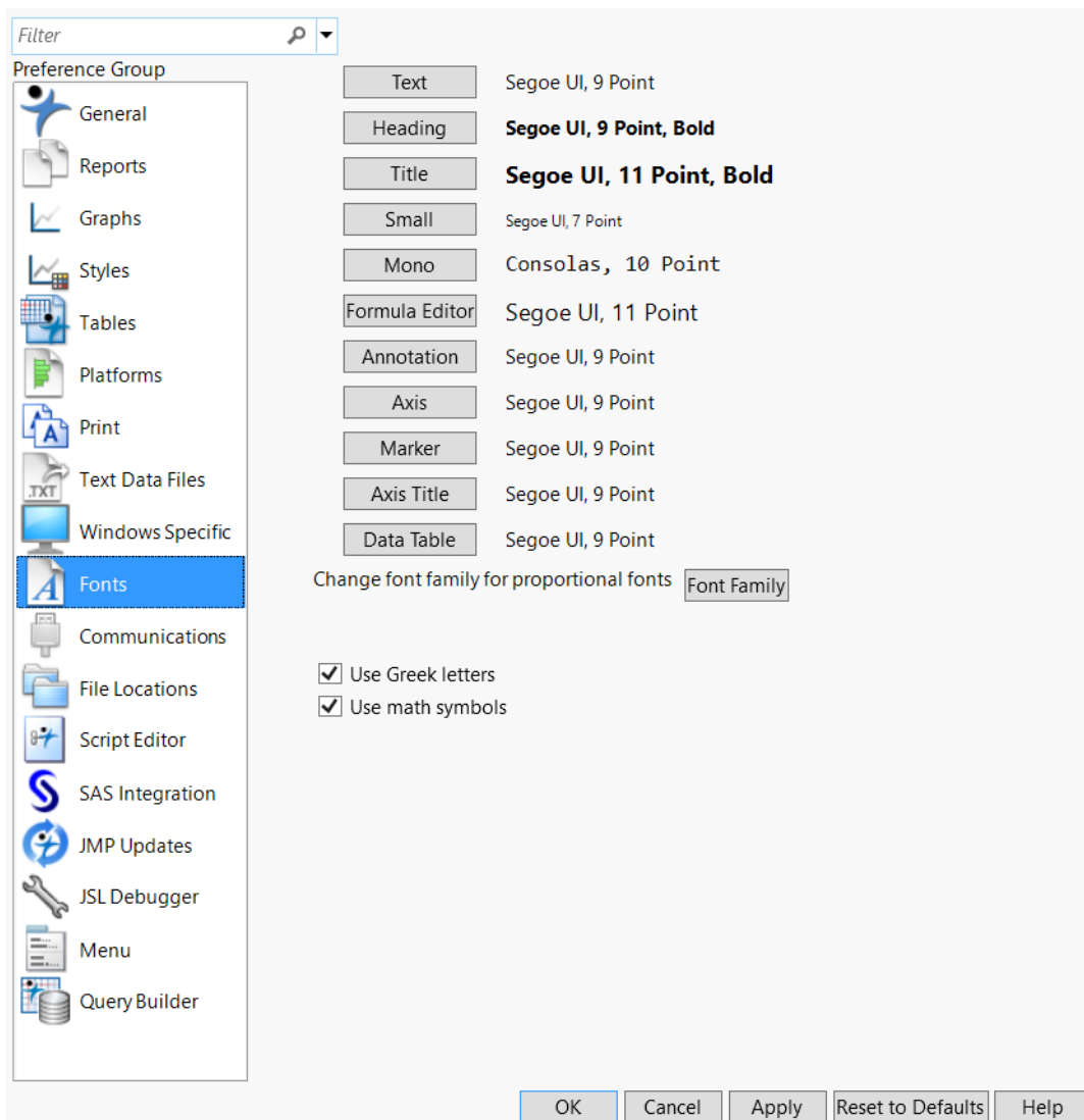
Figure 13.11 Fonts Preferences
