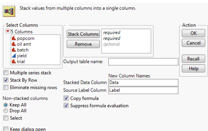
Figure 6.8 Stack Window
