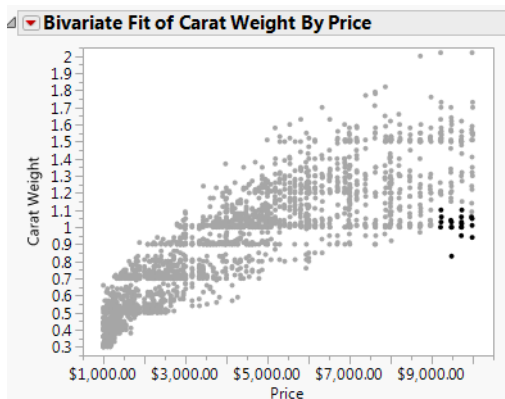
Figure 4.8 Points Selected
