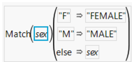
Figure 4.45 Recoded Column
