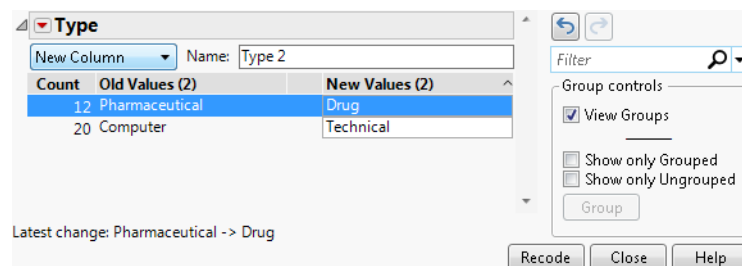
Figure 4.40 Recode Window
