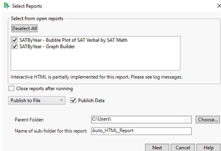
Figure 10.3 Selecting Reports
