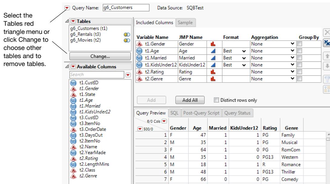
Figure 3.33 Selected Columns
