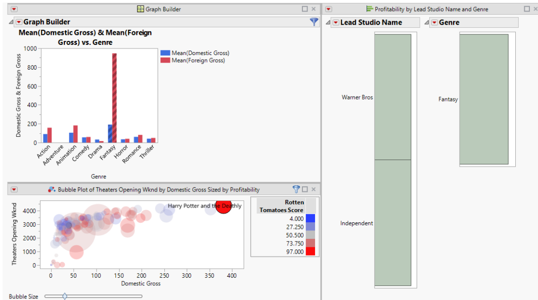
Figure 11.14 Filtering Data
