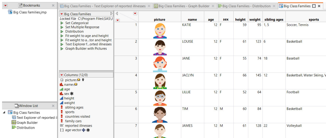
Figure 10.25 New Project
