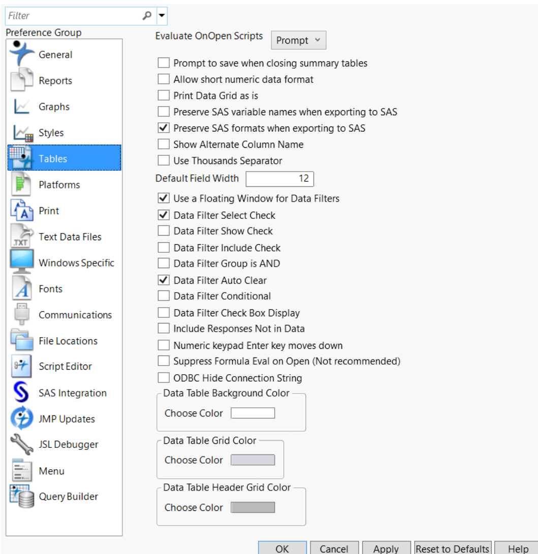
Figure 13.5 Tables Preferences
