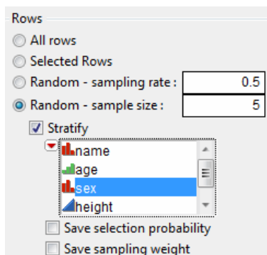
Figure 6.3 Stratified Subsets
