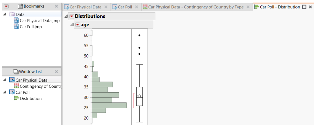
Figure 10.18 Tabbed Reports
