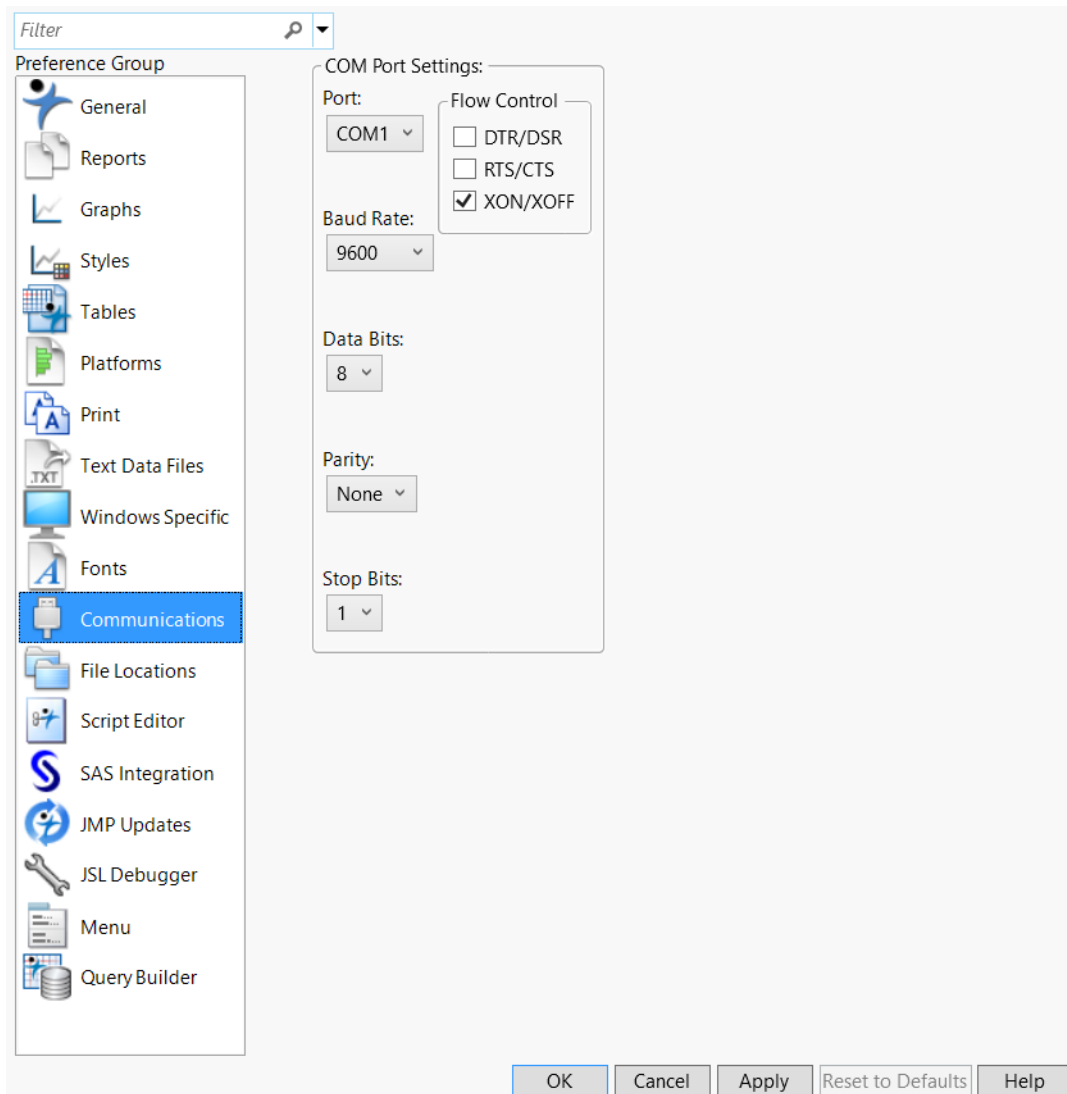
Figure 13.12 Communications Preferences
