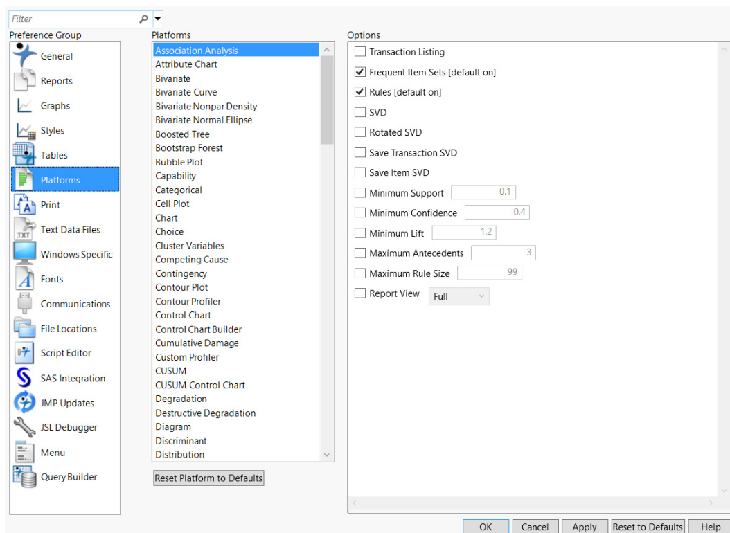
Figure 13.6 Platforms Preferences
