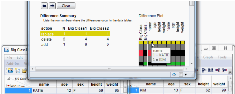
Figure 4.23 Modified Data
