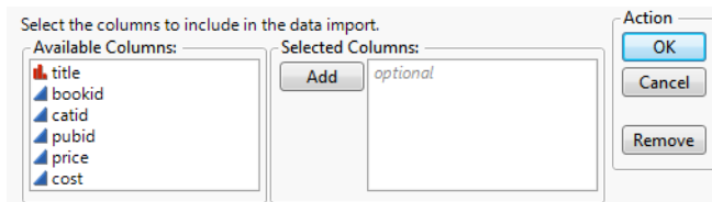
Figure 3.23 Select Columns
