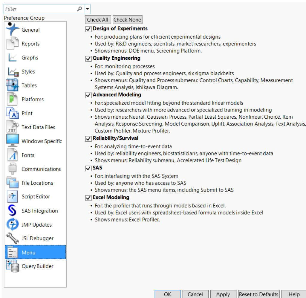
Figure 13.18 Menu Preferences
