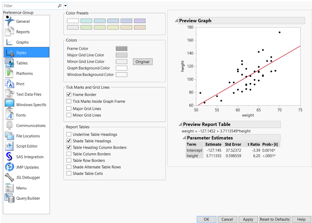
Figure 13.4 Styles Preferences
