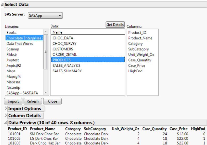
Figure 3.20 Data Preview
