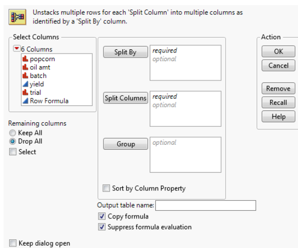
Figure 6.12 Split Window
