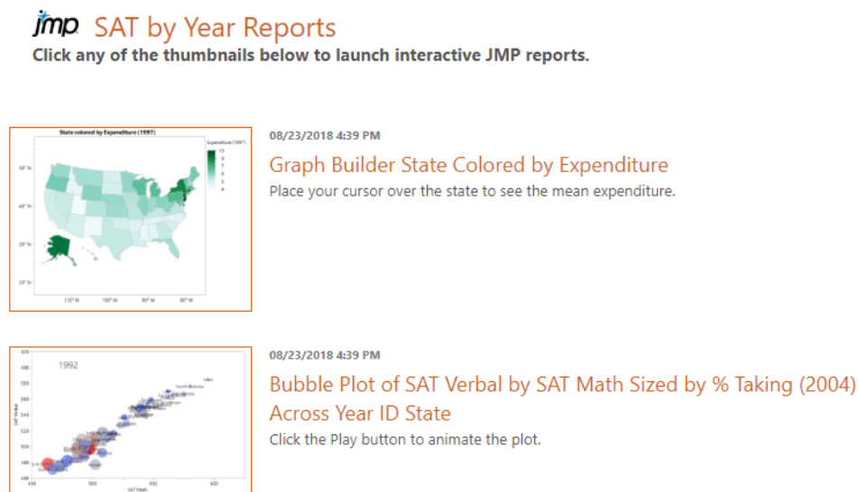
Figure 10.5 Web Report
