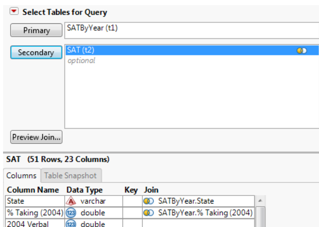
Figure 6.33 Joined Columns
