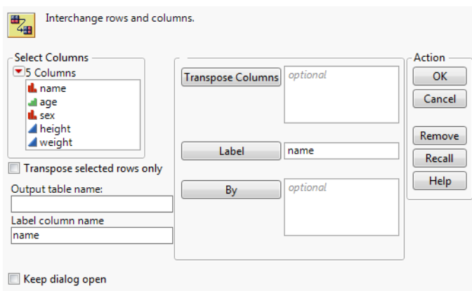
Figure 6.15 Transpose Window
