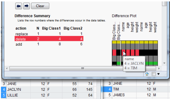
Figure 4.24 Deleted Rows
