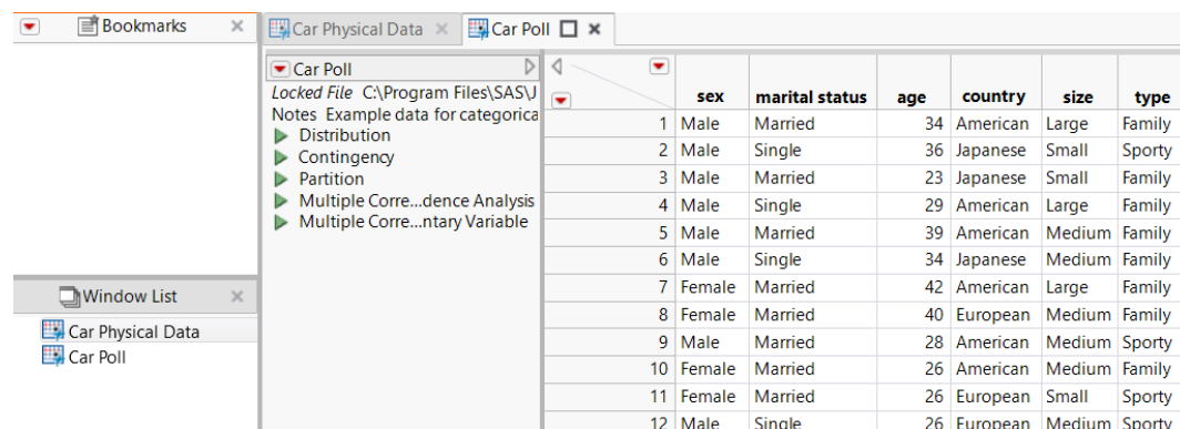
Figure 10.16 Initial Project
