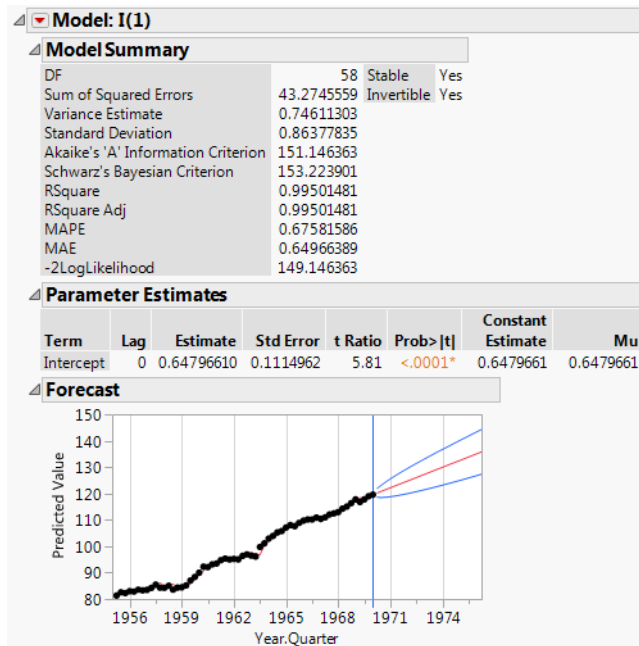
Figure 17.21 Model Report for ARIMA(0,1,0)
