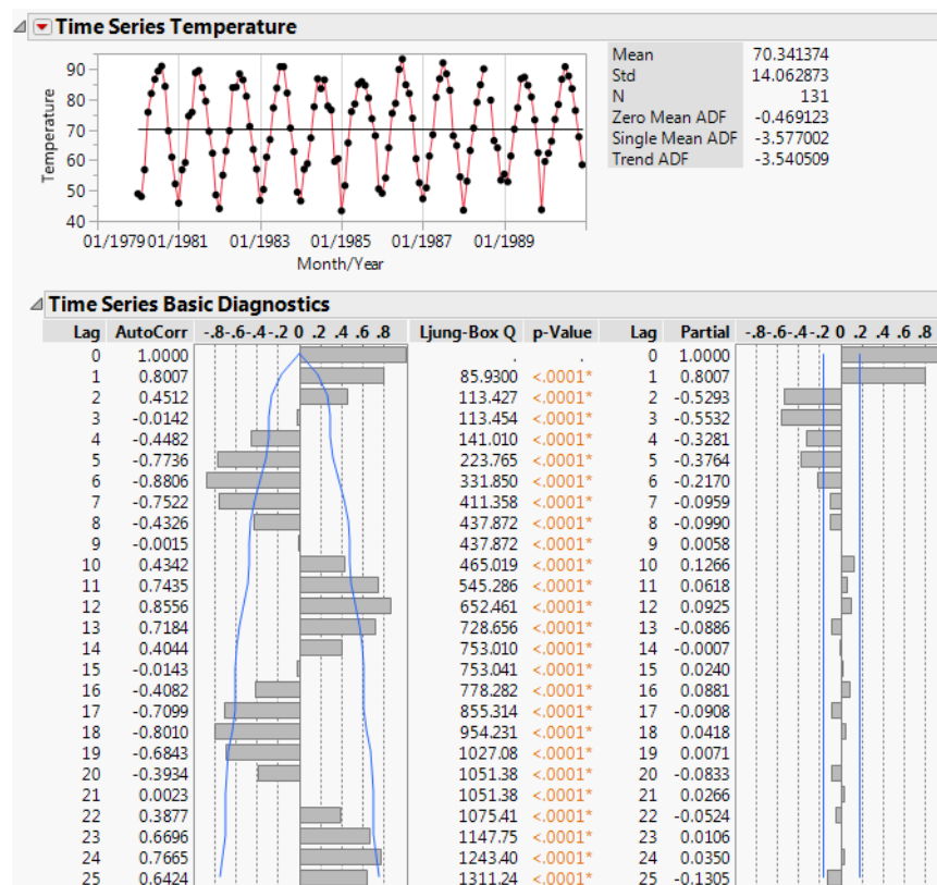
Figure 17.2 Time Series Analysis Report for Raleigh Temps.jmp
