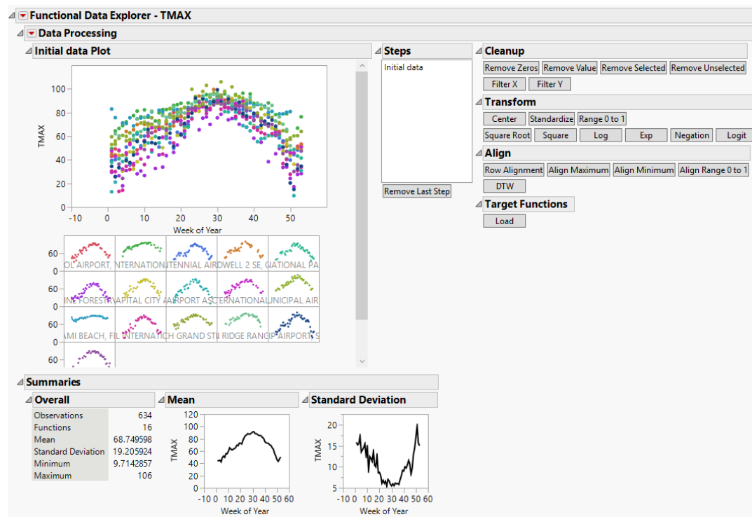
Figure 15.2 Initial Functional Data Explorer Report
