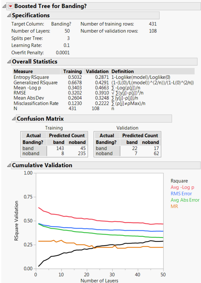
Figure 6.9 Boosted Tree Report for a Categorical Response
