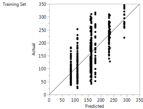
Figure 4.16 Actual by Predicted Plots for a Continuous Response
