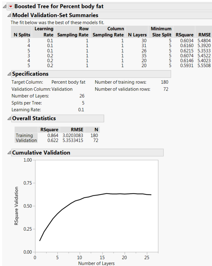
Figure 6.8 Boosted Tree Report for a Continuous Response
