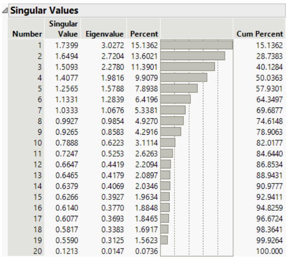
Figure 24.8 Singular Values Table
