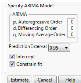
Figure 17.6 ARIMA Specification Window
