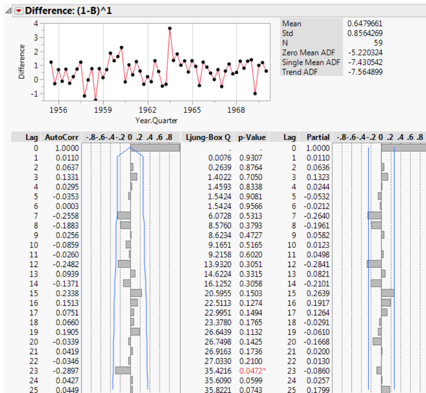
Figure 17.18 Difference Report for SeriesP.jmp
