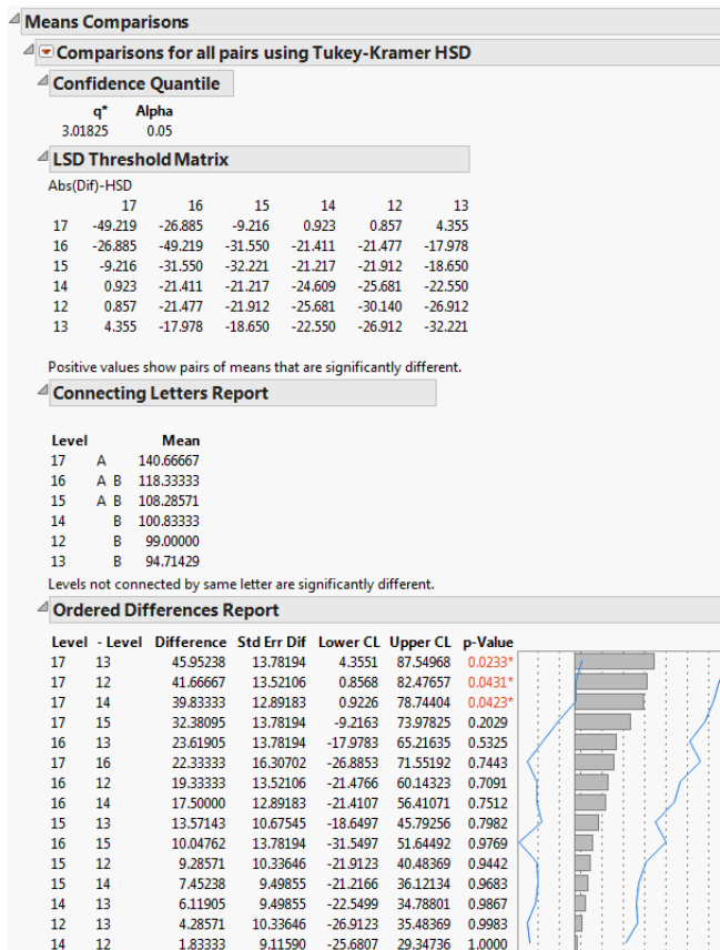
Figure 6.18 Example of Means Comparisons Report for All Pairs, Tukey HSD
