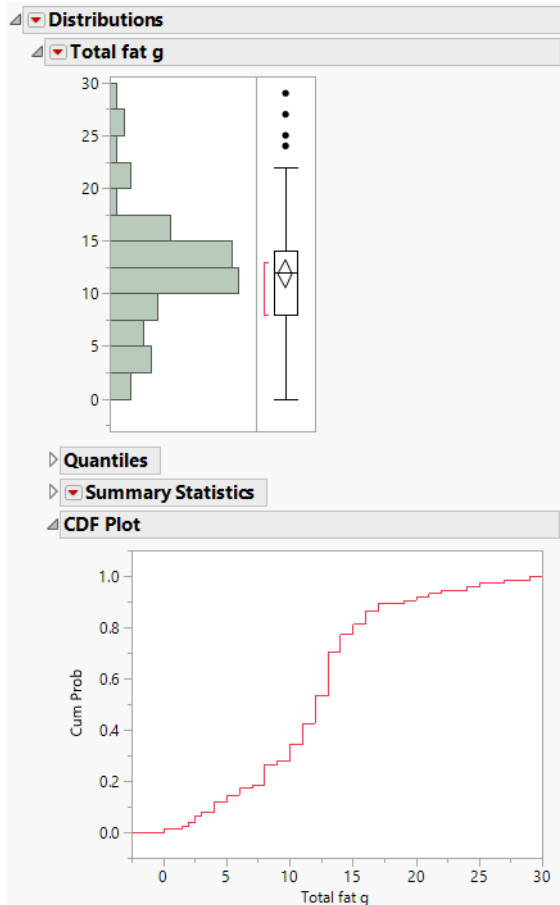
Figure 3.10 CDF Plot
