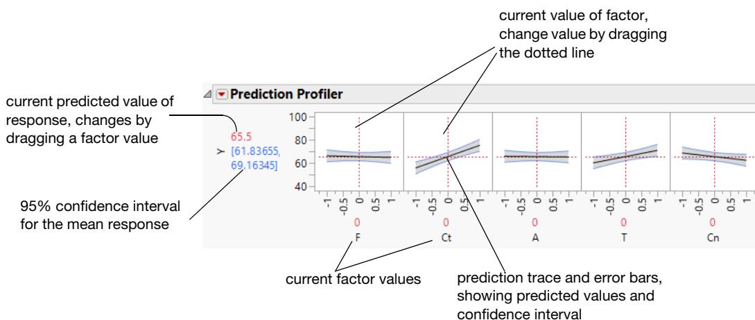
Figure 3.48 Illustration of Prediction Traces
