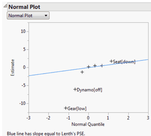
Figure 3.44 Normal Plot
