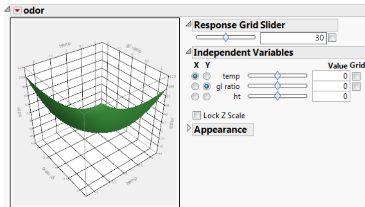
Figure 3.54 Surface Plot
