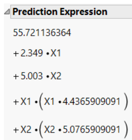
Figure 4.13 Prediction Expression
