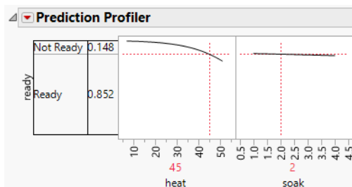
Figure 11.3 Prediction Profiler
