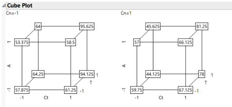
Figure 3.52 Cube Plots
