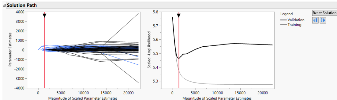
Figure 6.2 Solution Path Plot
