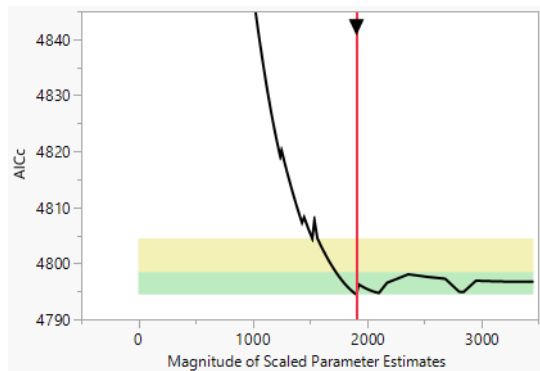
Figure 6.6 Validation Plot for Diabetes.jmp, Lasso with AICc Validation
