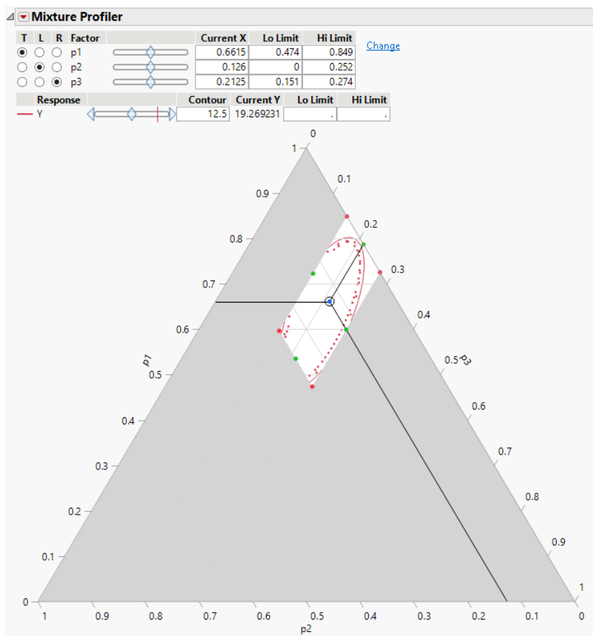
Figure 3.51 Mixture Profiler
