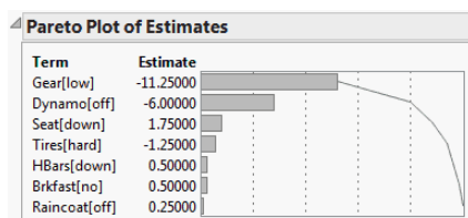
Figure 3.47 Pareto Plot
