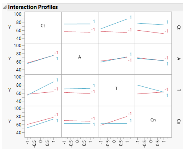
Figure 3.49 Interaction Plots
