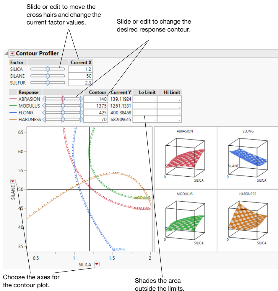
Figure 3.50 Contour Profiler
