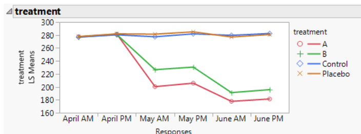
Figure 9.11 Treatment Graph
