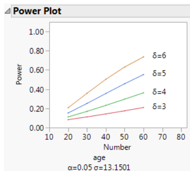
Figure 3.68 Plot of Power by Sample Size
