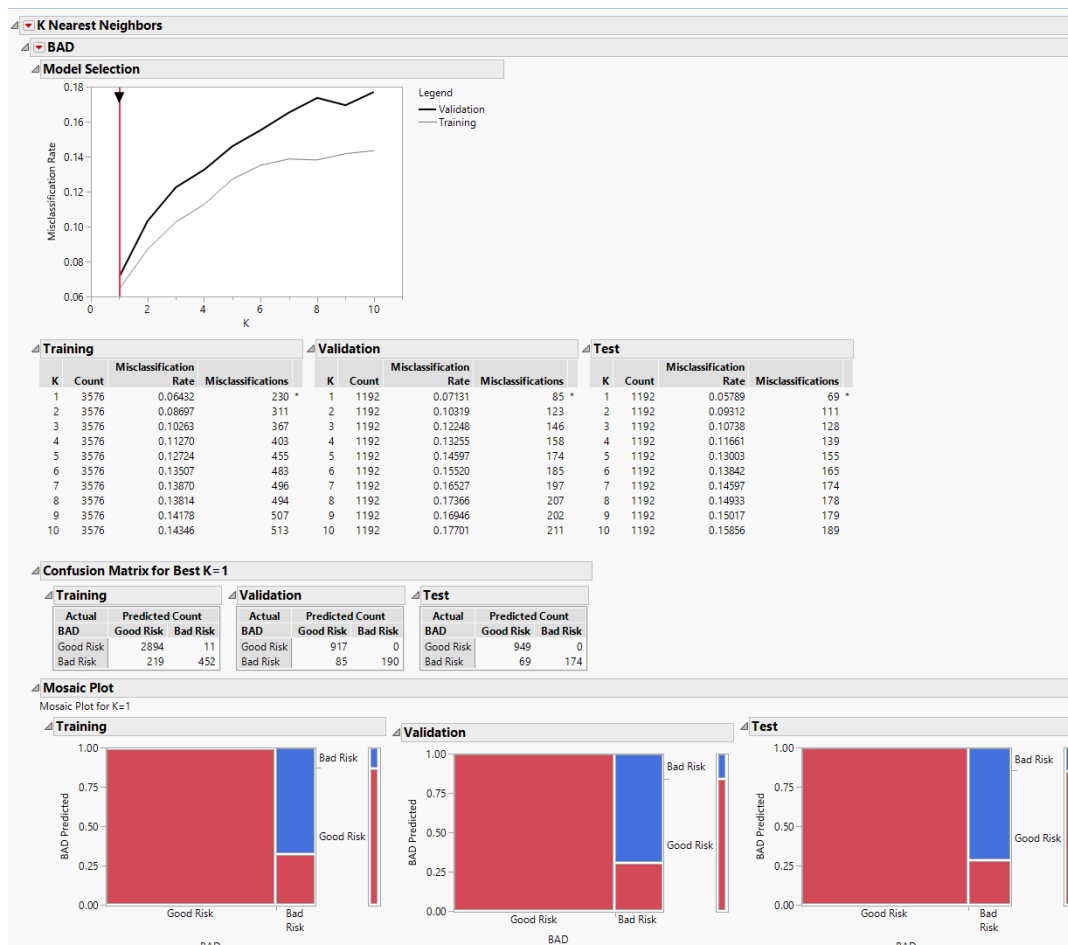
Figure 7.2 K Nearest Neighbors Report
