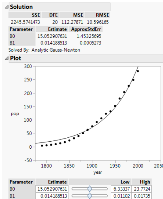
Figure 15.4 Plot and Solution Report
