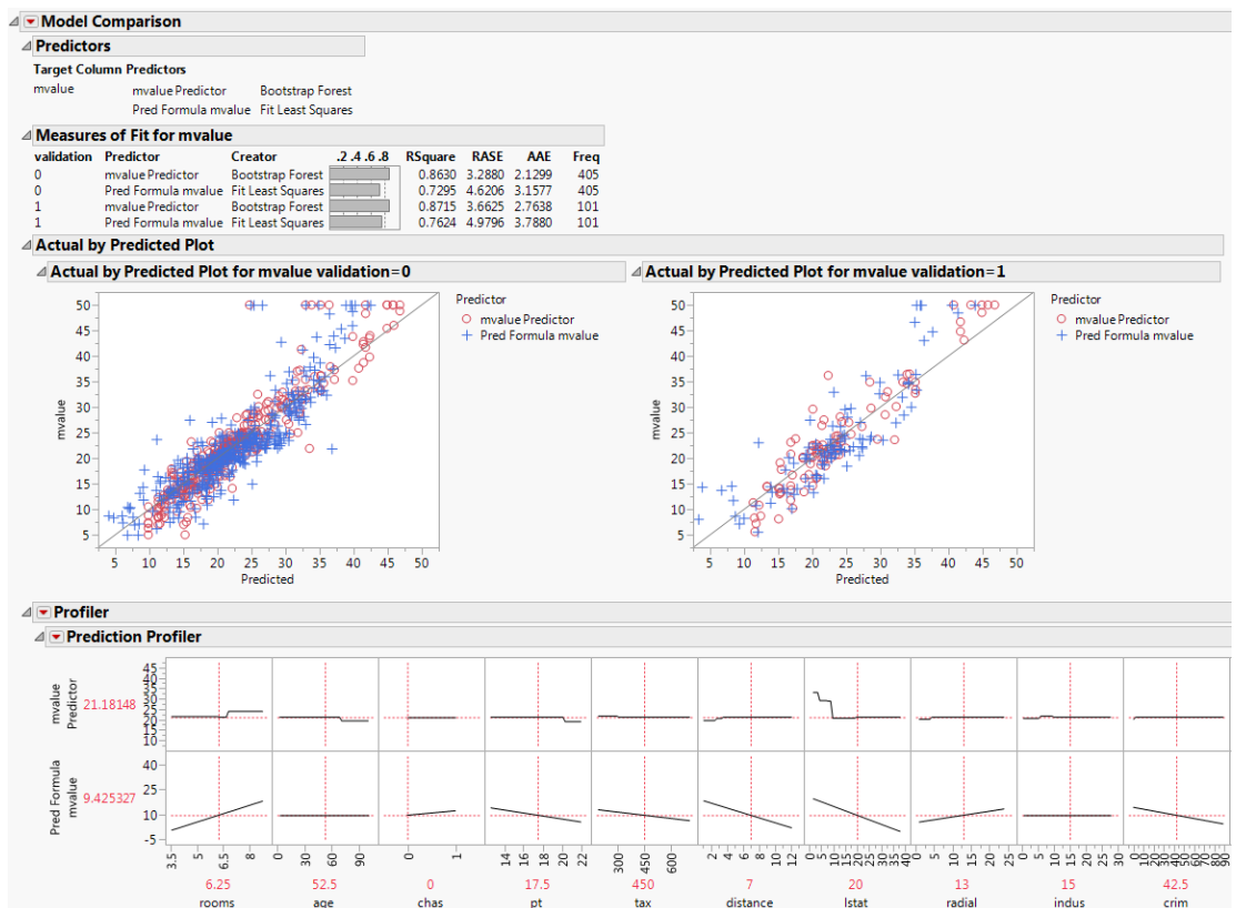
Figure 11.1 Example of Comparing Models
