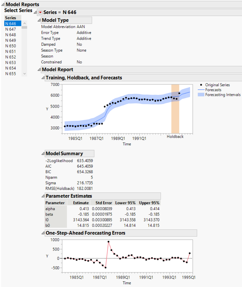
Figure 19.3 Model Reports
