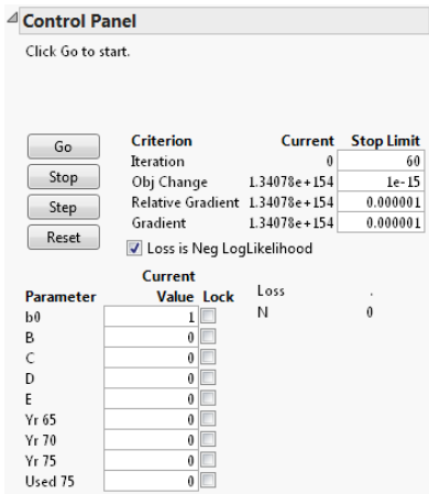
Figure 15.16 Enter New Parameters
