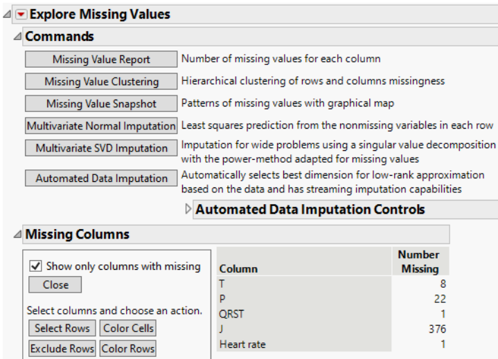
Figure 21.10 Missing Value Report
