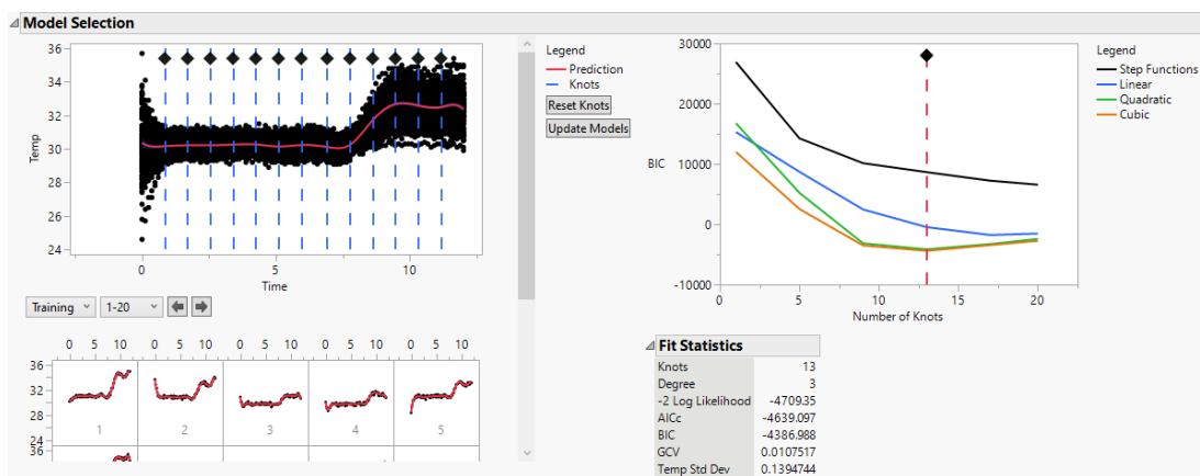
Figure 16.1 B-Spline Model Selection in FDE
