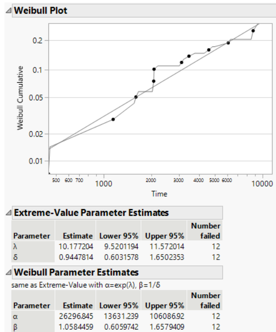
Figure 13.9 Weibull Output for Fan Data
