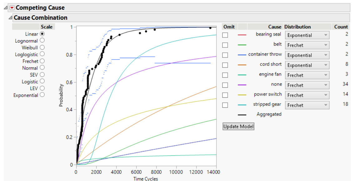
Figure 3.11 Initial Competing Cause Report
