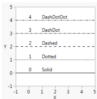
Figure 12.21 Line Styles
