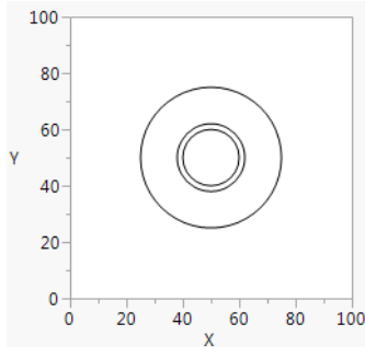
Figure 12.15 Drawing Circles
