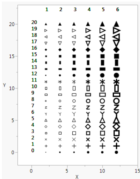
Figure 12.13 Drawing Markers
