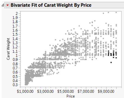
Figure 4.9 Points Selected
