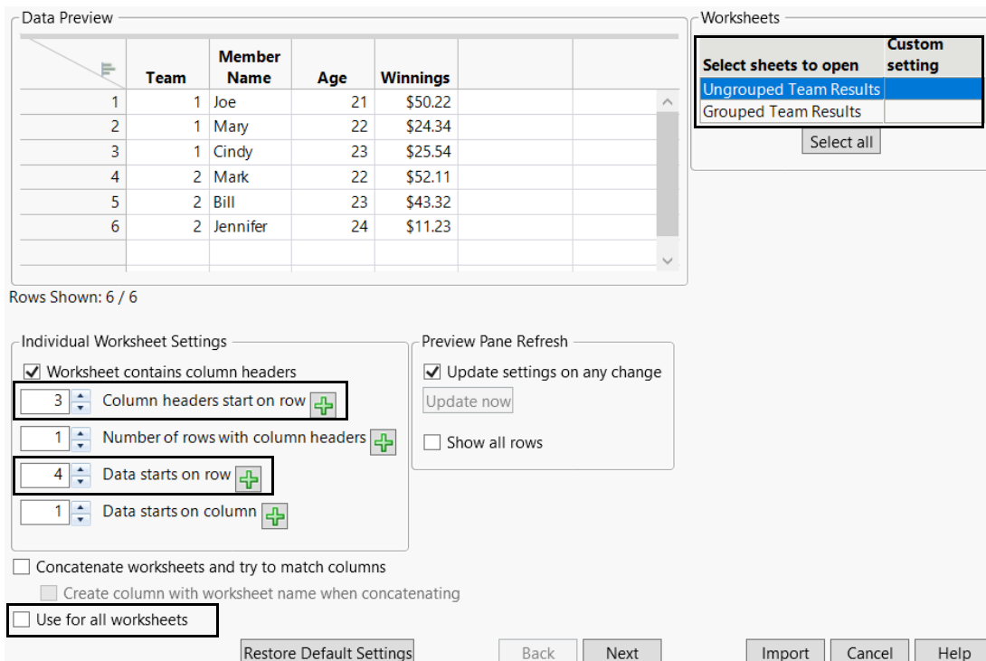
Figure 3.4 Selecting the Column Header Row
