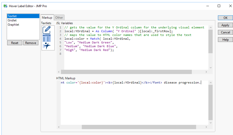
Figure 9.56 JSL Variables and HTML Markup for Textlet
