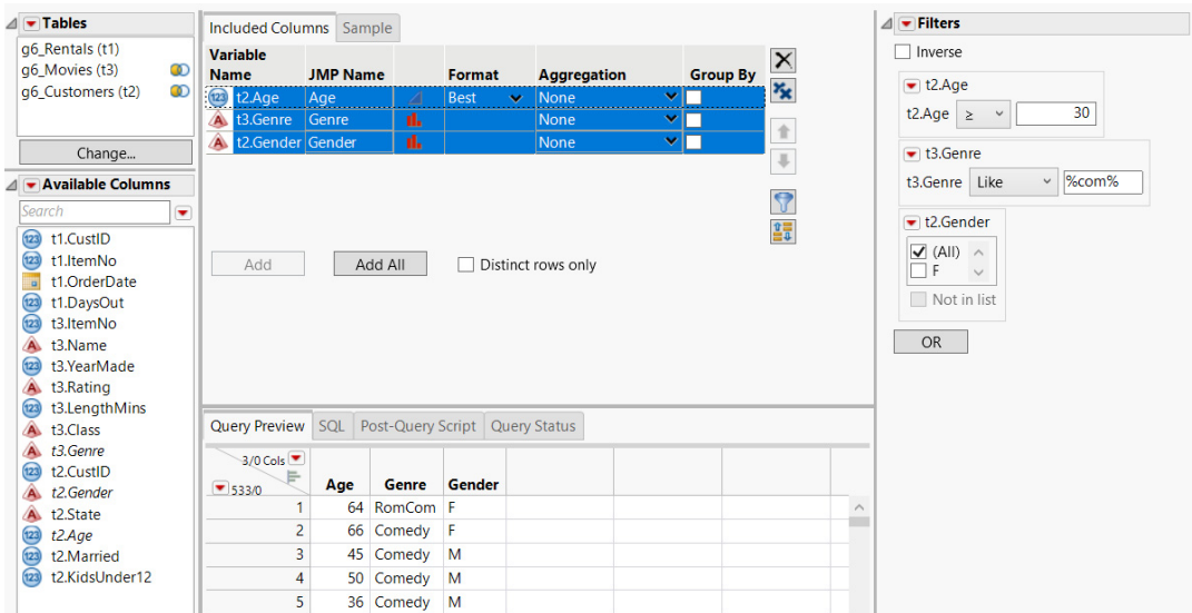
Figure 3.46 Selecting Filters
