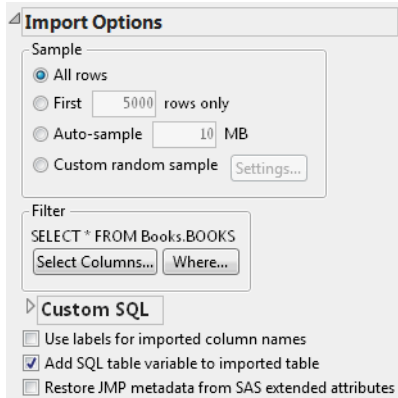
Figure 3.59 Import Options
