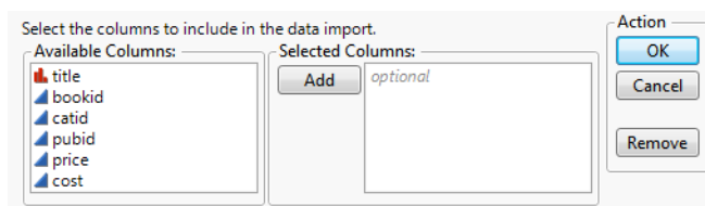
Figure 3.60 Select Columns
