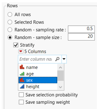
Figure 6.3 Stratified Subsets
