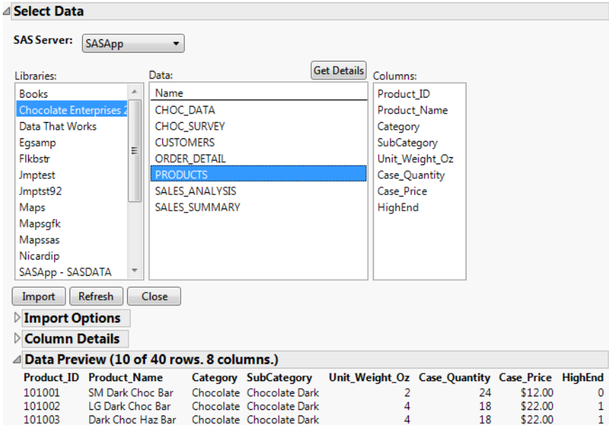
Figure 3.57 Data Preview
