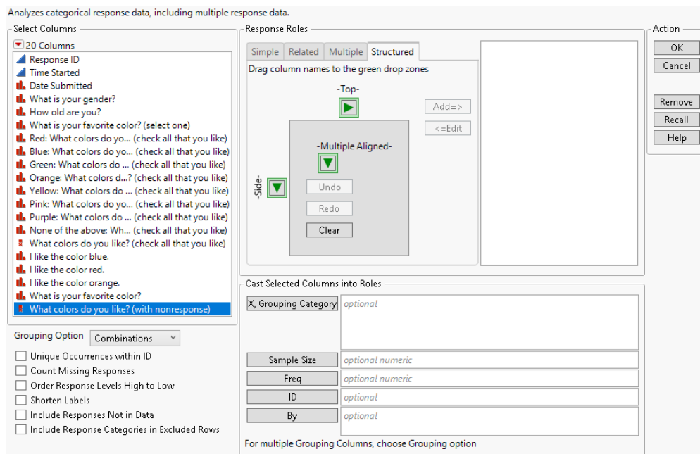
Figure 3.15 Categorical Platform Launch Window for the Structured Tab
