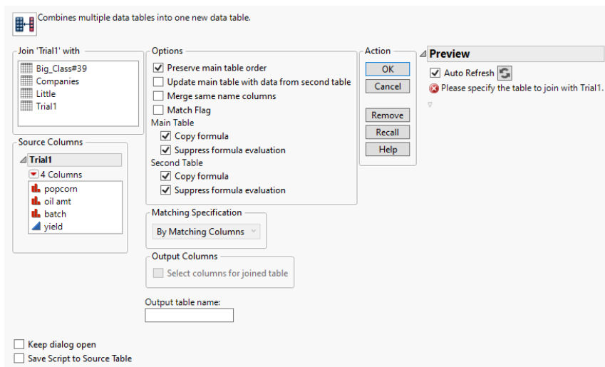
Figure 3.27 Completed Join Window
