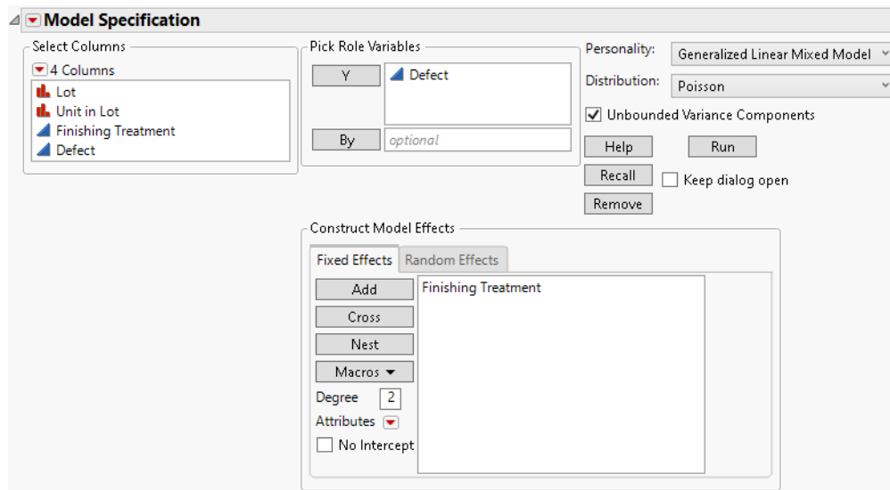
Figure 9.9 Completed Fit Model Launch Window Showing Fixed Effects
