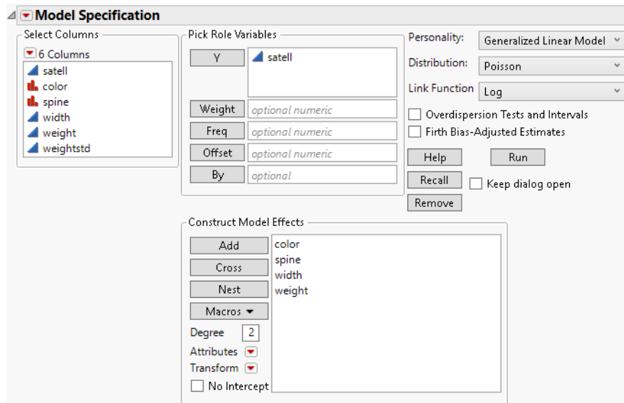
Figure 13.4 Fit Model Launch Window with Generalized Linear Model Selected
