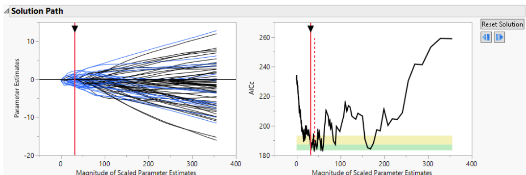
Figure 7.9 Smallest in Green Zone Model
