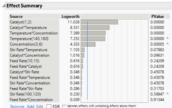
Figure 3.61 Effect Summary Table with Effect Heredity for Reactor 32 Runs.jmp
