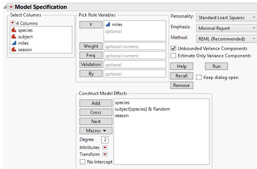
Figure 4.19 Fit Model Dialog
