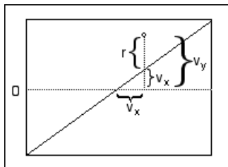
Figure 3.67 Construction of Leverage Plot
