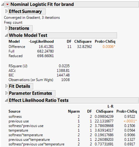
Figure 12.9 Nominal Logistic Fit for Three-Factor Factorial Model
