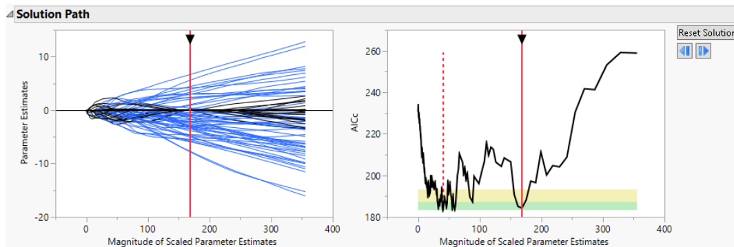
Figure 7.11 Biggest in Green Zone Model
