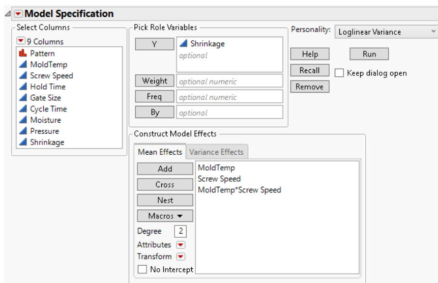
Figure 11.3 Fit Model Launch Window with Loglinear Variance Selected
