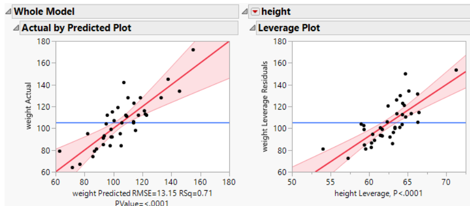
Figure 3.52 Whole Model and Effect Leverage Plots
