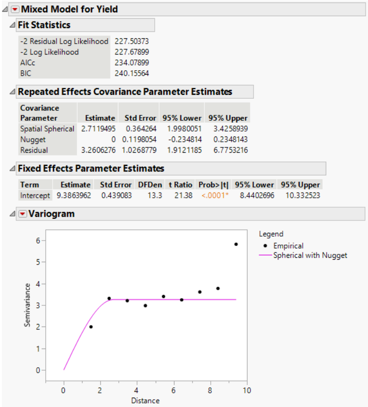
Figure 8.34 Mixed Model Report for Spatial Spherical with Nugget
