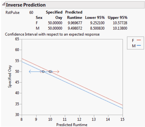
Figure 3.33 Inverse Prediction Report for a Multiple Regression Model
