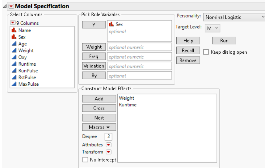
Figure 5.22 Model Specification Window for Reduced Model
