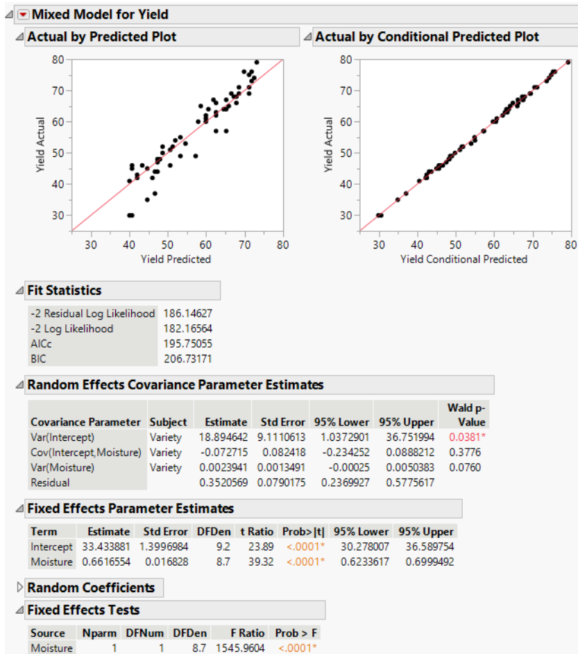
Figure 8.5 Mixed Model Report
