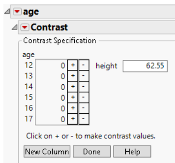
Figure 3.14 LSMeans Contrast Specification for age
