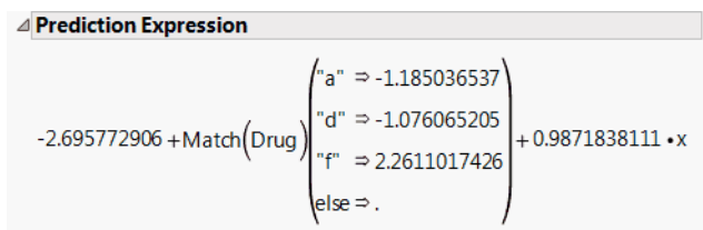
Figure 3.20 Prediction Expression
