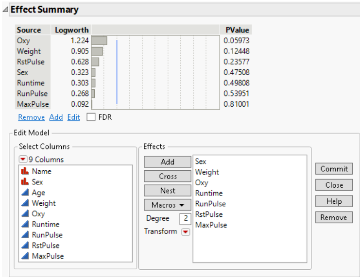
Figure 3.60 Effect Summary Edit Model Panel
