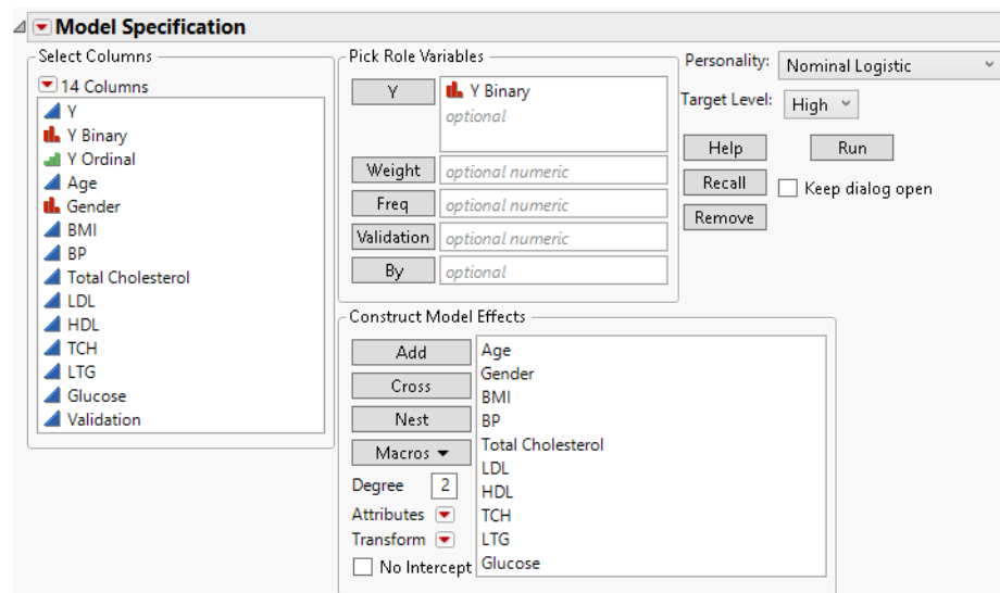
Figure 12.5 Fit Model Launch Window with Nominal Logistic Selected
