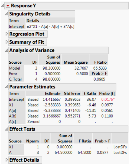
Figure 3.66 Fit Least Squares Report for Model with X1 and A
