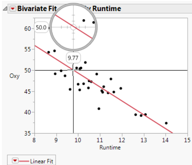
Figure 3.29 Bivariate Fit for Fitness.jmp
