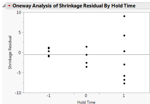
Figure 11.6 Residual by Dispersion Effect
