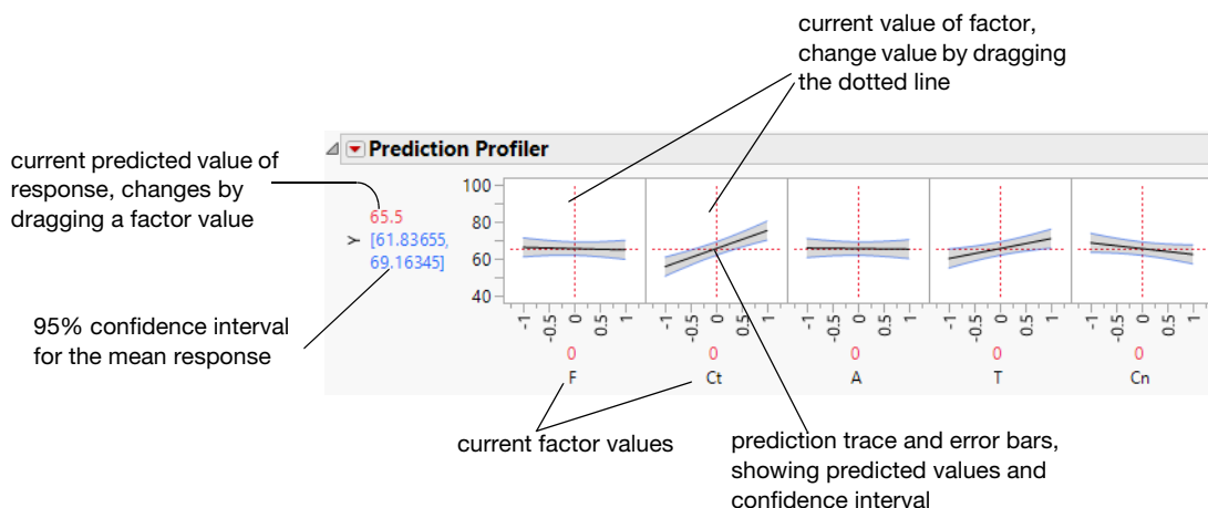
Figure 3.43 Illustration of Prediction Traces
