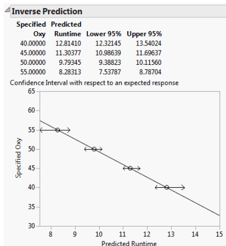
Figure 3.31 Inverse Prediction Report
