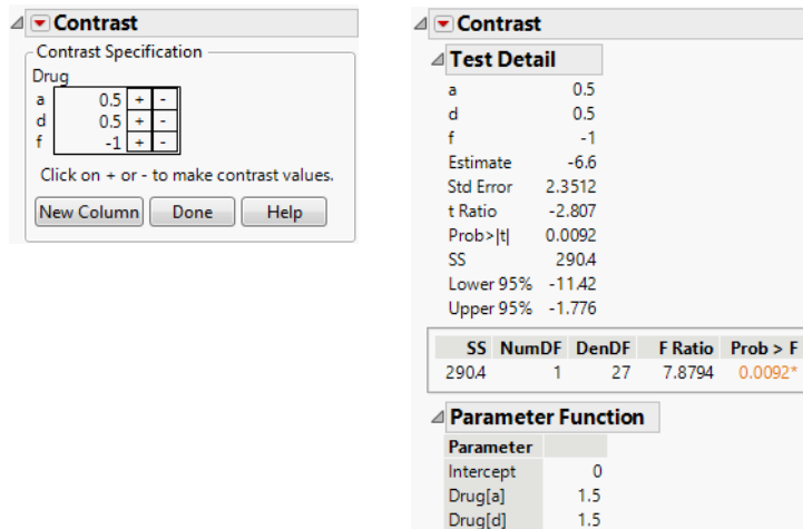
Figure 4.3 Contrast Example for the Drug Experiment
