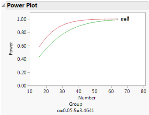
Figure 3.75 Power Plot for Bacteria Study
