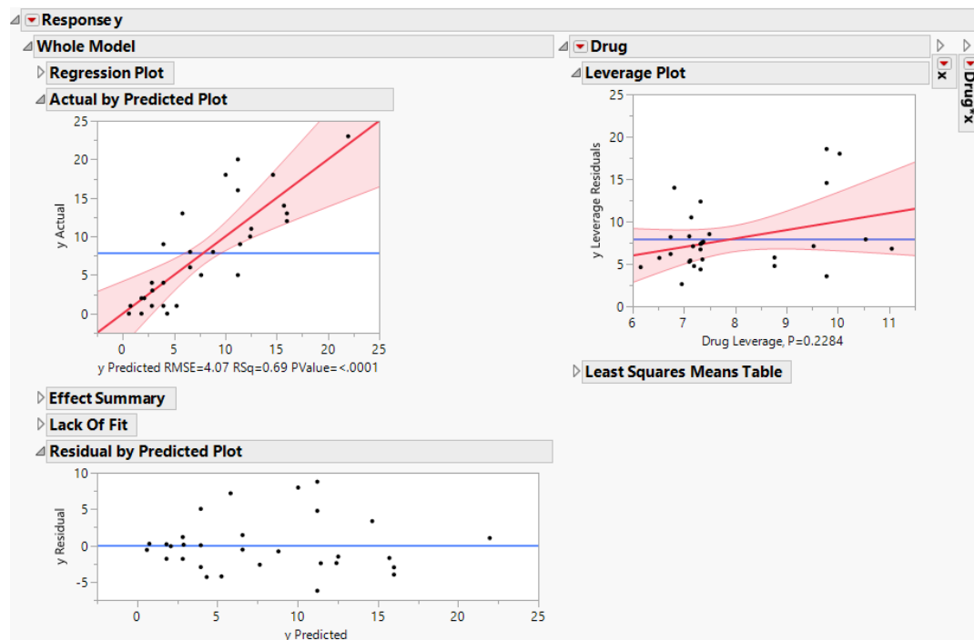
Figure 3.3 Fit Least Squares Report Showing Plots to Assess Model Fit
