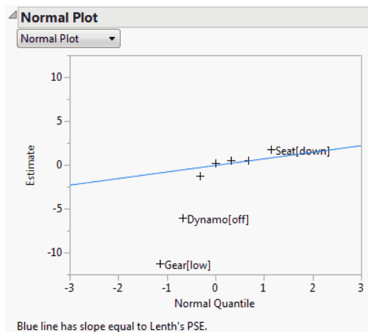
Figure 3.39 Normal Plot
