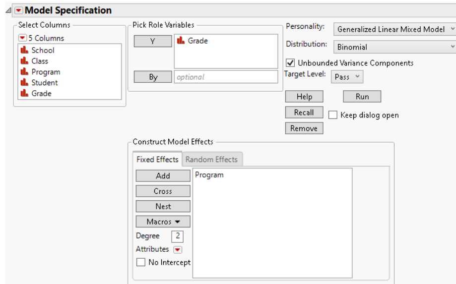
Figure 9.7 Completed Fit Model Launch Window Showing Fixed Effects
