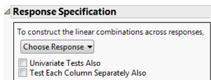
Figure 10.4 Response Specification Panel
