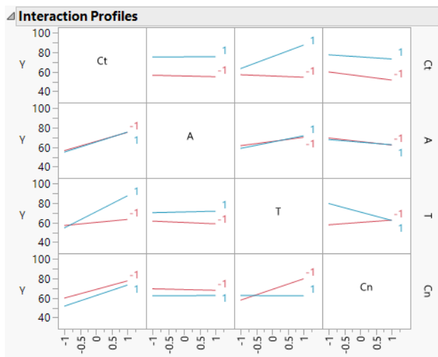
Figure 3.44 Interaction Plots
