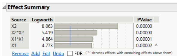
Figure 4.12 Effect Summary Report After Reducing Model
