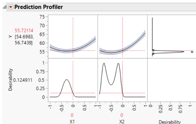
Figure 4.15 Prediction Profiler with Match Target as Goal
