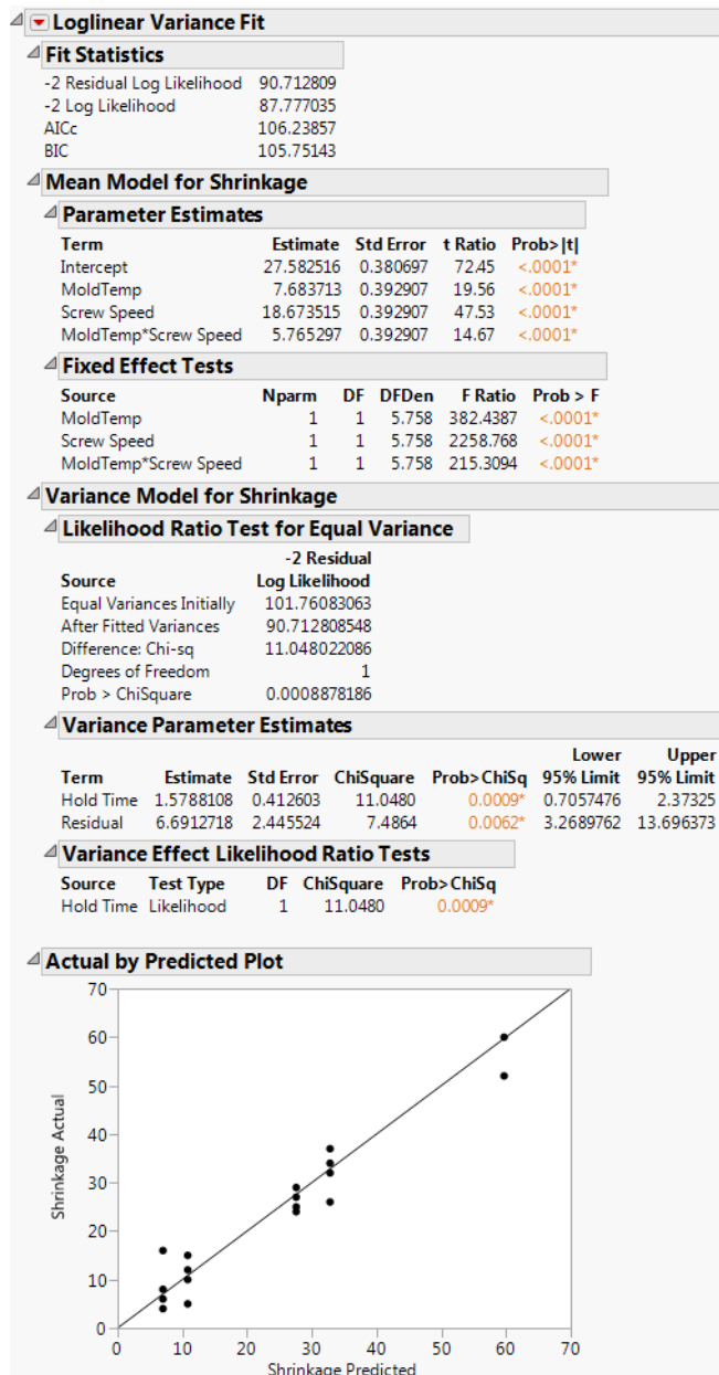
Figure 11.2 Loglinear Variance Report Window
