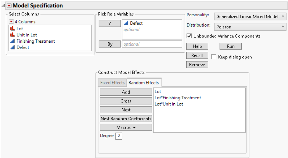
Figure 9.12 Completed Fit Model Launch Window Showing Random Effects Tab
