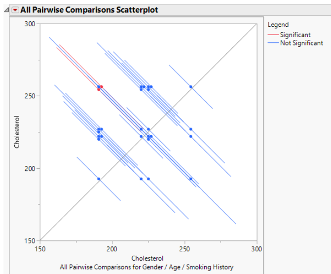
Figure 3.57 All Pairwise Comparisons Scatterplot for User-Defined Comparisons
