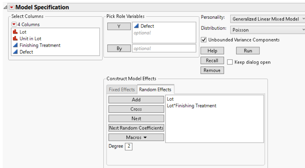
Figure 9.10 Completed Fit Model Launch Window Showing Random Effects Tab
