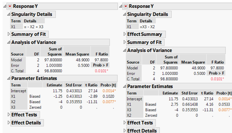
Figure 3.65 Fit Least Squares Reports for Model 1 (on left) and Model 2 (on right)
