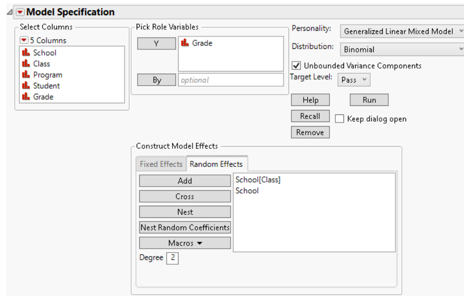
Figure 9.8 Completed Fit Model Launch Window Showing Random Effects
