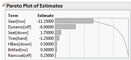
Figure 3.42 Pareto Plot
