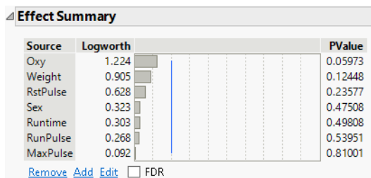
Figure 3.58 Effect Summary Report
