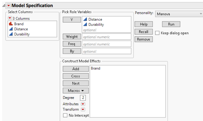
Figure 10.1 Manova Setup
