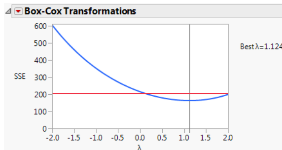
Figure 3.48 Box Cox Y Transformation
