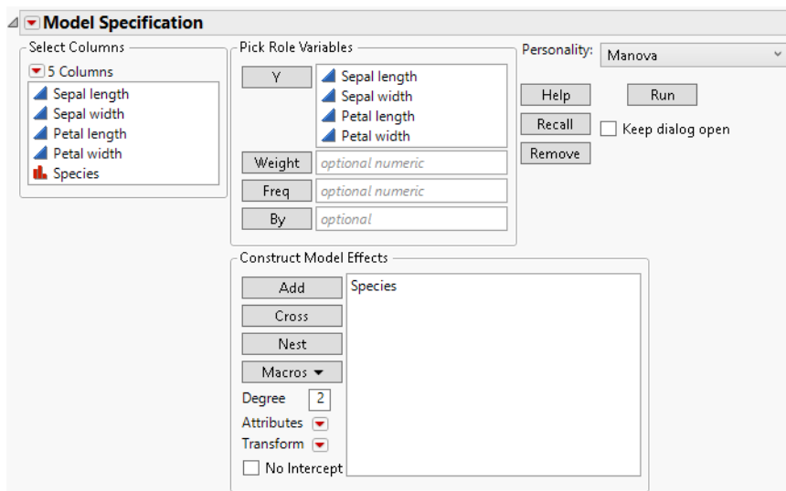
Figure 10.3 Fit Model Launch Window with Manova Selected
