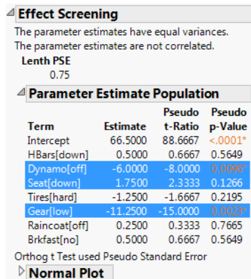
Figure 3.37 Effect Screening Report for Equal Variance and Uncorrelated Estimates
