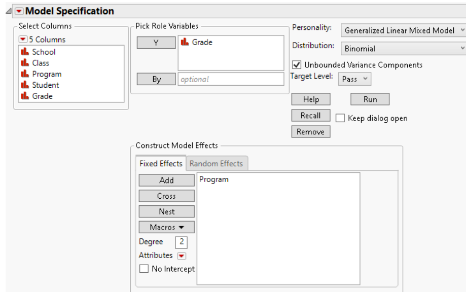
Figure 9.2 Completed Fit Model Launch Window Showing Fixed Effects
