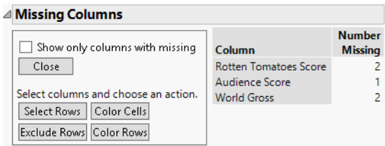
Figure 5.15 Missing Columns Report
