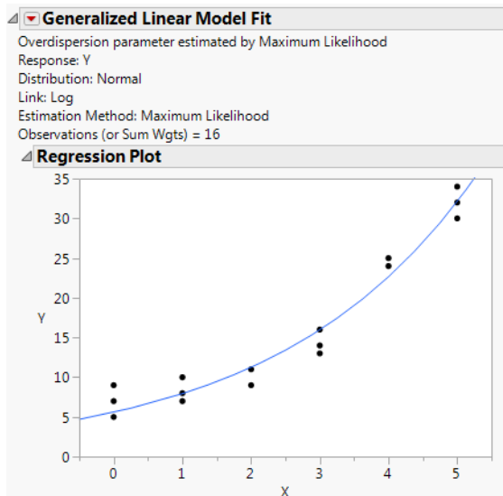
Figure 13.1 Example of a Generalized Linear Model Fit
