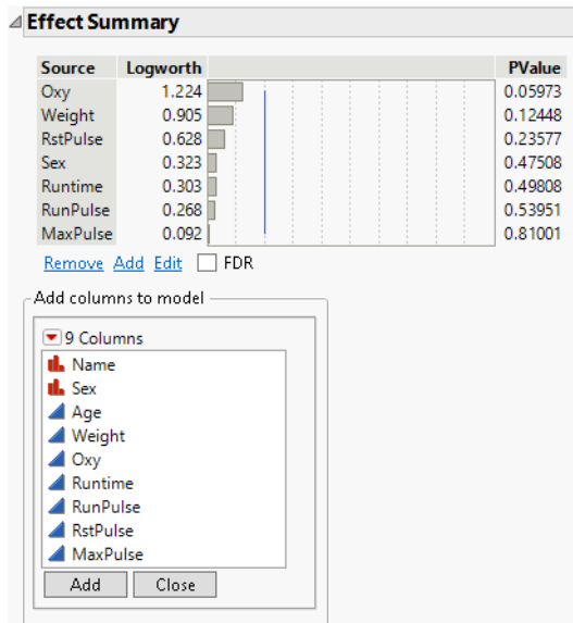
Figure 3.59 Effect Summary Add Columns Panel
