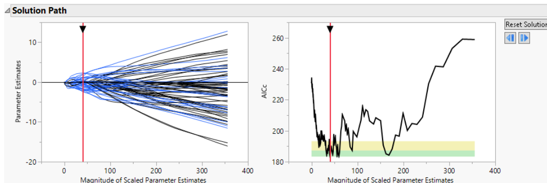
Figure 7.10 Best Fit Model
