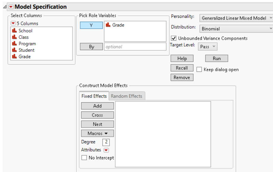
Figure 9.6 Fit Model Launch Window with Generalized Linear Mixed Model Selected
