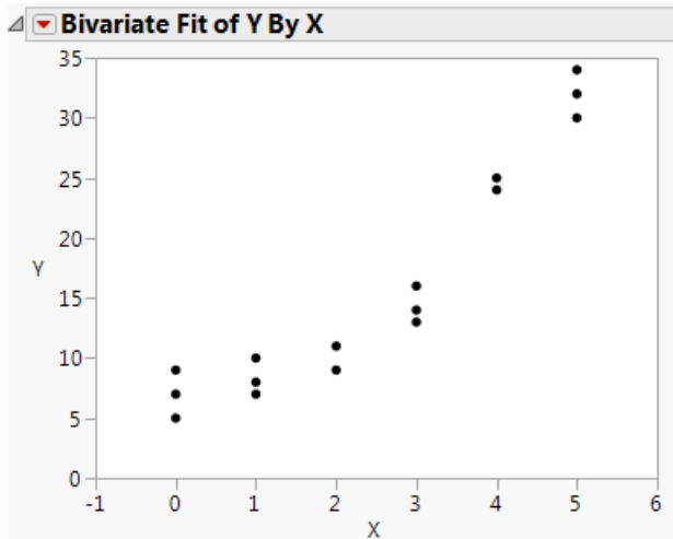
Figure 13.8 Y by X Results
