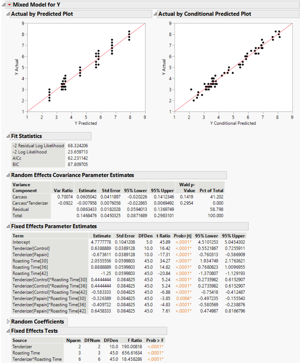
Figure 8.29 Mixed Model Report
