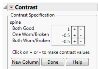
Figure 13.5 Contrast Specification Window
