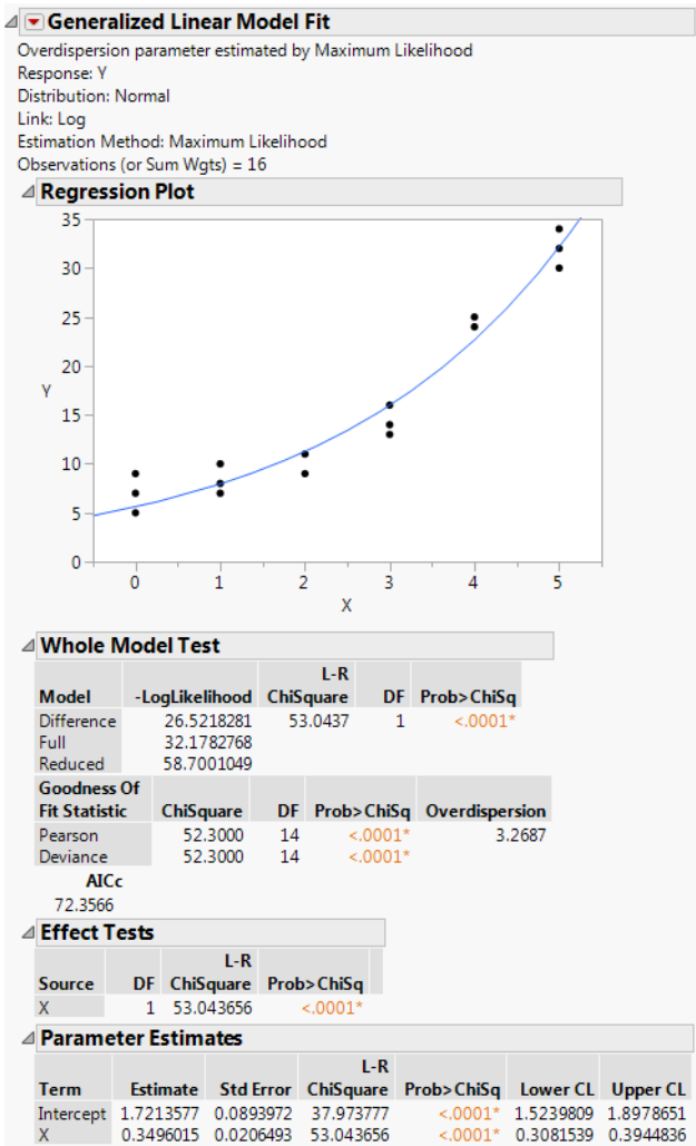
Figure 13.9 Model Results
