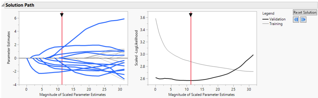
Figure 7.1 Solution Path for Adaptive Lasso Fit with Nonzero Terms Highlighted
