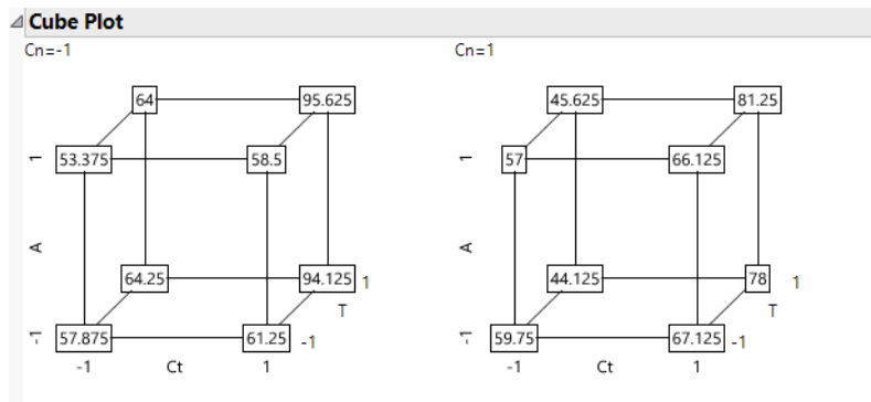
Figure 3.47 Cube Plots
