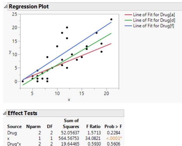
Figure 4.6 Plot with Interaction
