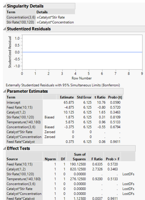
Figure 3.64 Singularity and Parameter Estimates Report for Model with Linear Dependencies
