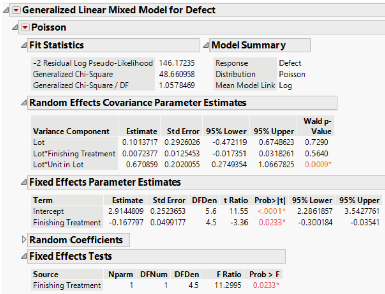
Figure 9.13 Generalized Linear Mixed Model Report Window
