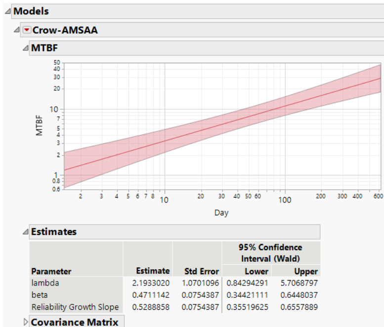
Figure 11.9 MTBF Plot
