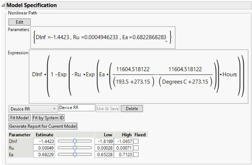
Figure 7.11 Model Specification
