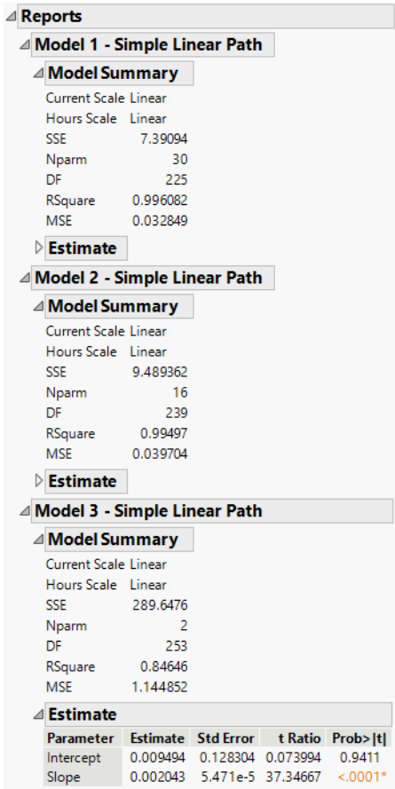
Figure 7.18 Model Reports
