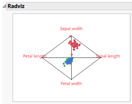
Figure 16.26 Iris.jmp Graph
