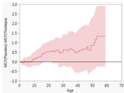
MCF Plot
