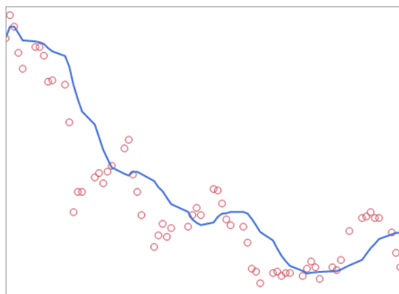
Smoother Graph > Graph Builder
