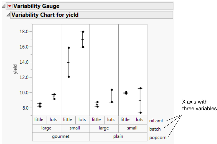
Figure 4.38 Results Window
