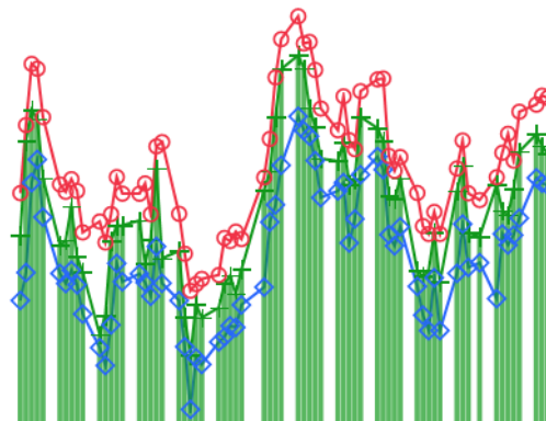
Needle and Line Chart Graph > Graph Builder
