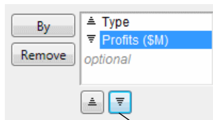
Figure 3.30 Change Profits to Descending
