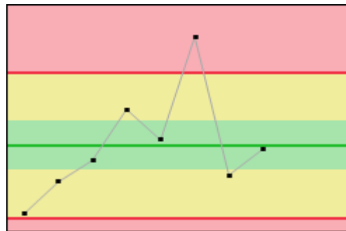
XBar Chart
