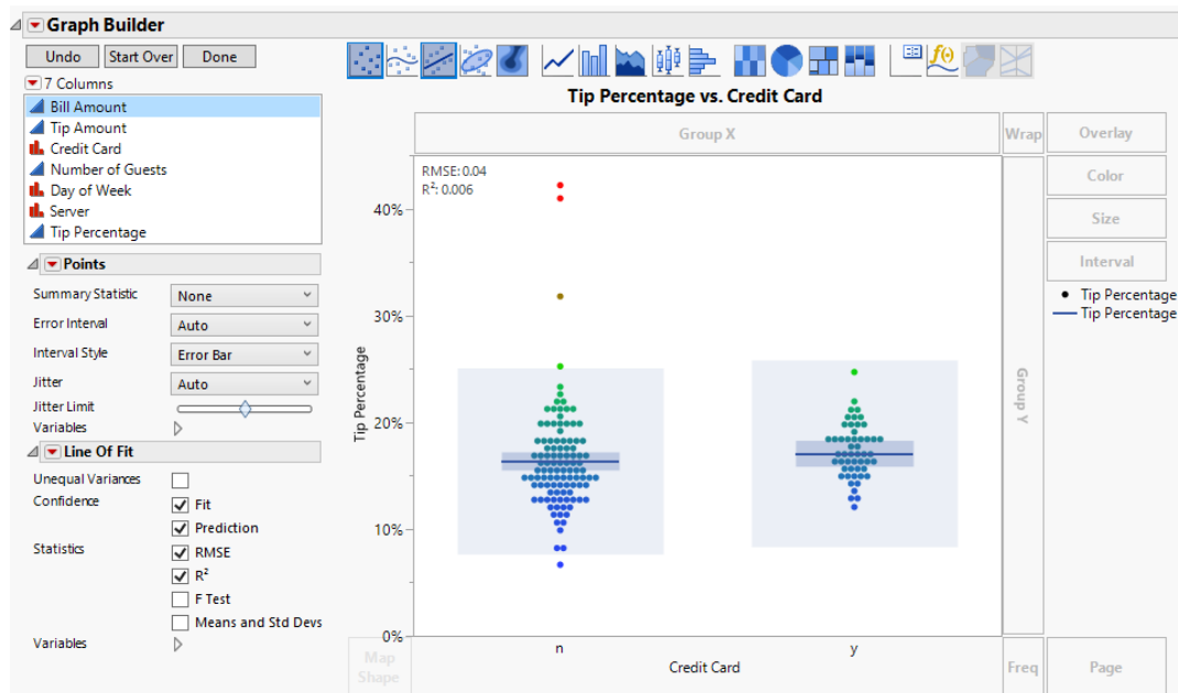
Figure 7.23 Graph Builder Selections For Tip Percentage by Credit Card Type
