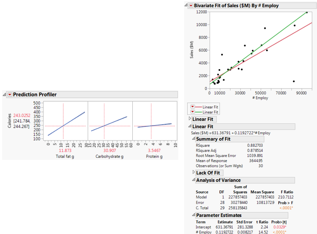
Figure 5.1 Analysis Examples
