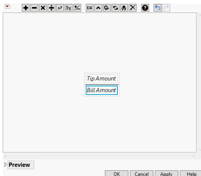
Figure 7.21 Formula for Tip Amount by Bill Amount
