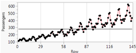
Time Series Analyze > Specialized Modeling > Time Series
