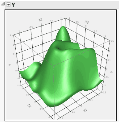
Surface Profiler Analyze > Specialized Modeling > Gaussian Process
