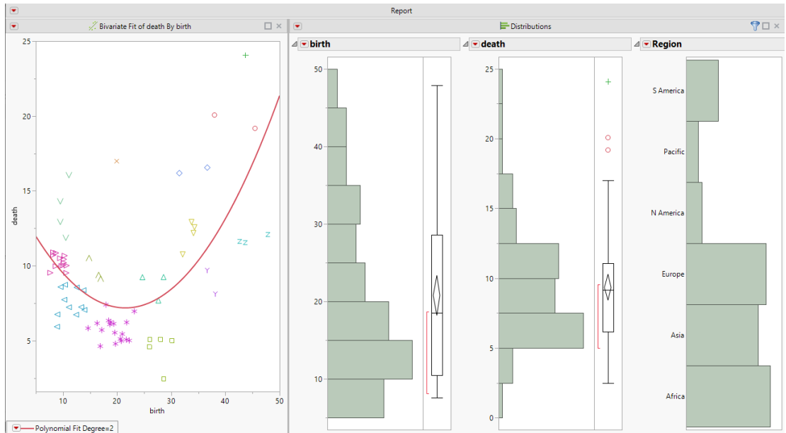
Figure 7.19 Combined Windows
