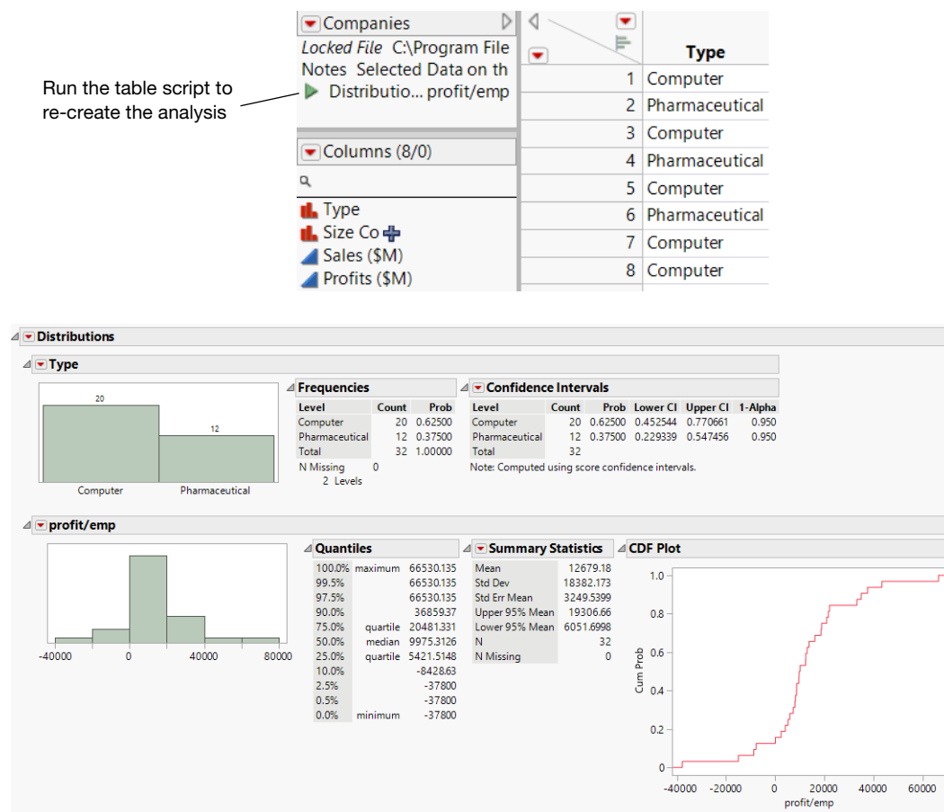
Figure 7.13 Running the Distribution Script
