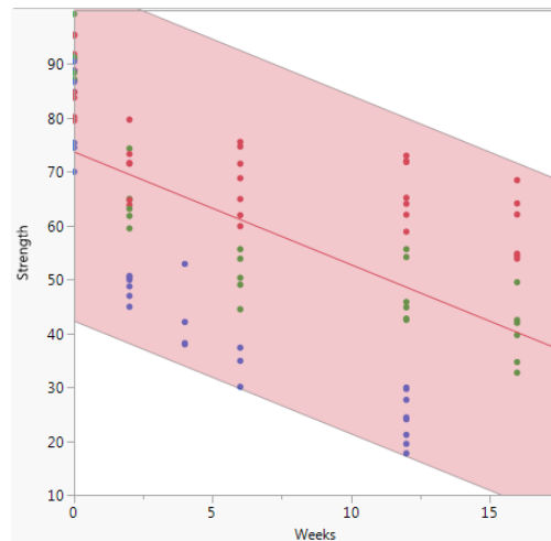
Prediction Interval
