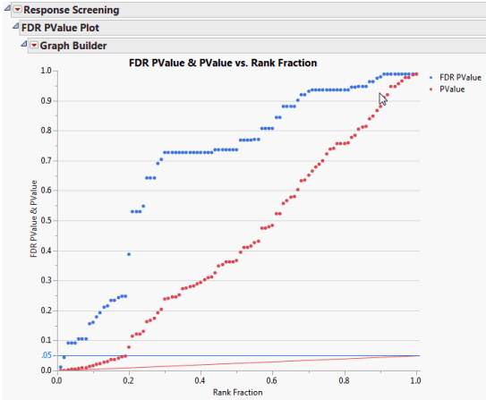
FDR pValue Plot Analyze > Screening > Response Screening
