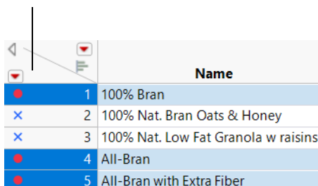
Figure 6.6 Deselecting Rows
