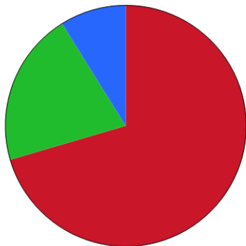
Pie Chart Graph > Graph Builder
