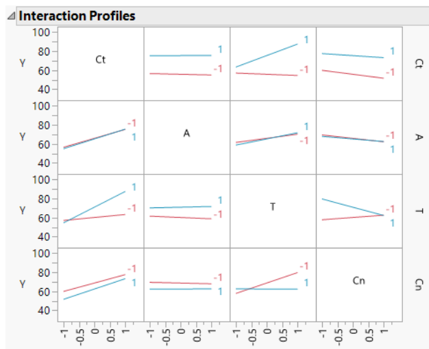
Figure 3.44 Interaction Plots
