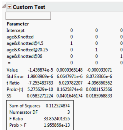
Figure 4.23 Curvature Report
