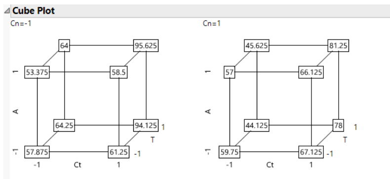
Figure 3.47 Cube Plots
