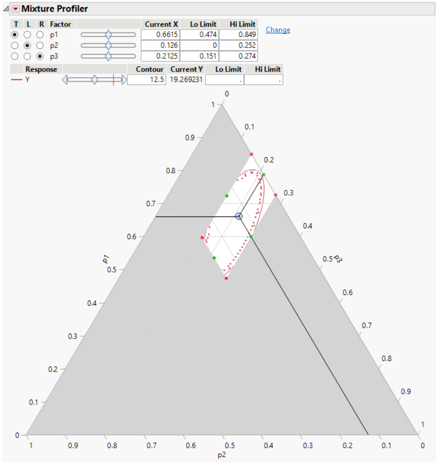
Figure 3.46 Mixture Profiler
