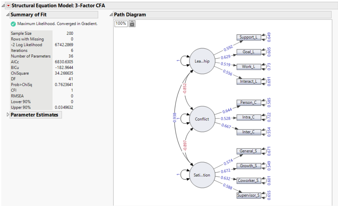
Figure 8.2 Structural Equation Model Report
