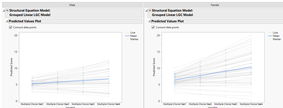
Figure 8.16 Predicted Values Plots
