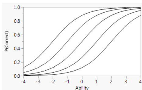
Figure 12.11 Logistic Curve for Several Values of b
