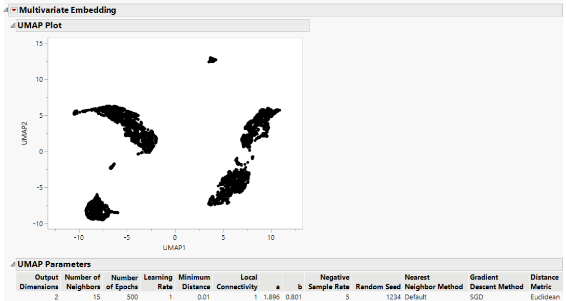
Figure 11.2 Multivariate Embedding Report
