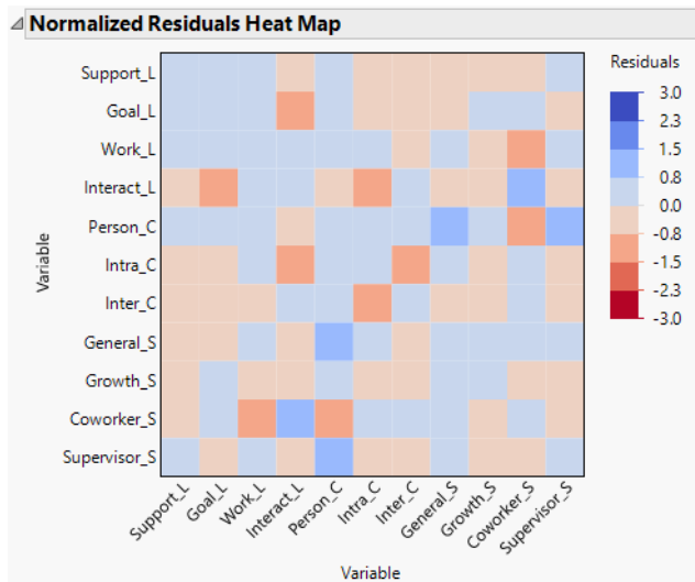
Figure 8.3 Normalized Residuals Heat Map
