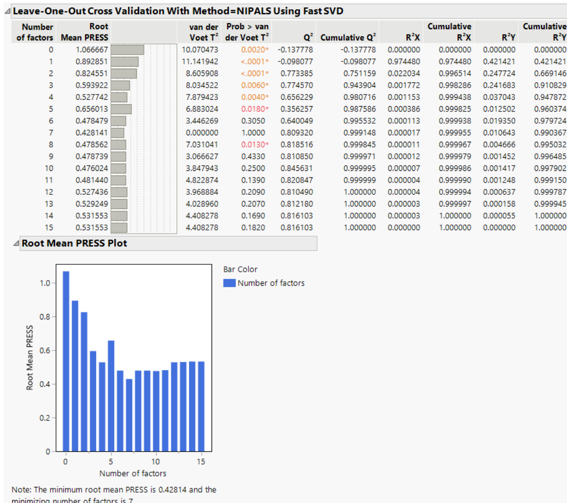
Figure 6.2 Partial Least Squares Report
