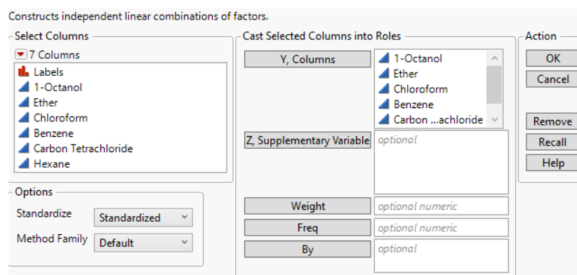
Figure 4.3 Principal Components Launch Window
