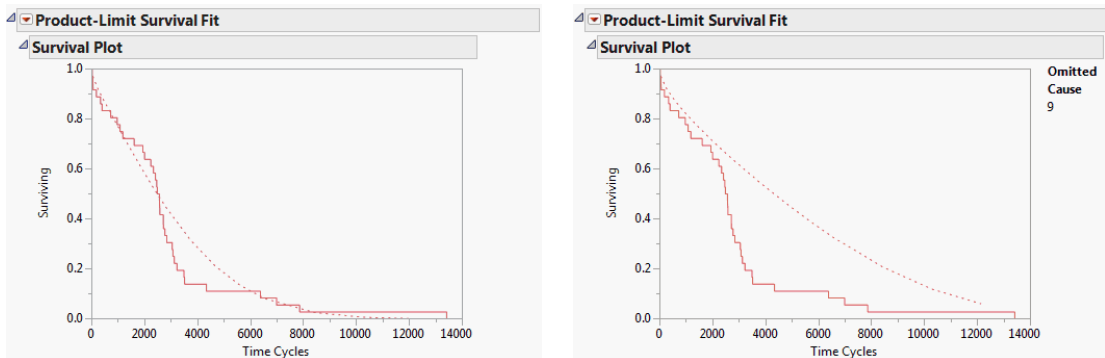
Figure 14.13 Survival Plots with Omitted Causes
