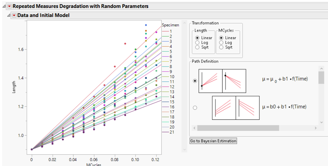
Figure 8.2 Initial Repeated Measures Degradation with Random Parameters Report
