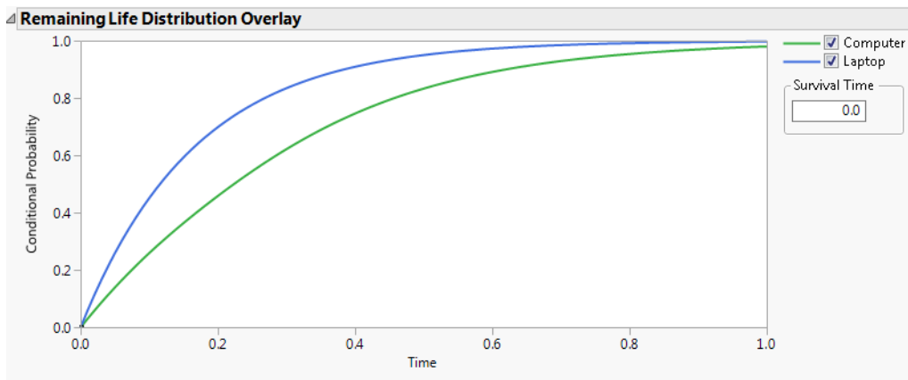
Figure 12.15 Remaining Life Distribution Overlay Example
