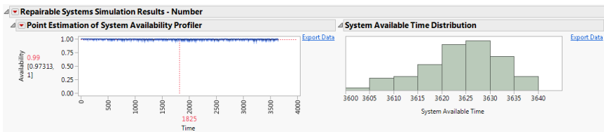
Figure 13.3 Partial RSS Report
