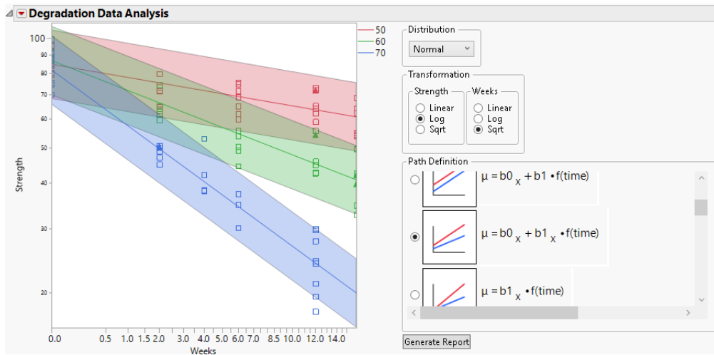
Figure 9.3 Plot Showing Model
