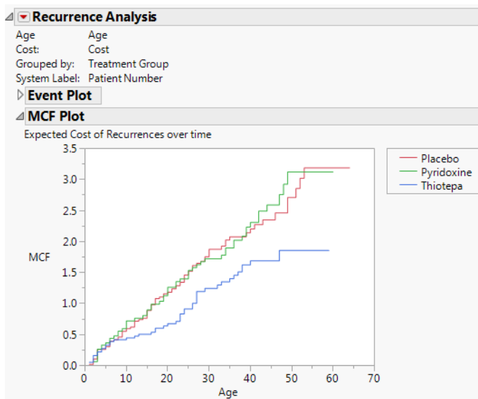
Figure 6.7 Bladder Cancer MCF Plot
