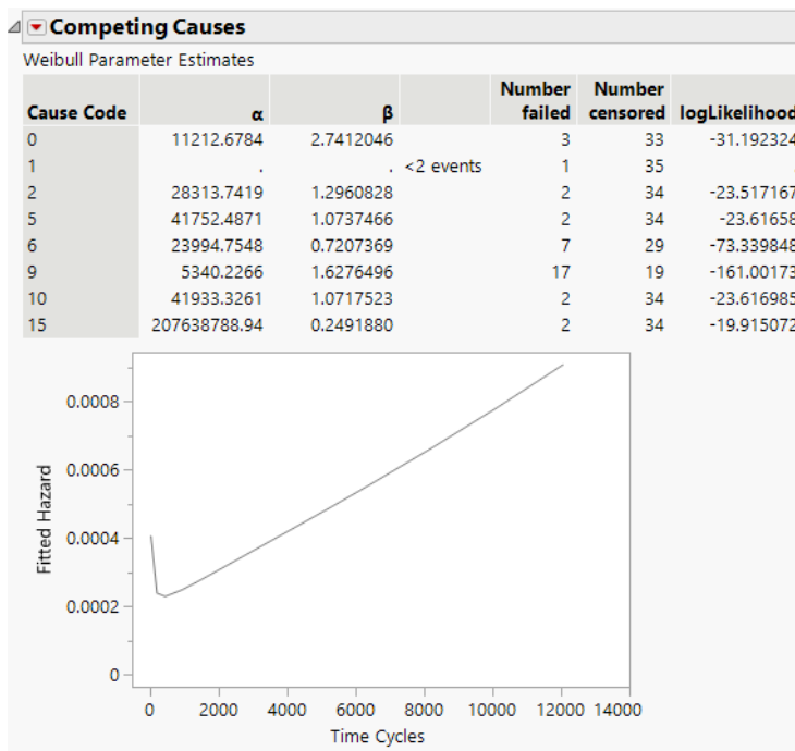
Figure 14.11 Competing Causes Report and Hazard Plot
