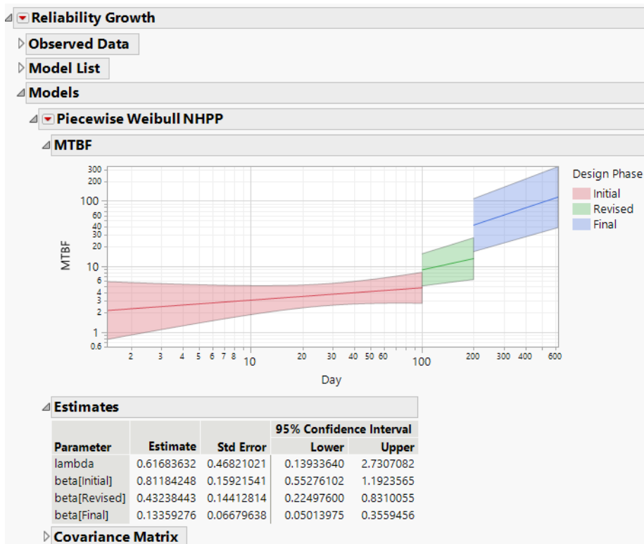
Figure 11.18 Piecewise Weibull NHPP Report
