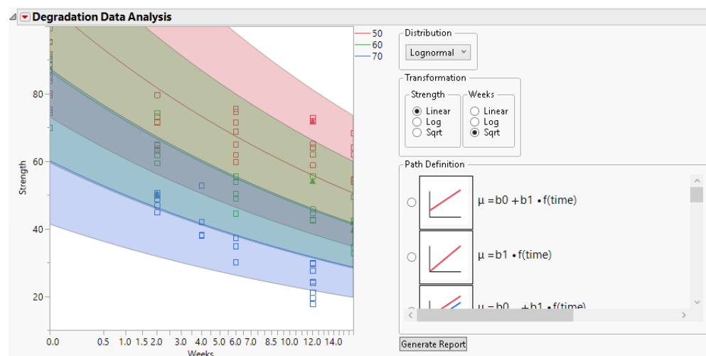
Figure 9.12 Common Slope Model Using a Lognormal Distribution
