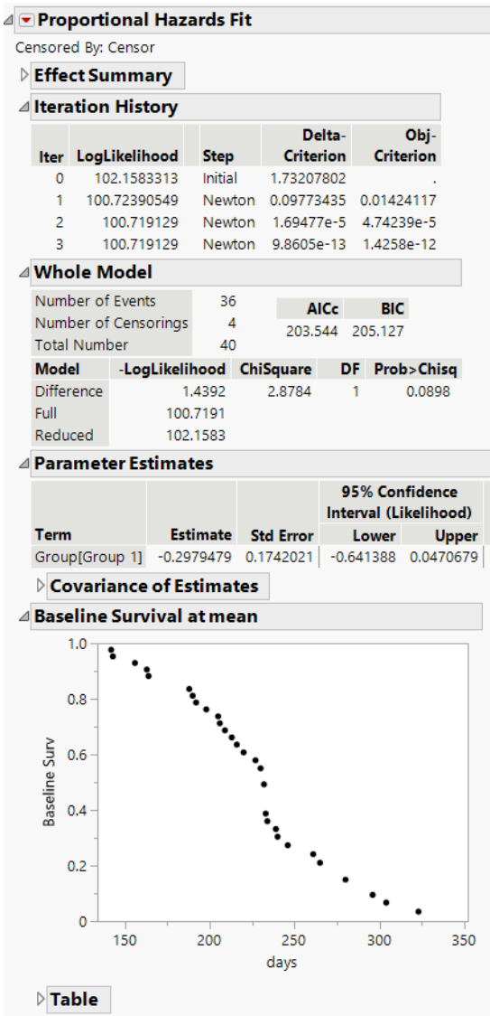
Figure 16.2 Proportional Hazards Fit Report for Rats.jmp Data
