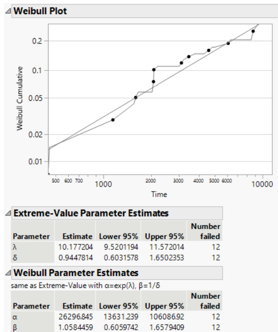
Figure 14.9 Weibull Output for Fan Data
