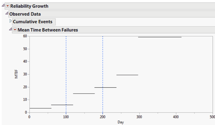
Figure 11.3 Mean Time between Failures Plot
