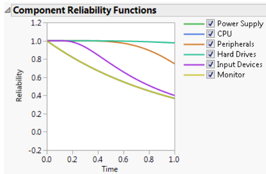
Figure 12.25 Component Reliability Functions
