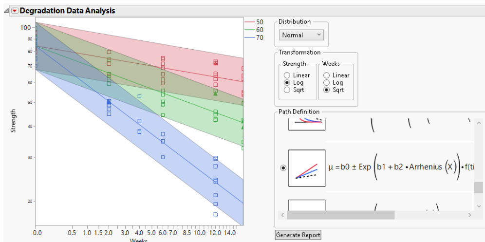
Figure 9.5 Plot Showing Model with Arrhenius Transformation
