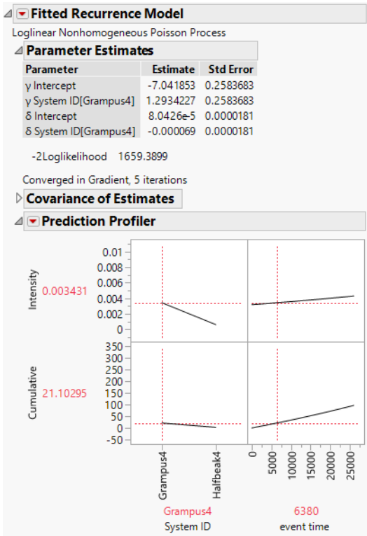
Figure 6.12 Diesel Ship Profiler
