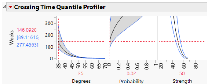
Figure 9.9 Crossing Time Quantile Profiler
