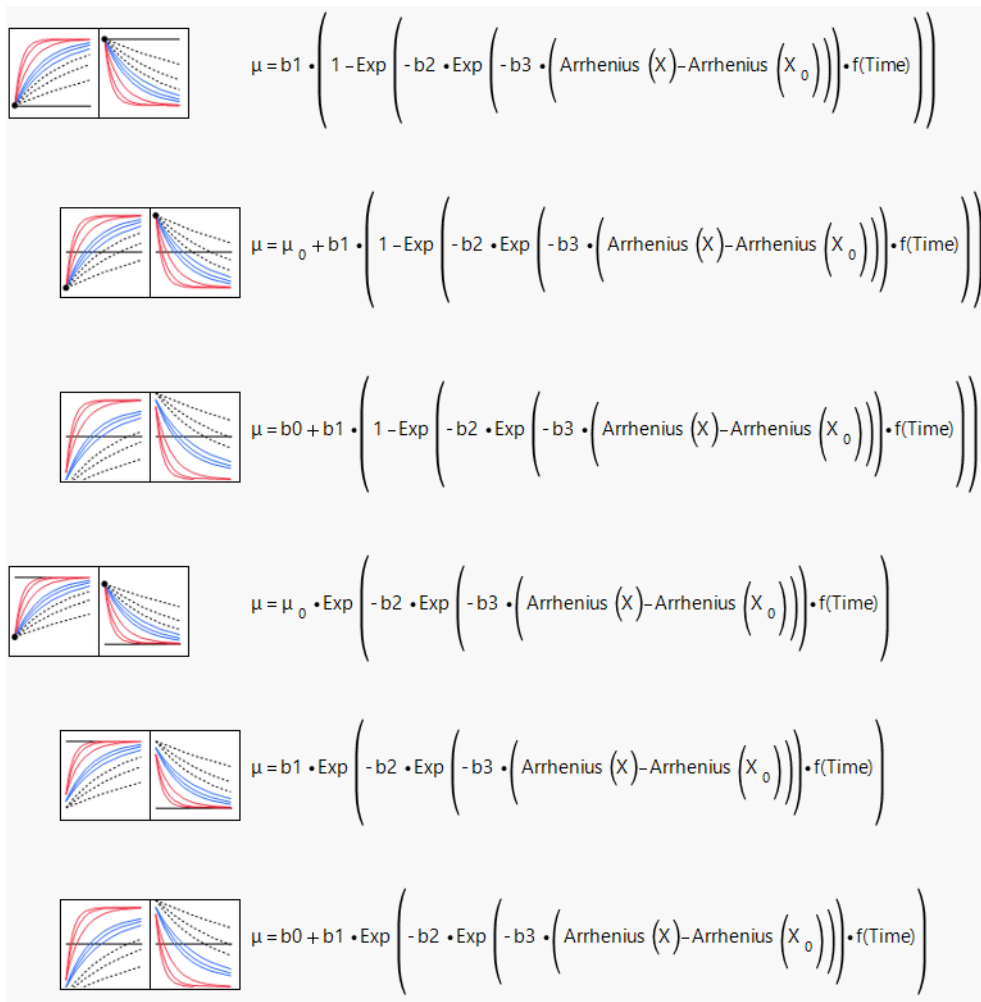
Figure 8.10 First-Order Kinetics Models
