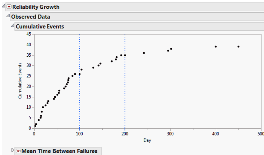
Figure 11.2 Observed Data Report
