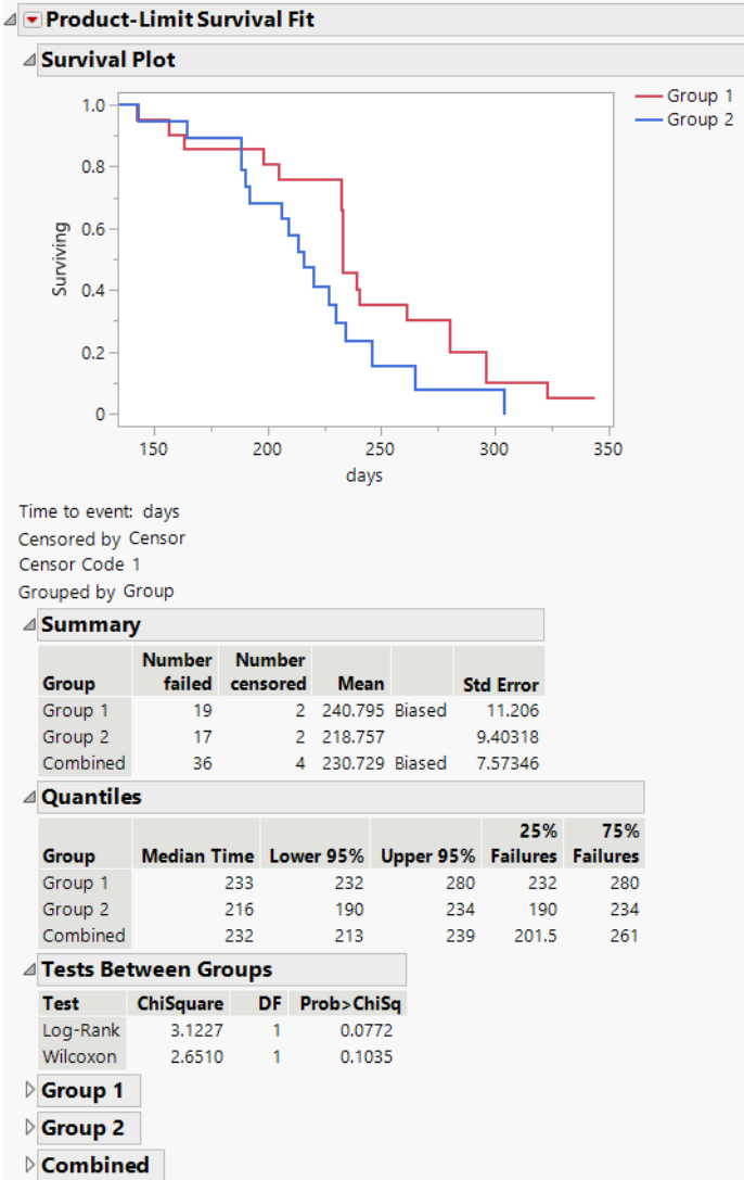
Figure 14.2 Survival Plot for Rats.jmp Data
