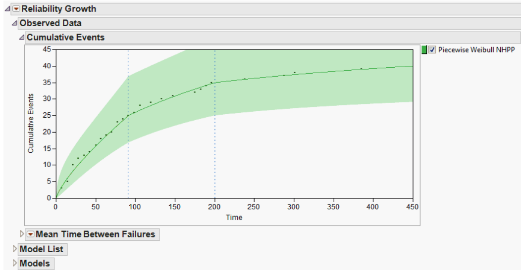
Figure 11.23 Cumulative Events Plot
