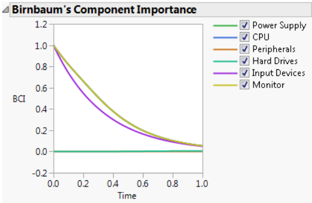
Figure 12.21 Birnbaum's Component Importance
