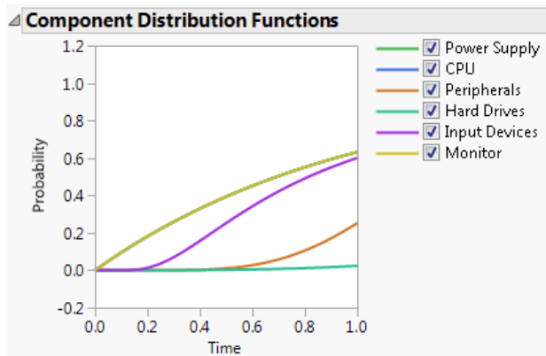
Figure 12.24 Component Distribution Functions
