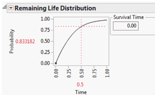
Figure 12.19 Remaining Life Distribution
