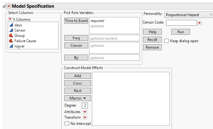
Figure 16.4 The Fit Proportional Hazards Launch Window
