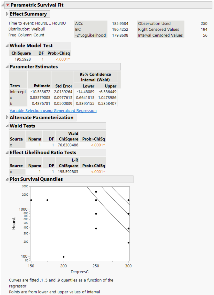
Figure 15.12 ICDevice Output
