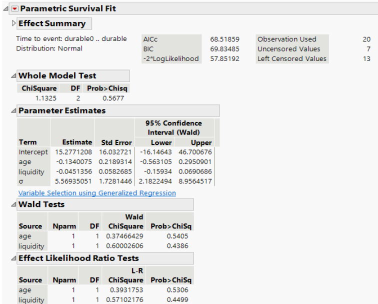
Figure 15.14 Tobit Model Results
