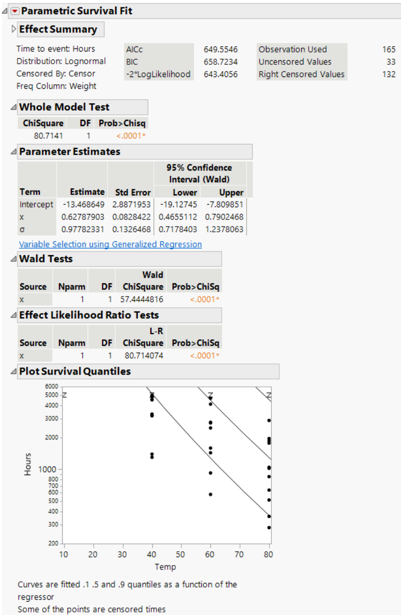
Figure 15.9 Devalt Parametric Output
