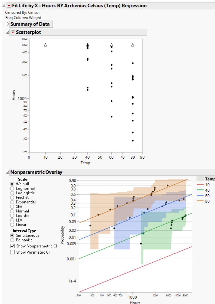
Figure 4.3 Fit Life by X Report Window
