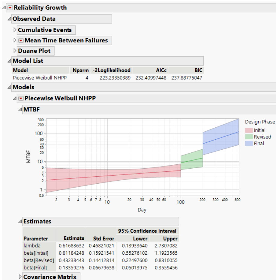
Figure 11.5 Piecewise Weibull NHPP Report
