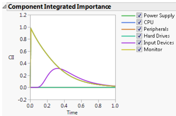
Figure 12.23 Component Integrated Importance
