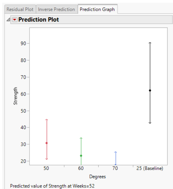
Figure 7.24 Prediction Plot at Weeks = 52
