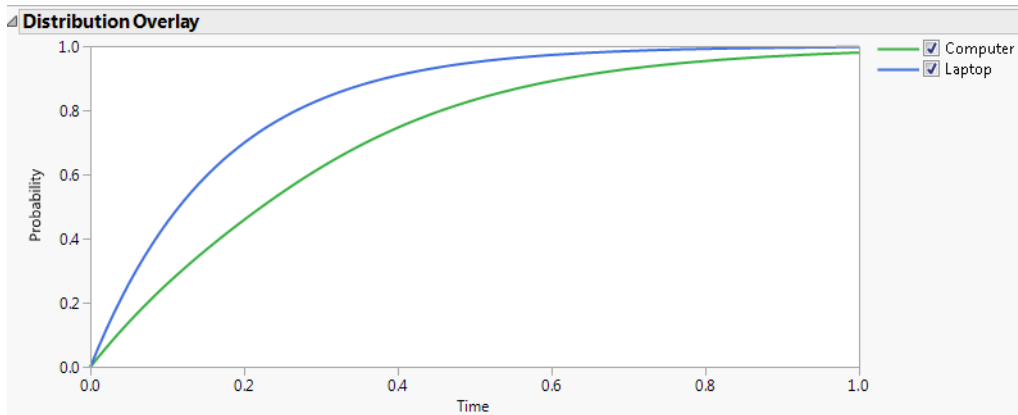
Figure 12.14 Distribution Overlay Example
