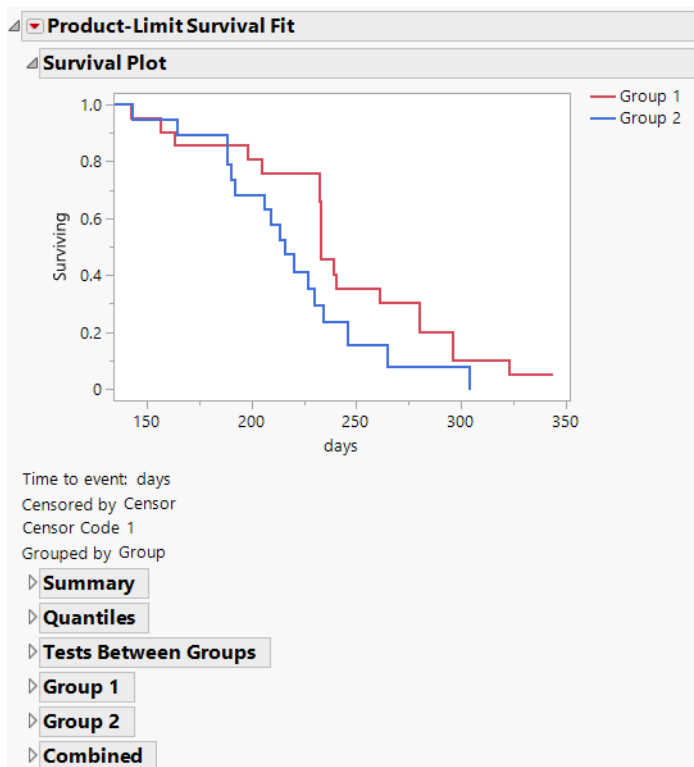
Figure 14.4 The Survival Plot
