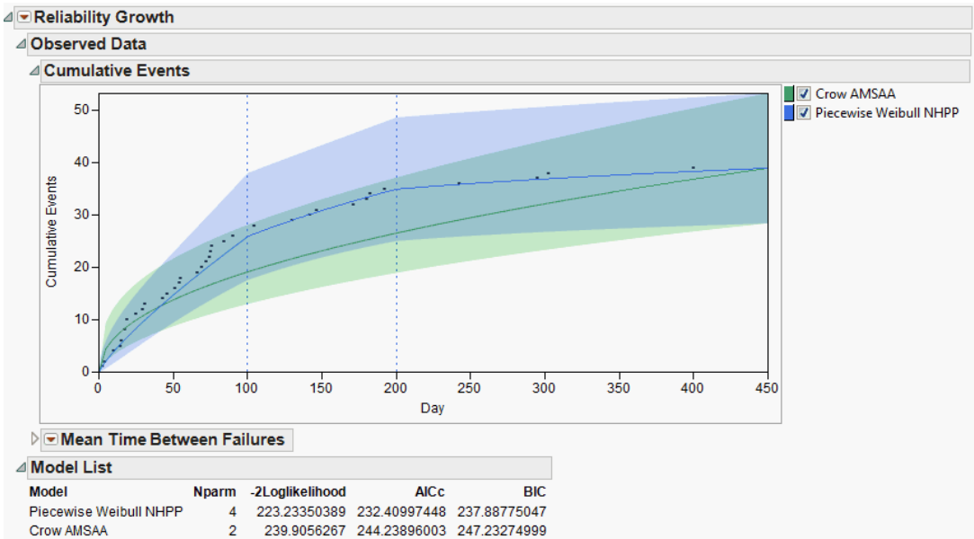
Figure 11.17 Cumulative Events Plot and Model List Report
