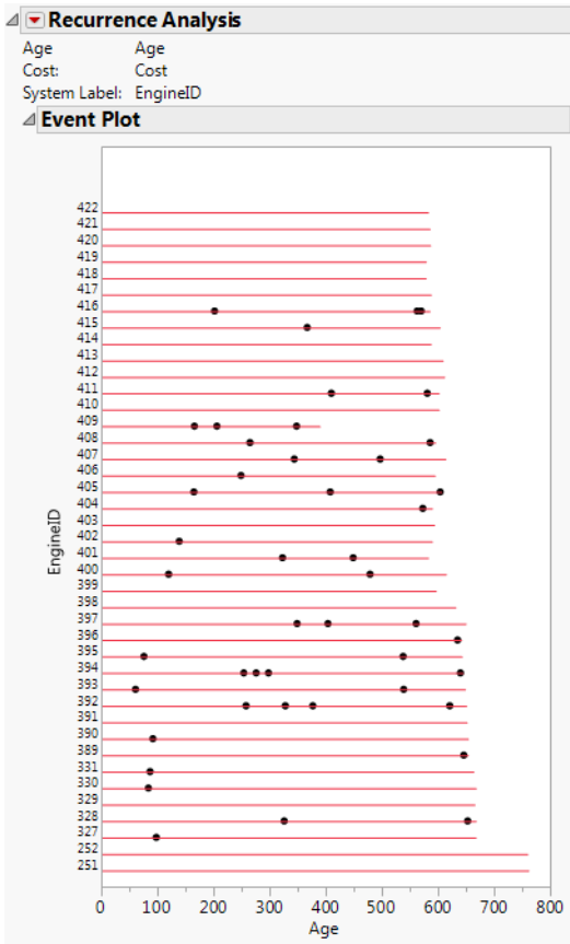
Figure 6.2 Event Plot for Valve Seat Replacements
