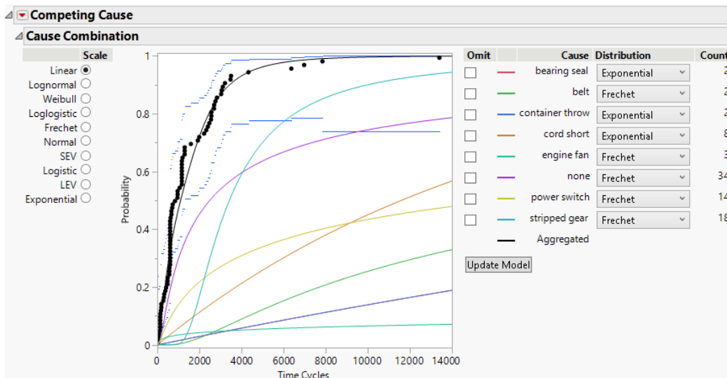
Figure 3.11 Initial Competing Cause Report
