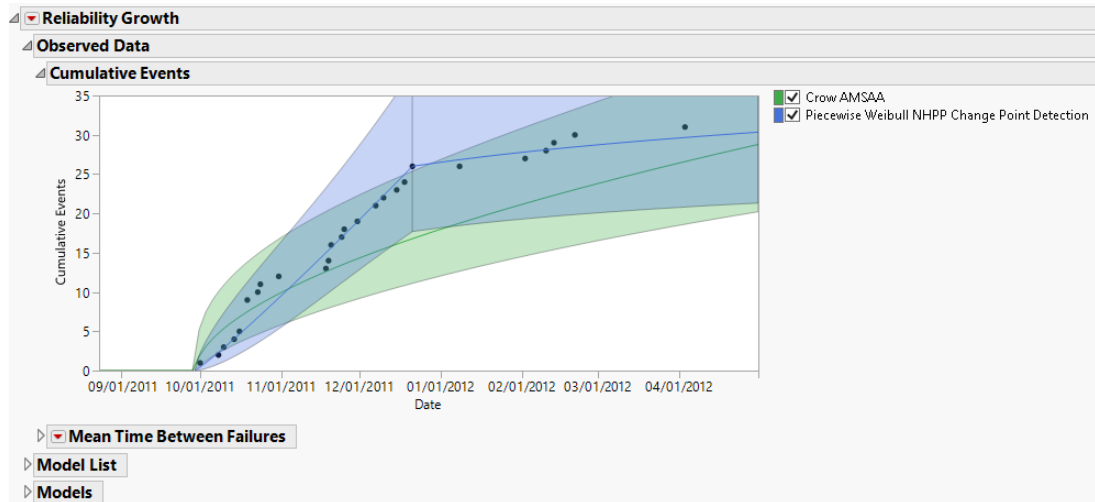
Figure 11.26 Cumulative Events Plot with Two Models
