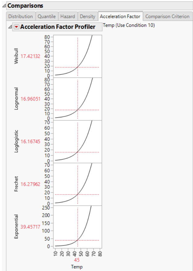
Figure 4.10 Acceleration Factor Profiler
