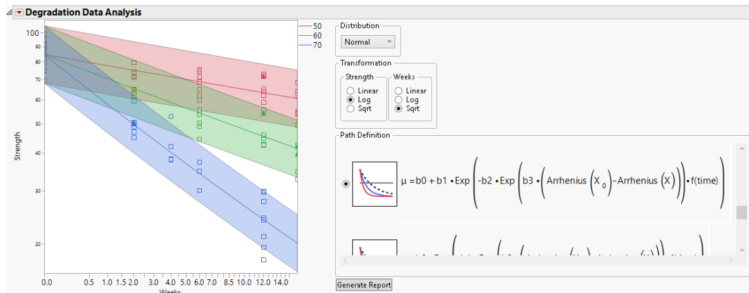
Figure 9.13 Example of First-Order Kinetics Model Type 3
