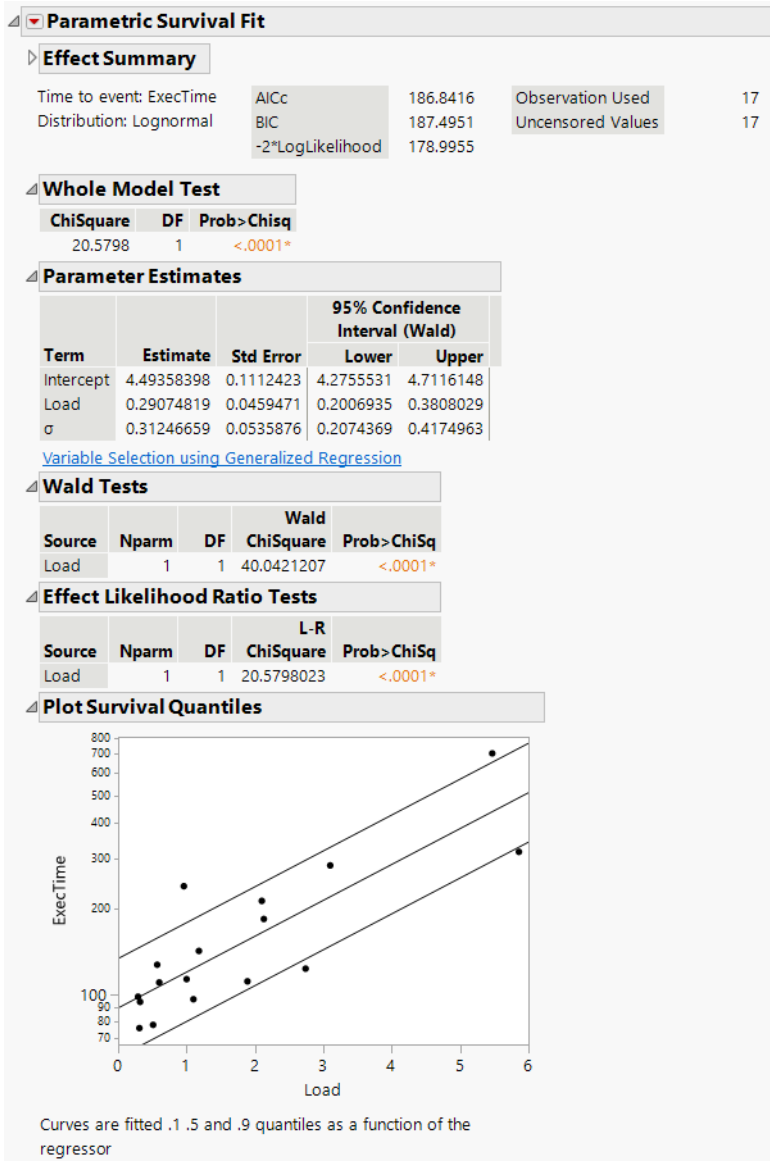
Figure 15.5 The Parametric Survival Fit Report
