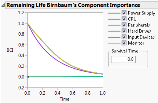
Figure 12.22 Birnbaum's Component Importance for Remaining Life
