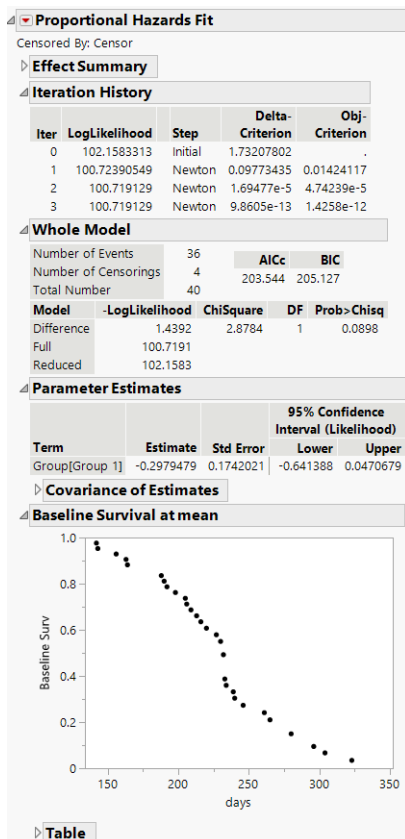
Figure 16.1 Example of a Proportional Hazards Fit
