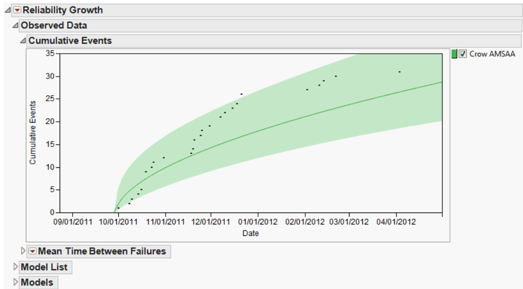
Figure 11.25 Cumulative Events Plot with Crow AMSAA Model
