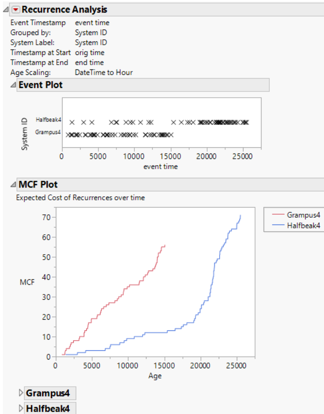
Figure 6.10 Diesel Ship Engines Report
