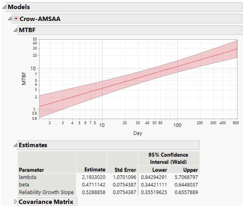
Figure 11.9 MTBF Plot
