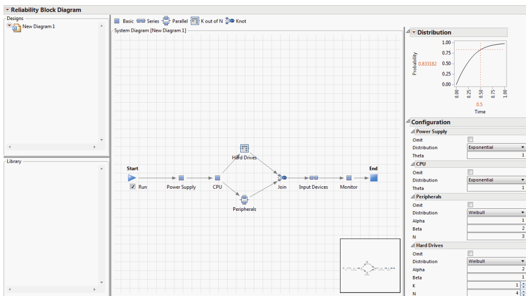
Figure 12.1 Example of a Reliability Block Diagram
