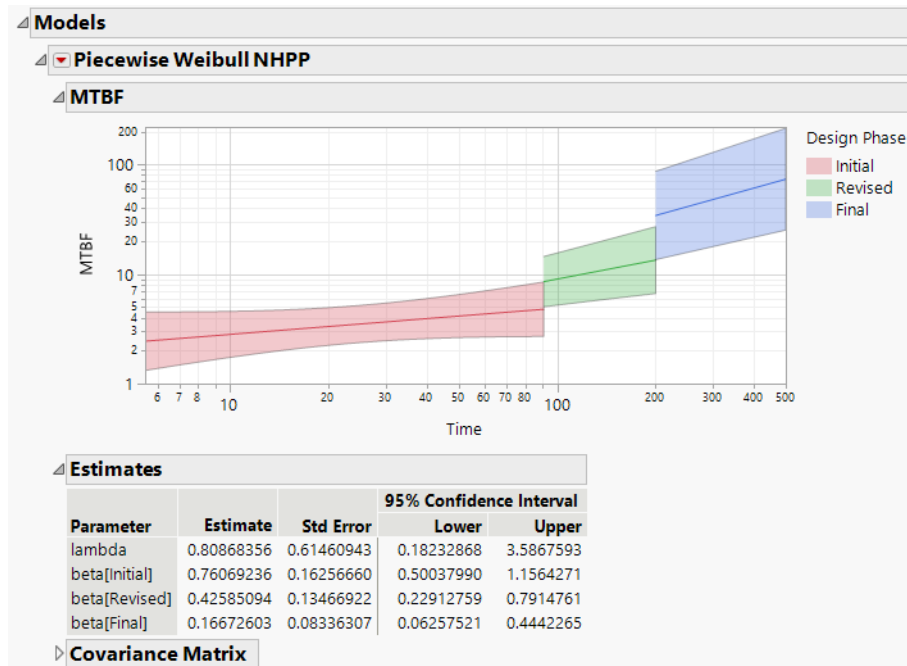
Figure 11.24 MTBF Plot
