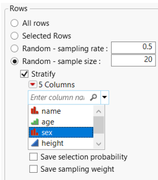
Figure 6.3 Stratified Subsets
