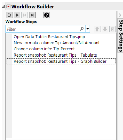
Figure 12.1 Workflow Builder
