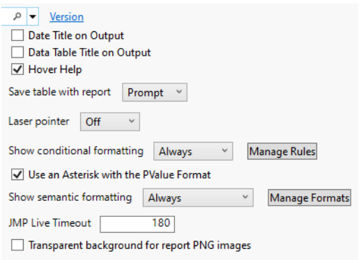
Figure 14.2 Reports Preferences
