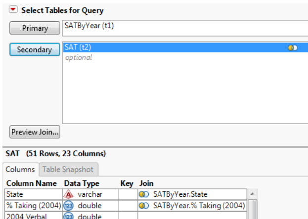
Figure 6.30 Joined Columns
