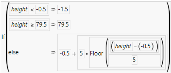
Figure 4.40 Formula
