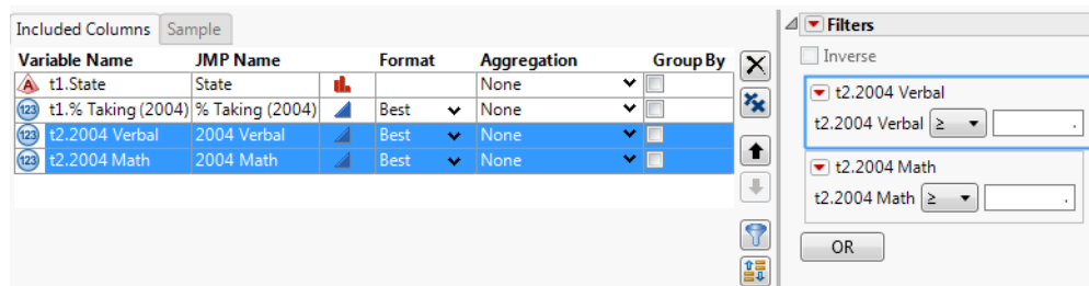
Figure 6.31 Selected Filters
