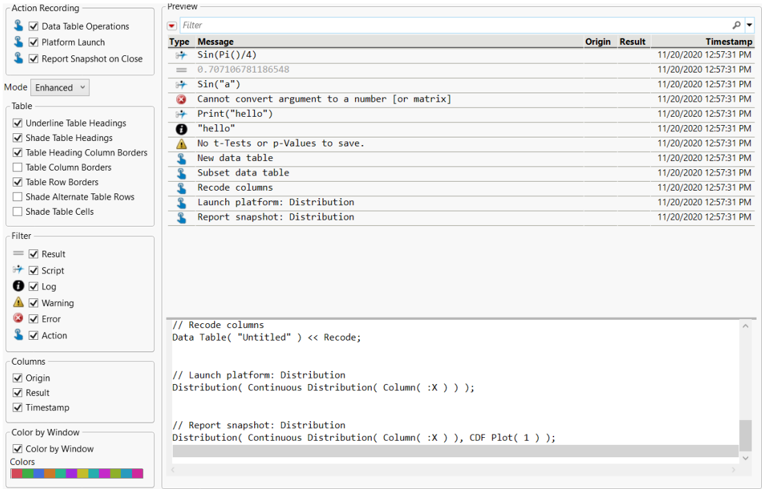
Figure 14.21 Log Preferences
