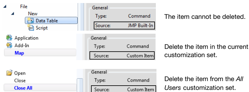
Figure 13.4 Examples of Customization Sources
