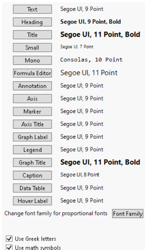
Figure 14.5 Fonts Preferences
