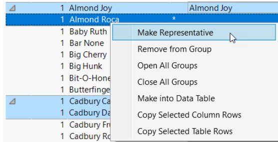
Figure 4.45 Make Representative
