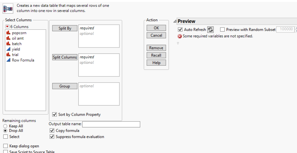
Figure 6.10 Split Window
