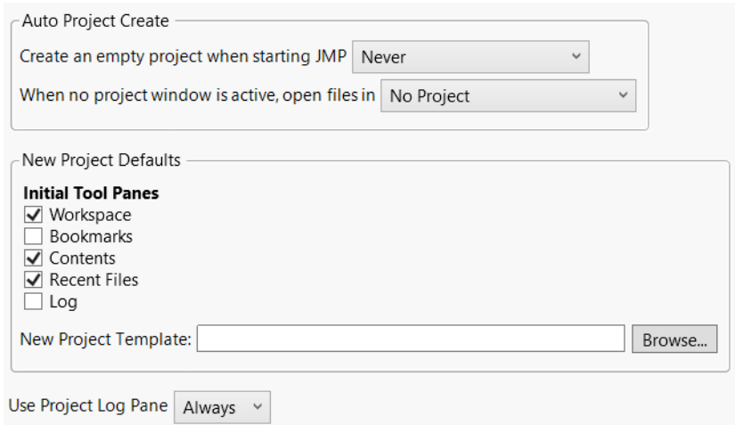
Figure 14.7 Projects Preferences
