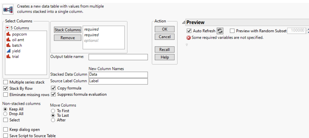
Figure 6.7 Stack Window
