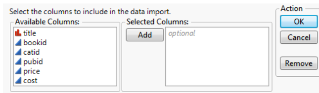
Figure 3.60 Select Columns
