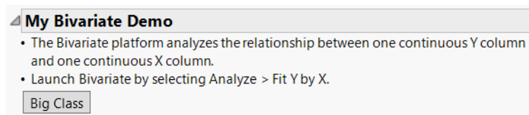
Figure 10.36 Final Journal
