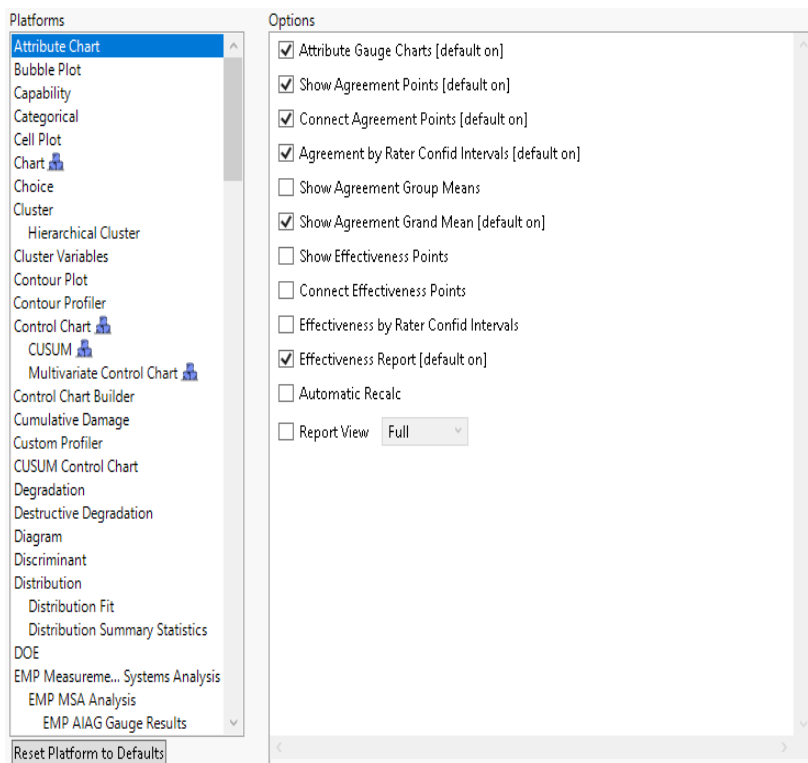
Figure 14.13 Platforms Preferences
