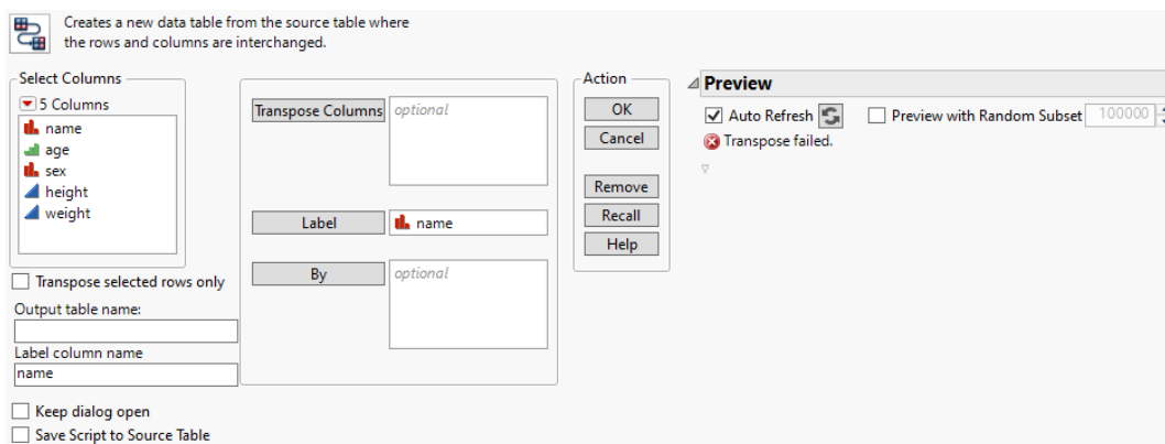
Figure 6.13 Transpose Window
