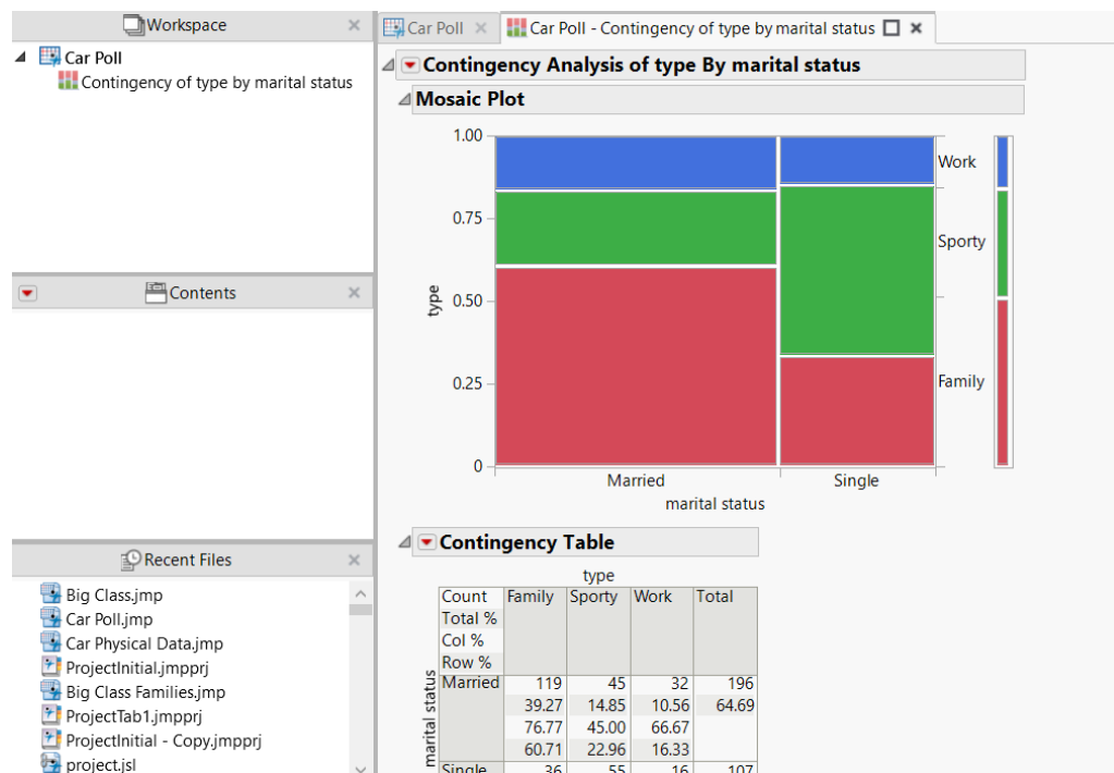
Figure 10.22 Initial Project
