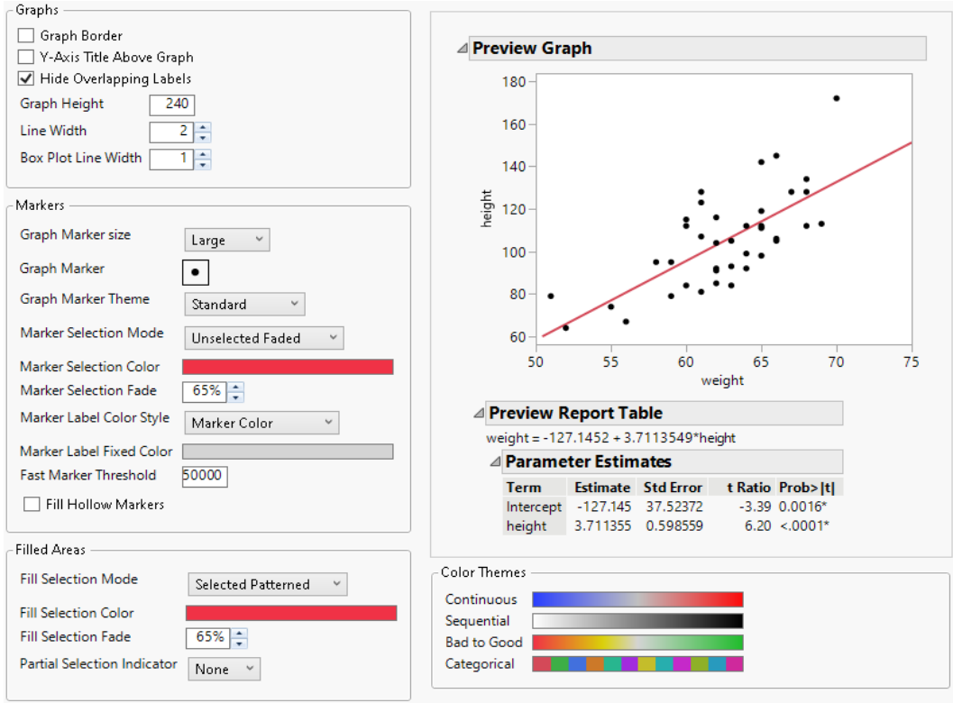
Figure 14.3 Graphs Preferences
