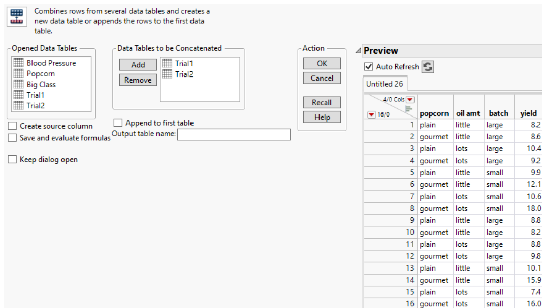
Figure 6.17 Concatenate Window
