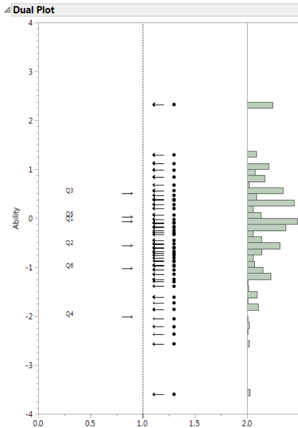
Figure 12.7 Dual Plot
