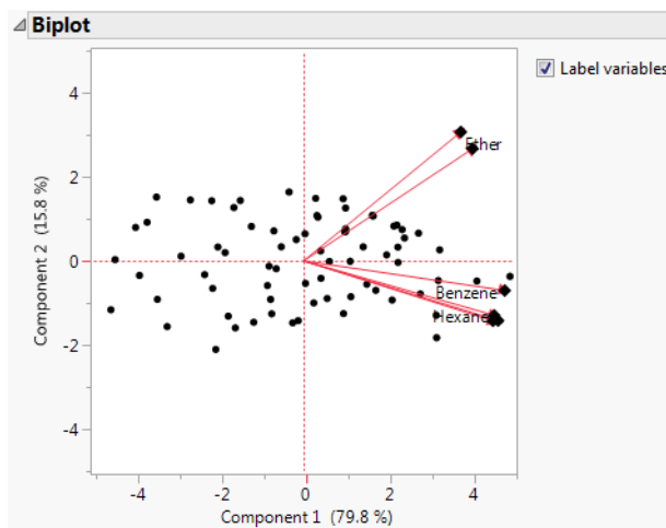
Figure 4.8 Biplot
