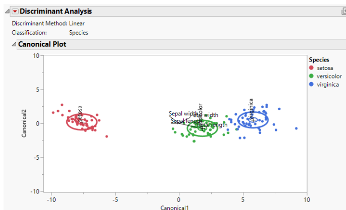
Figure 5.1 Canonical Plot
