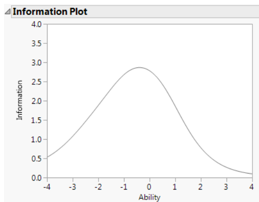
Figure 12.6 Information Plot
