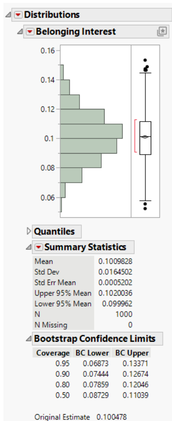
Figure 8.28 Bootstrap Report
