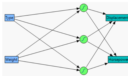
Diagrama neuronal
