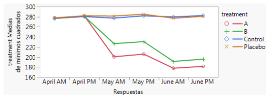
MANOVA
