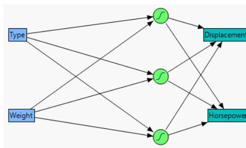
Diagrama neuronal
