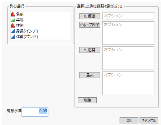
図11.35 Column Dialog
