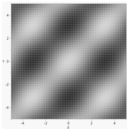
図12.38 Gradient Function
